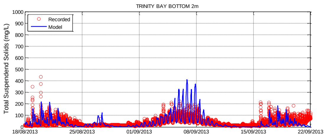
Figure 5-24 Sediment Re-suspension Validation – Trinity Bay
