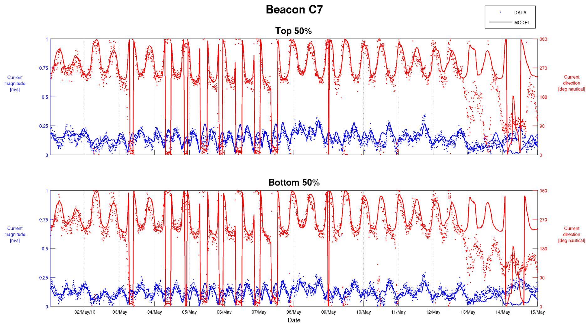
Figure C-19 Top 50% and Bottom 50% Current Calibration – Beacon C7 01/05/2013 to 15/05/2013
