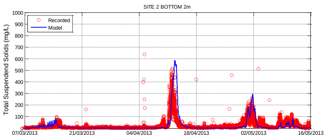
Figure 3-39 Sediment Re-suspension Calibration – Site 2
