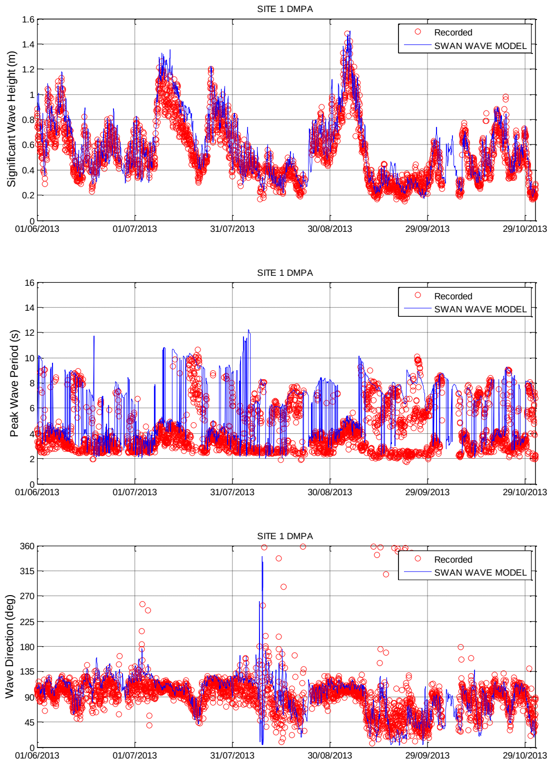
Figure 5-22 SWAN Wave Model Validation – Site 1 DMPA
