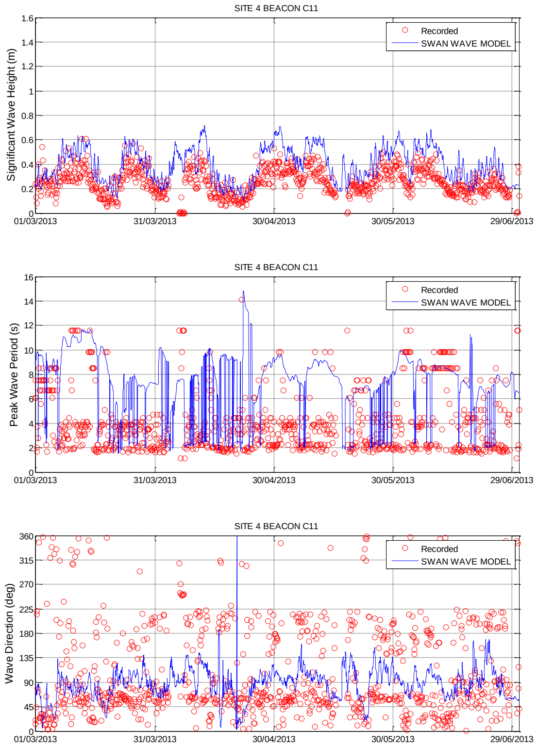
Figure 3-34 SWAN Wave Model Calibration – Site 4 Beacon C11
