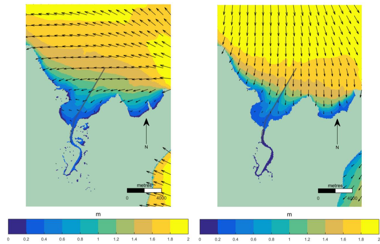
Figure 7-19 100m Grid Modelled Wave Fields South Easterly Wave Case, 9/4/2013 (top left) Northerly Wave Case, 24/1/2013 (top right)
