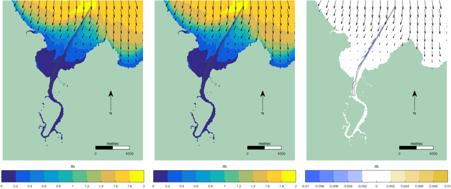
Figure 7-21 25m Grid Northerly Wave Case: Base Case ( left ); Developed Case ( middle ); Difference ( right ). Vectors indicate Direction; Contours indicate Magnitude
