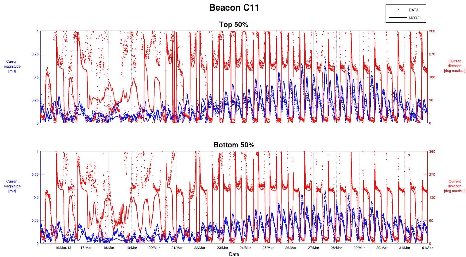
Figure C-23 Top 50% and Bottom 50% Current Calibration – Beacon C11 15/03/2013 to 01/04/2013
