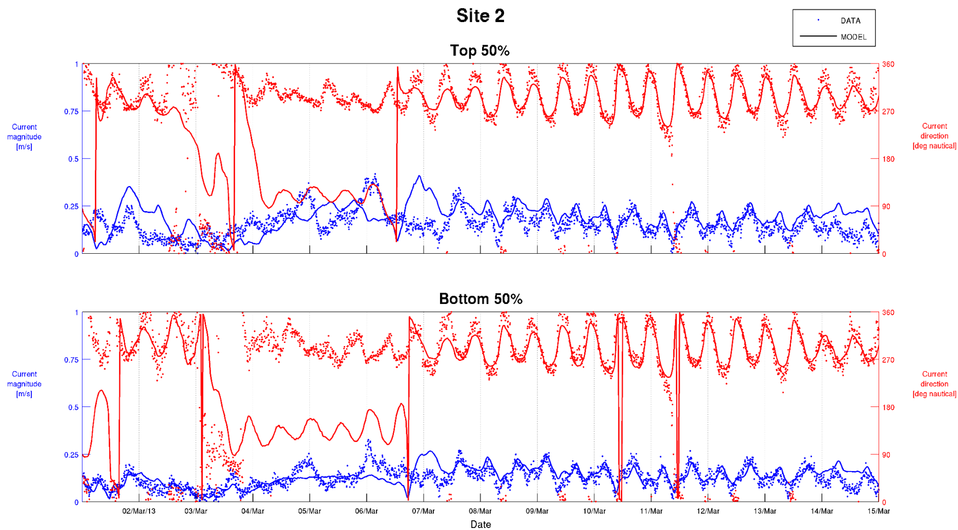
Figure C-8 Top 50% and Bottom 50% Current Validation – Site 2 01/03/2013 to 15/03/2013
