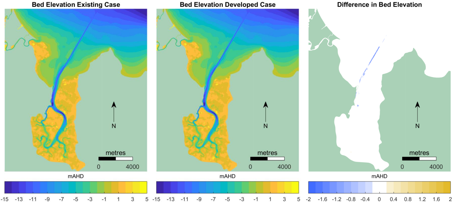
Figure 7-1 Cairns Shipping Channel and Surrounds Bed Elevation: Existing case (left); Developed case (middle) and Difference (right)
