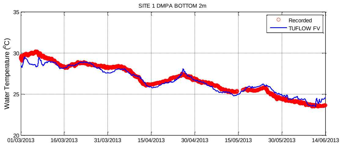
Figure 3-25 Hydrodynamic Model Calibration Near Bed Temperature – Site 1 DMPA
