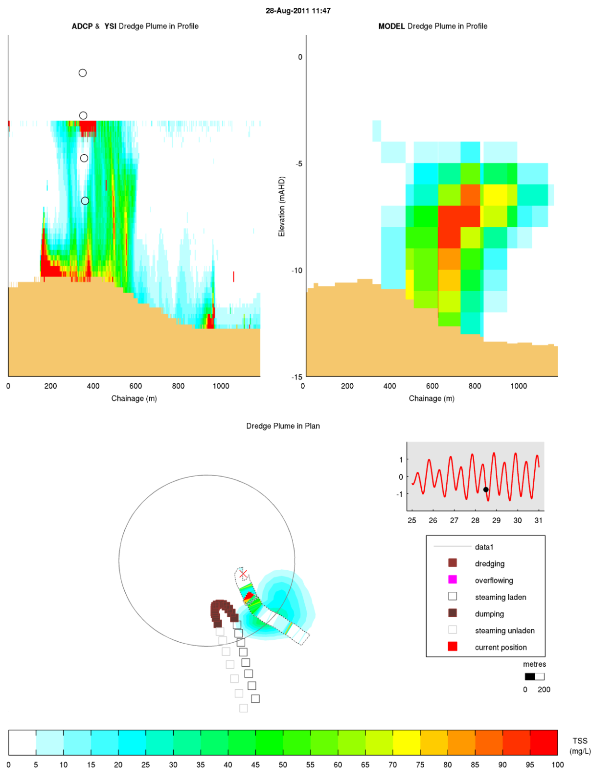
Figure 4-8 DMPA Plume Validation, 28/08/2011 11:47: Recorded Plume (top left) and Modelled Plume (top right) Vertical Distribution; Recorded and Modelled Plume Plan View (bottom)
