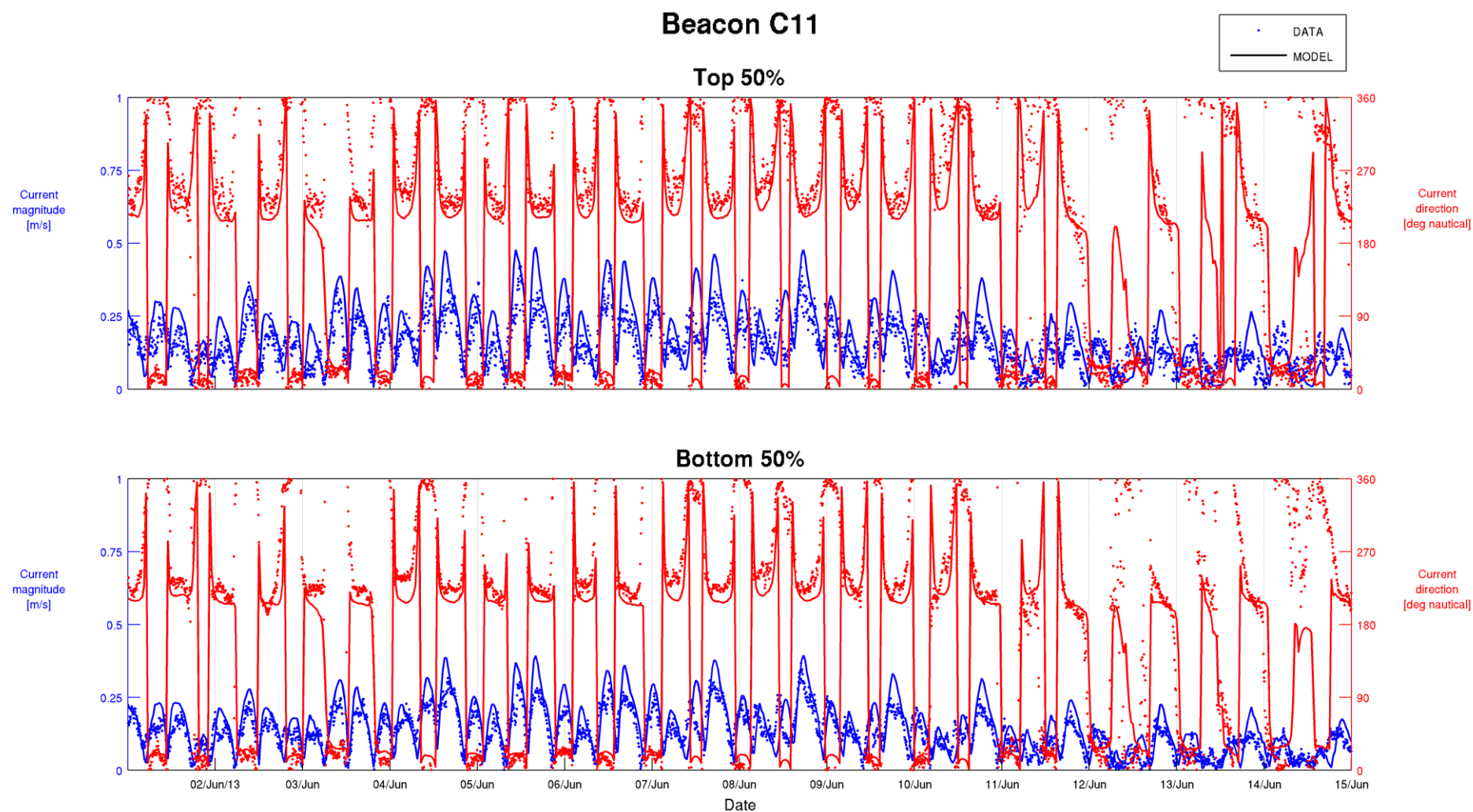
Figure C-28 Top 50% and Bottom 50% Current Calibration – Beacon C11 01/06/2013 to 15/06/2013
