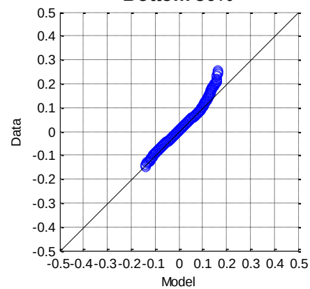
Figure E-2 Current Q-Q Plot – Site 2
