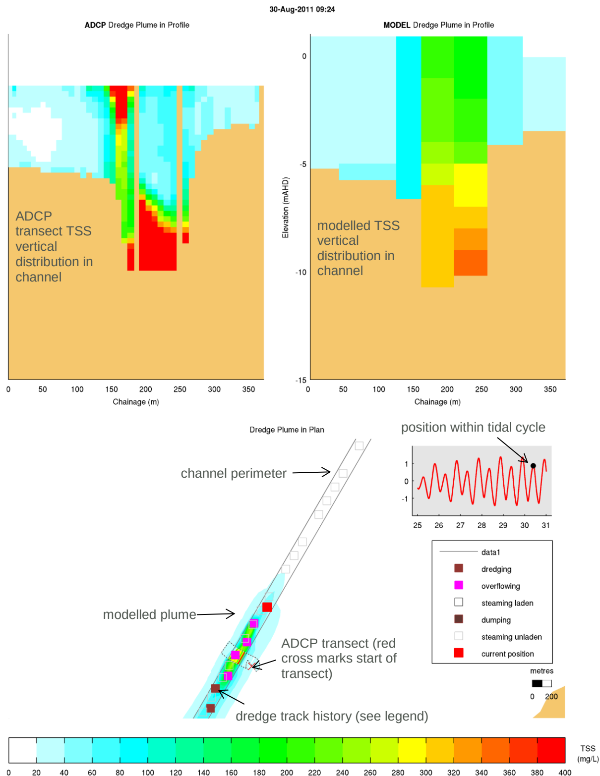
Figure 4-2 Maintenance Dredging Plume Validation, 30/08/2011 09:24: Recorded Plume (top left) and Modelled Plume (top right) Vertical Distribution; Recorded and Modelled Plume Plan View (bottom)
