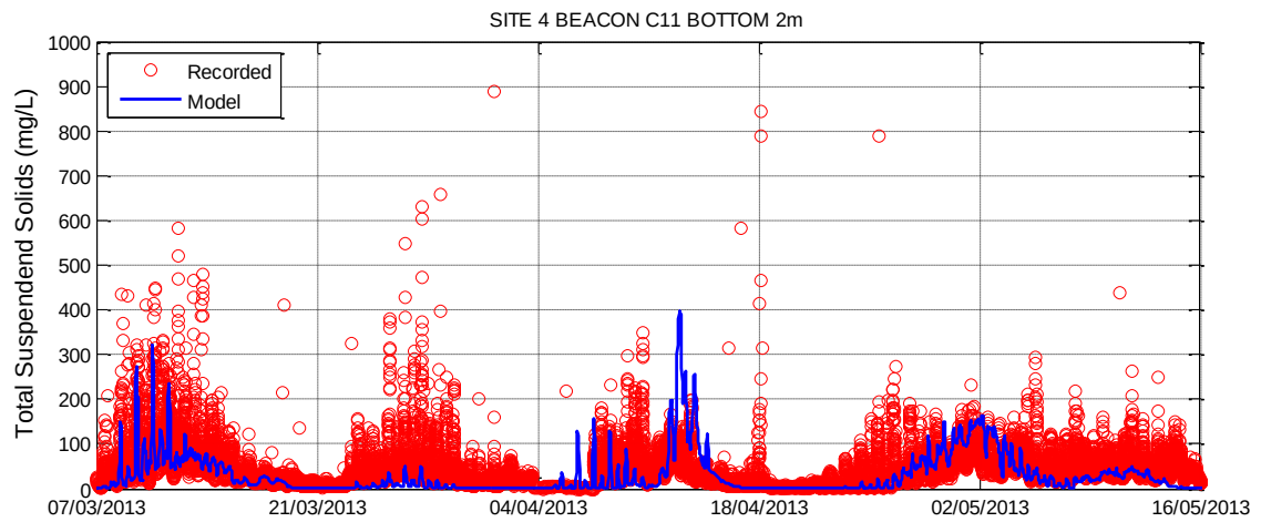
Figure 3-41 Sediment Re-suspension Calibration – Beacon C11
