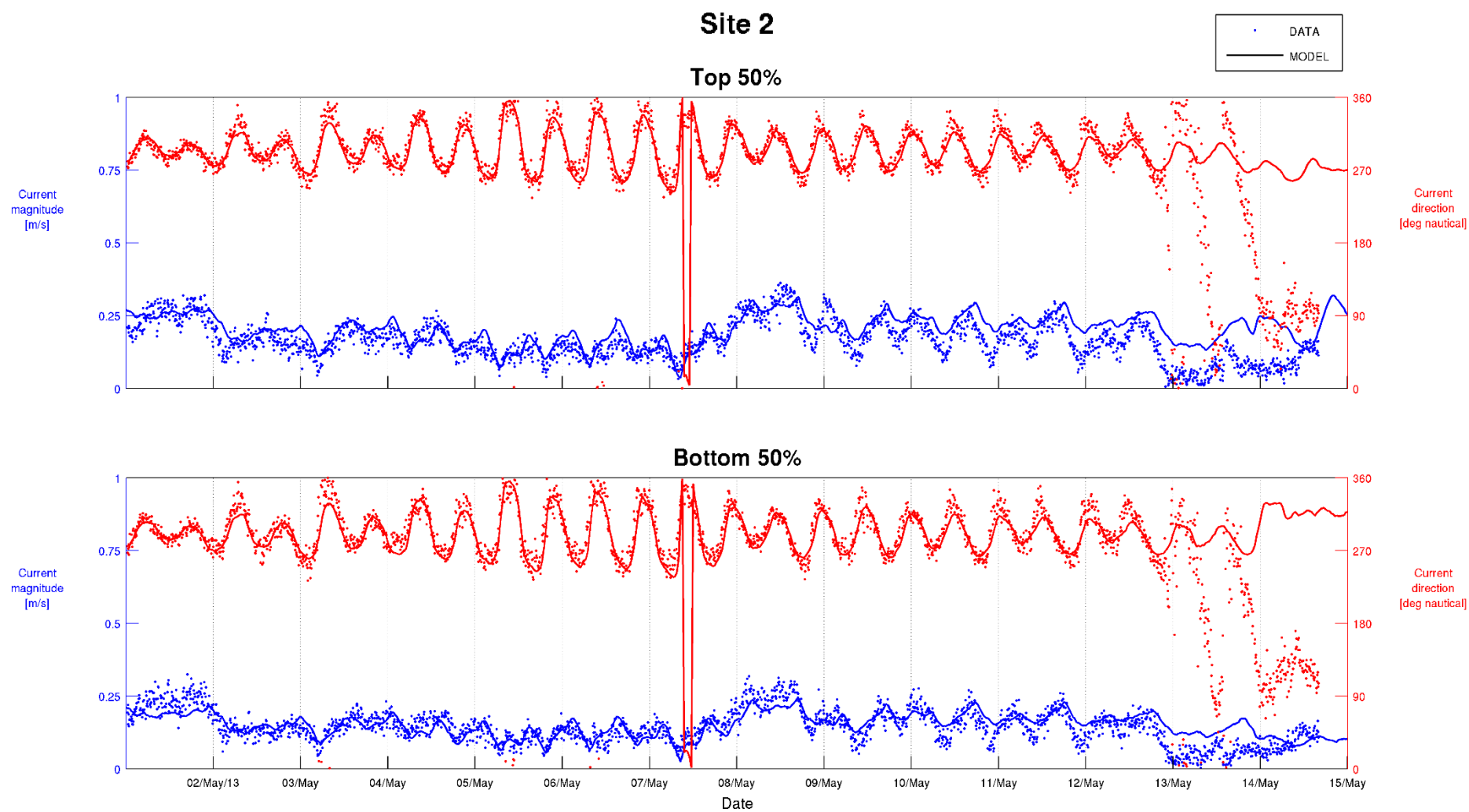
Figure C-12 Top 50% and Bottom 50% Current Calibration – Site 2 01/05/2013 to 15/05/2013
