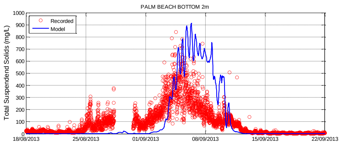
Figure 5-26 Sediment Re-suspension Validation – Palm Beach
