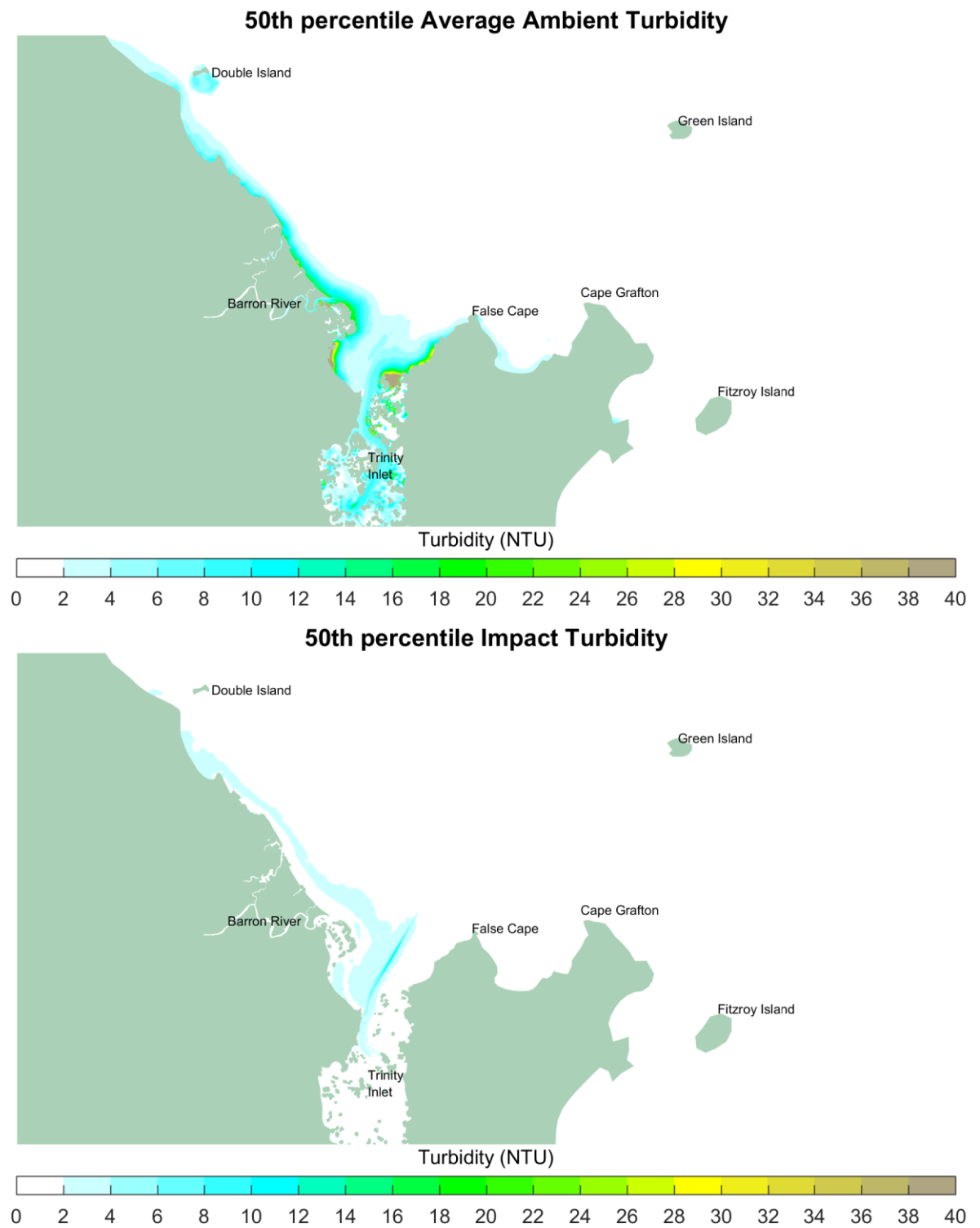
Figure K-4 Likely Best Case 50 th percentile: average ambient (Top), impact of dredging (Bottom)
