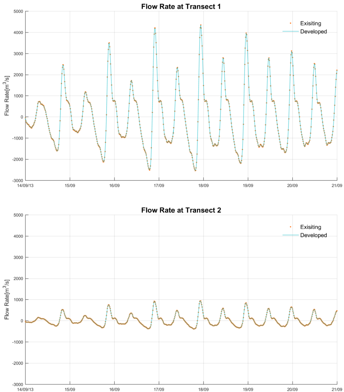
Figure 7-12 Existing and Developed Case Flow Timeseries at Transect 1 and 2 (shown in Figure 7-2)
