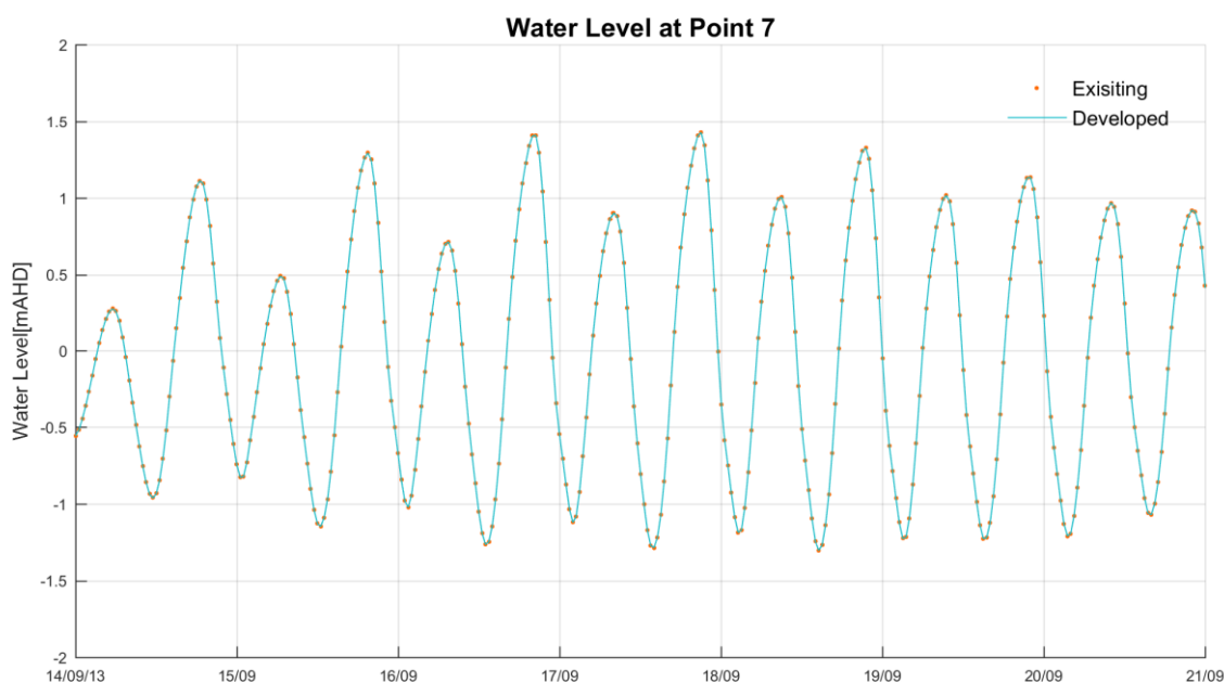
Figure 7-11 Existing and Developed Case Water Level Timeseries (Point 7 – Trinity Inlet)
