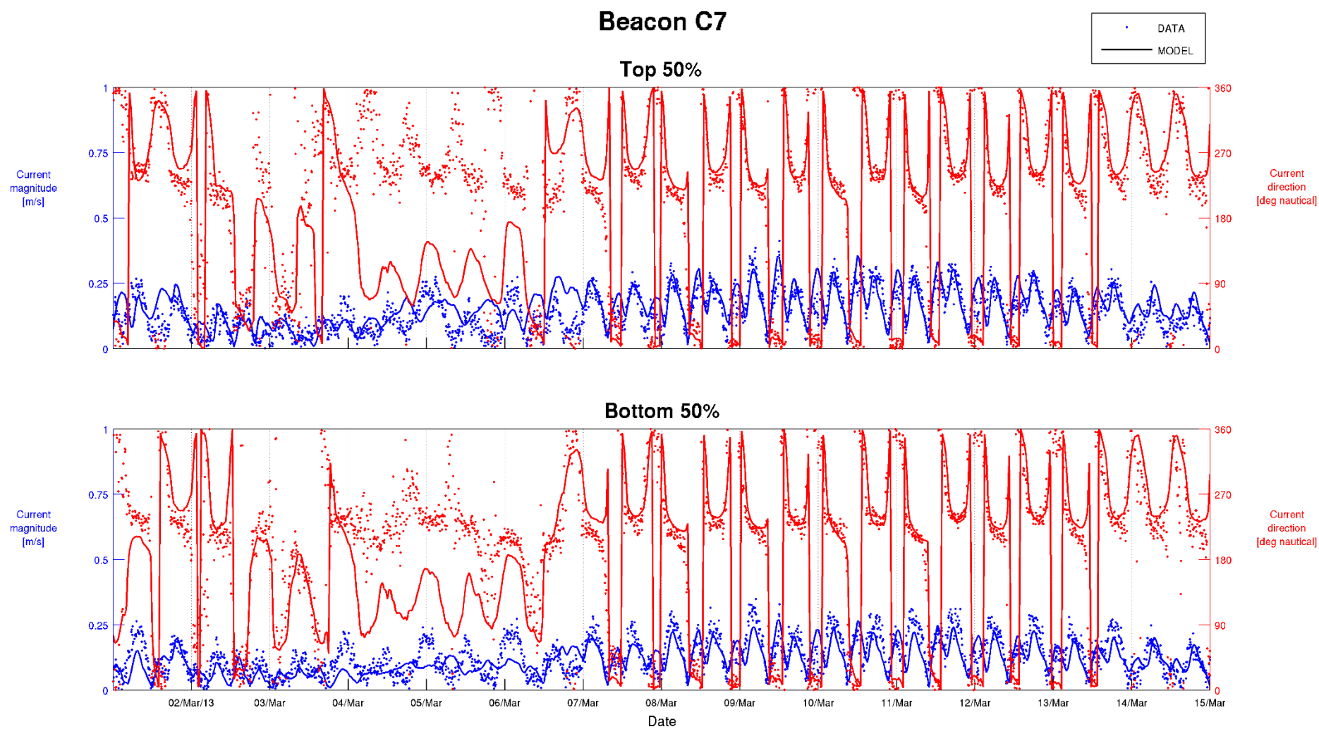
Figure C-15 Top 50% and Bottom 50% Current Calibration – Beacon C7 01/03/2013 to 15/03/2013
