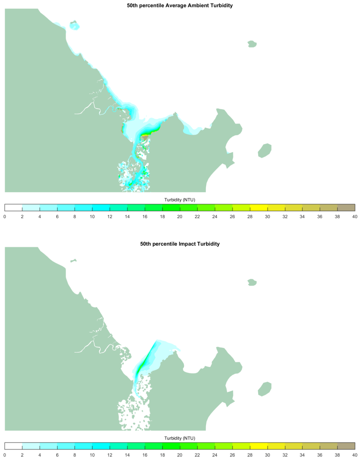
Figure 6-19 Maintenance 50 th Percentiles Turbidity: Average Ambient (Top), Impact of Dredging (bottom)
