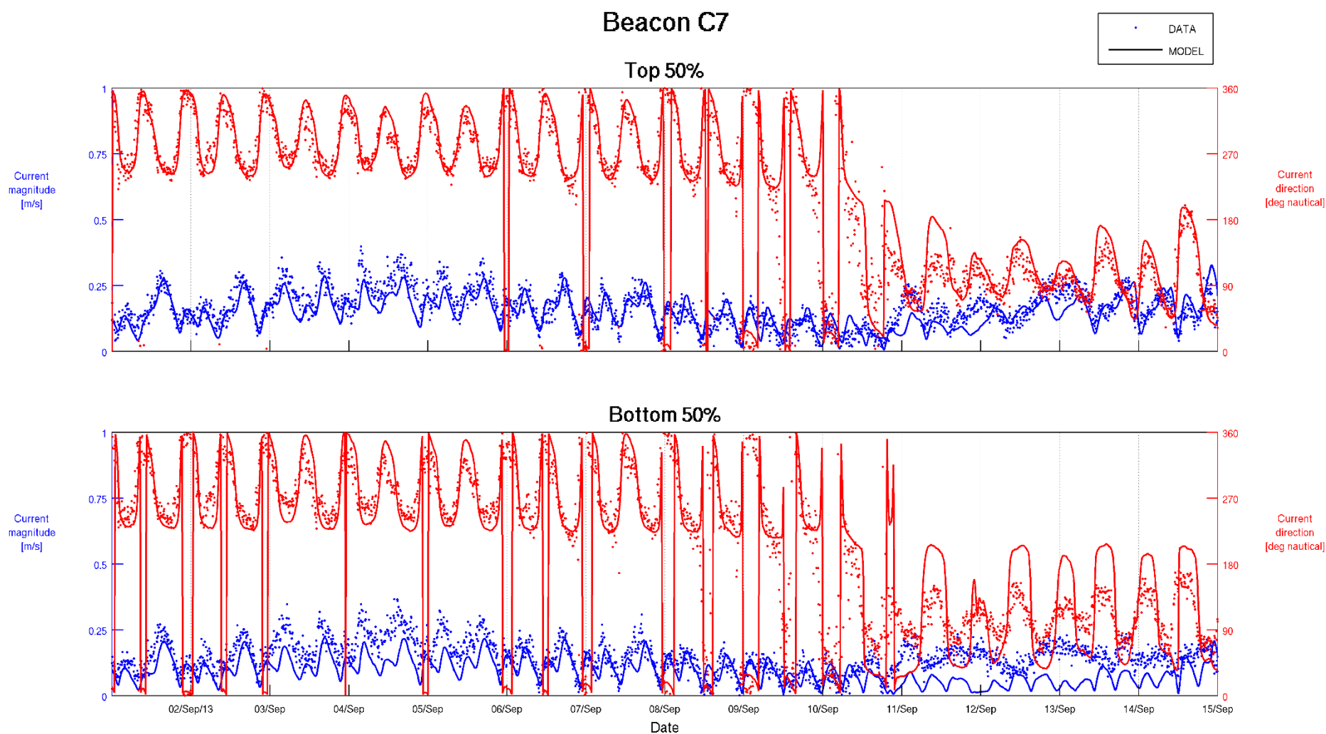
Figure F-13 Top 50% and Bottom 50% Current Validation – Beacon C7 01/09/2013 to 15/09/2013
