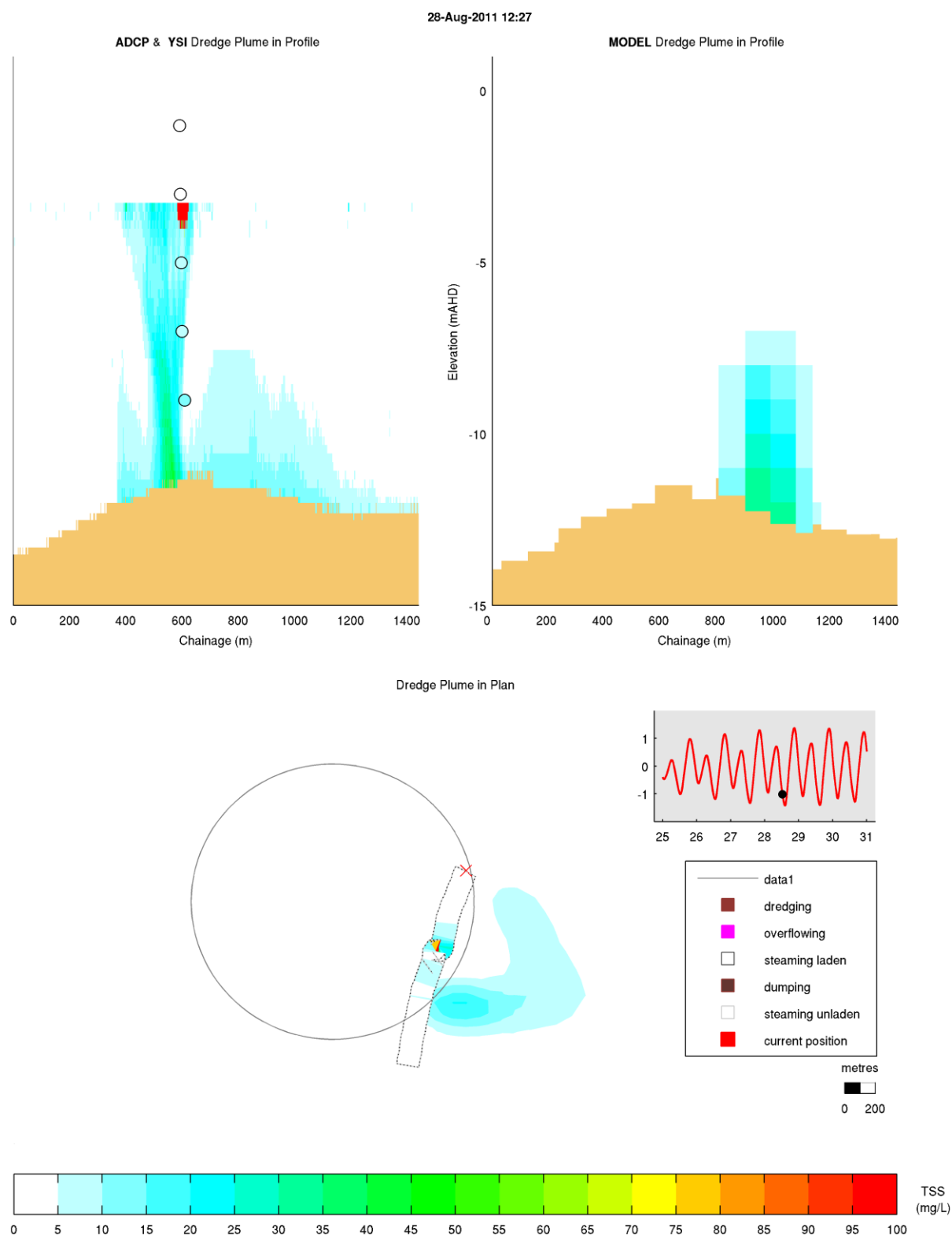
Figure 4-10 DMPA Plume Validation, 28/08/2011 12:27: Recorded Plume (top left) and Modelled Plume (top right) Vertical Distribution; Recorded and Modelled Plume Plan View (bottom)
