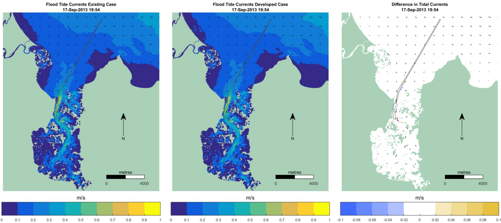
Figure 7-3 Modelled Spring Tide Flood Currents and Impacts. Existing case (left); Developed case (middle) and Impacts (right)
