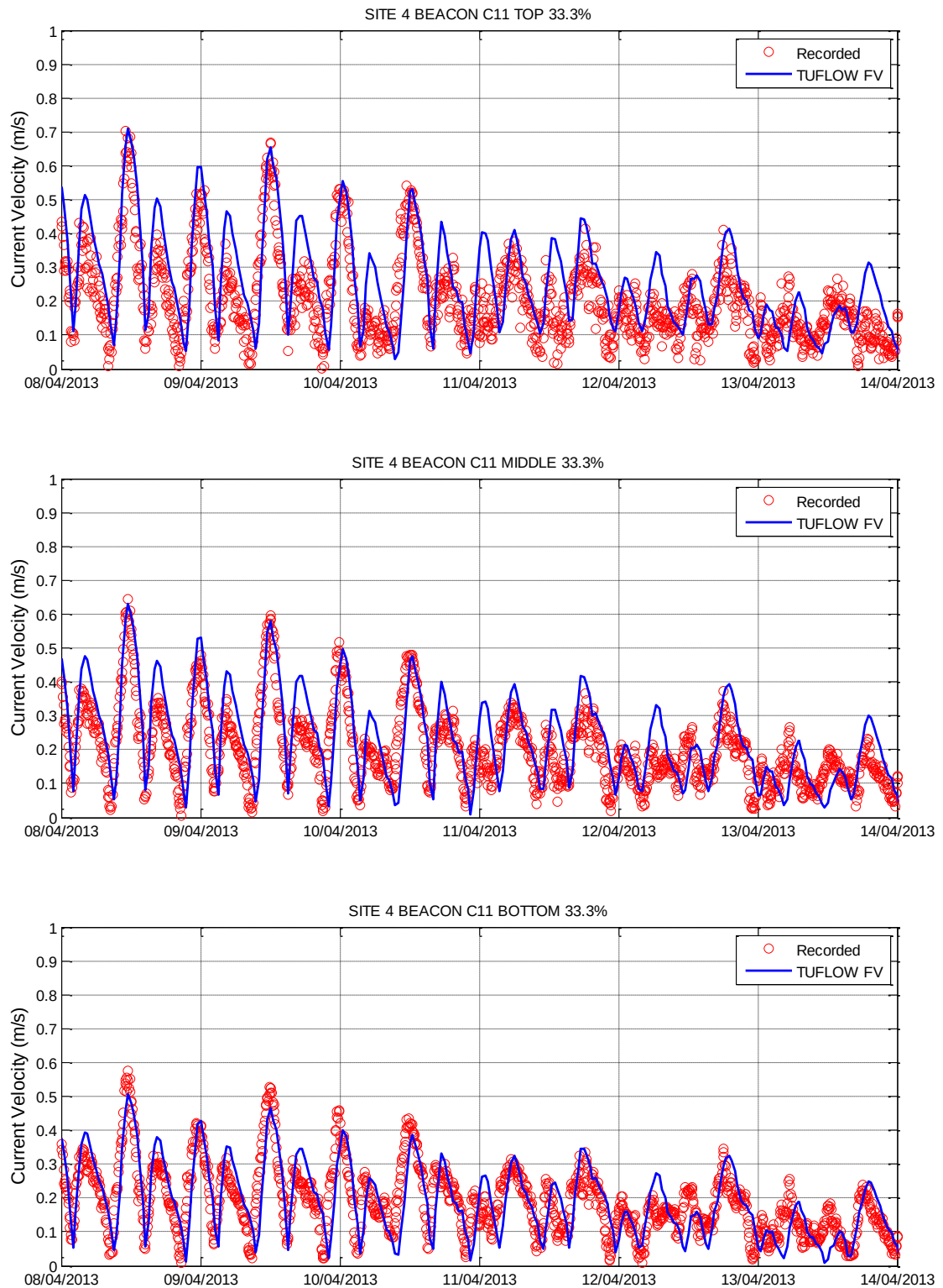
Figure 3-22 Hydrodynamic Model Calibration Current Velocity Layers – Site 4 Beacon C11
