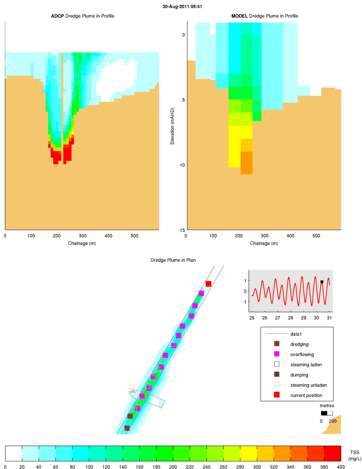
Figure 4-4 Maintenance Dredging Plume Validation, 30/08/2011 09:41: Recorded Plume (top left) and Modelled Plume (top right) Vertical Distribution; Recorded and Modelled Plume Plan View (bottom)
