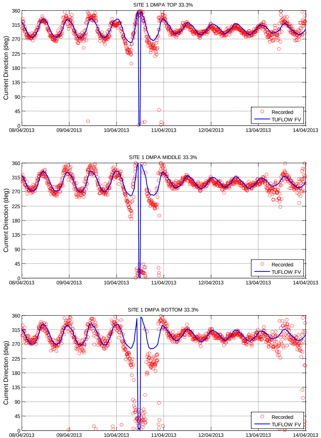
Figure 3-11 Hydrodynamic Model Calibration Current Direction Layers – Site 1 DMPA
