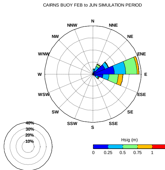
Figure 3-7 Cairns Buoy Wave Rose – February to June 2013
