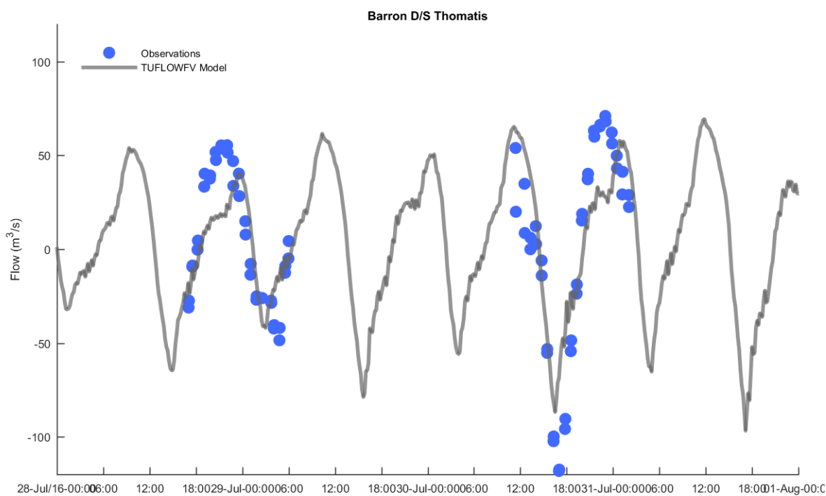
Figure 5-21 Barron River Flows at Transect Downstream of the Richters Creek Confluence
