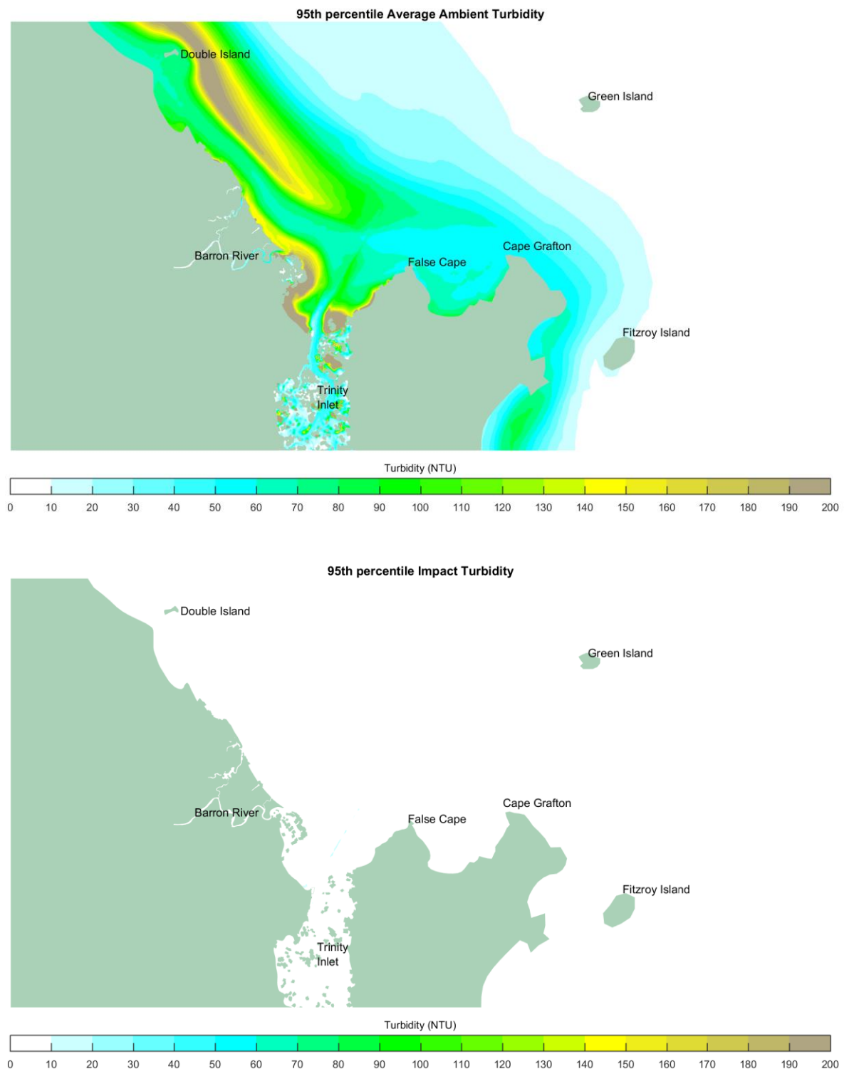
Figure 6-4 Likely Best Case Capital Program 95 th Percentiles Turbidity; Average Ambient Turbidity (Top), Impact of Dredging (Bottom)
