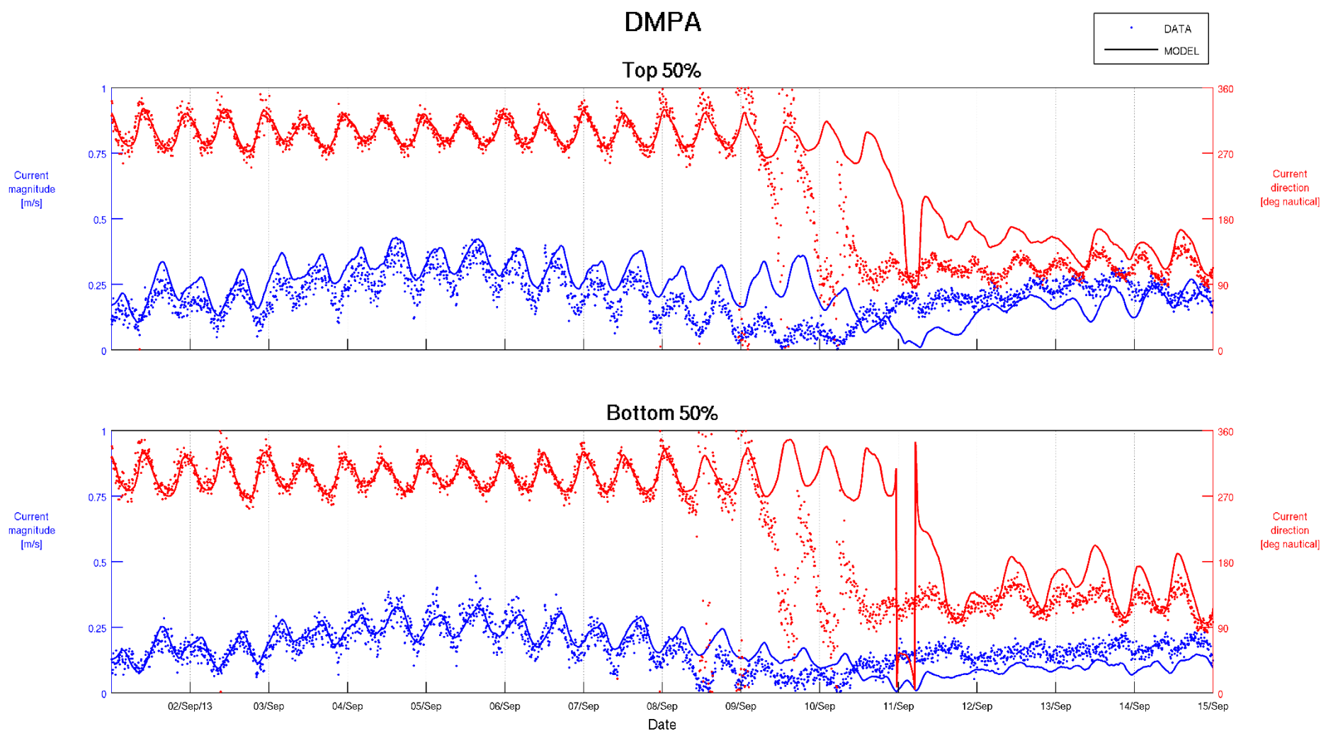
Figure F-6 Top 50% and Bottom 50% Current Validation – DMPA 01/09/2013 to 15/09/2013
