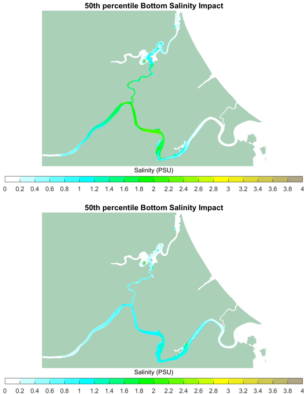
Figure 6-13 Impact to 50 th Percentile Bottom Salinity: Site 1 (Top), Site 2 (Bottom)
