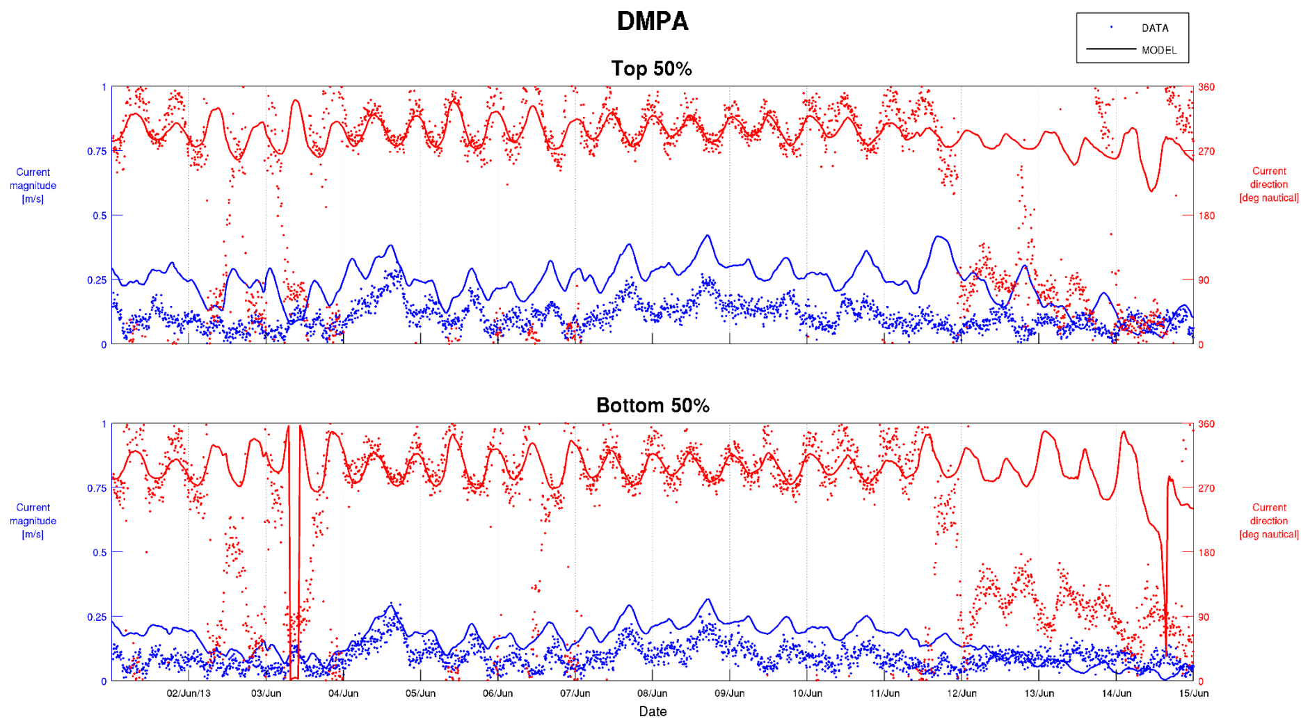
Figure C-7 Top 50% and Bottom 50% Current Calibration – DMPA 01/06/2013 to 15/06/2013
