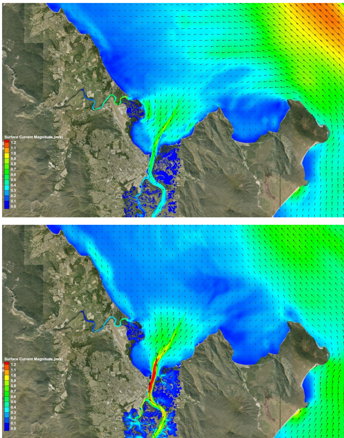
Figure 3-8 Predicted Peak Flood (top) and Peak Ebb (bottom) Surface Current Patterns
