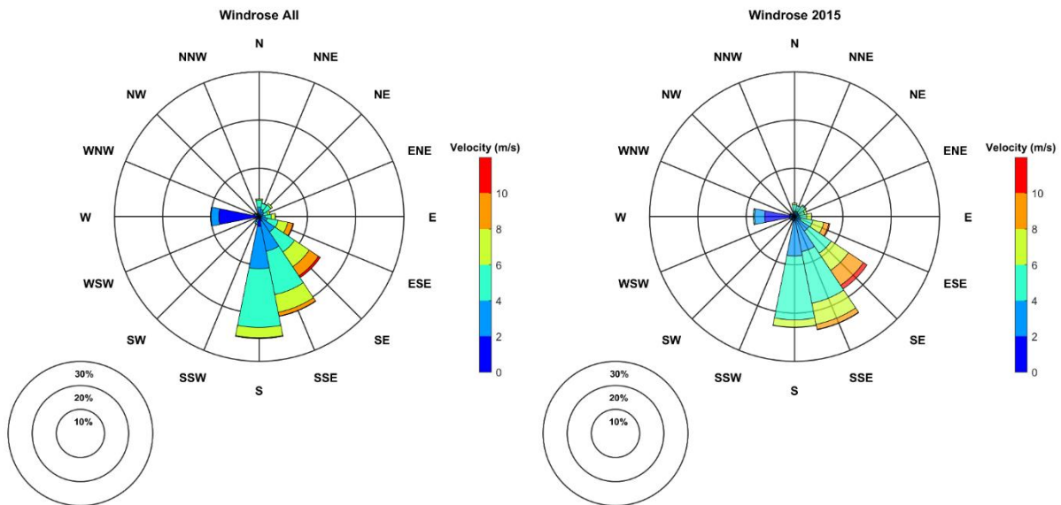
Figure 5-27 Cairns Aero Windroses: All Data (Left), 2015 year (Right)
