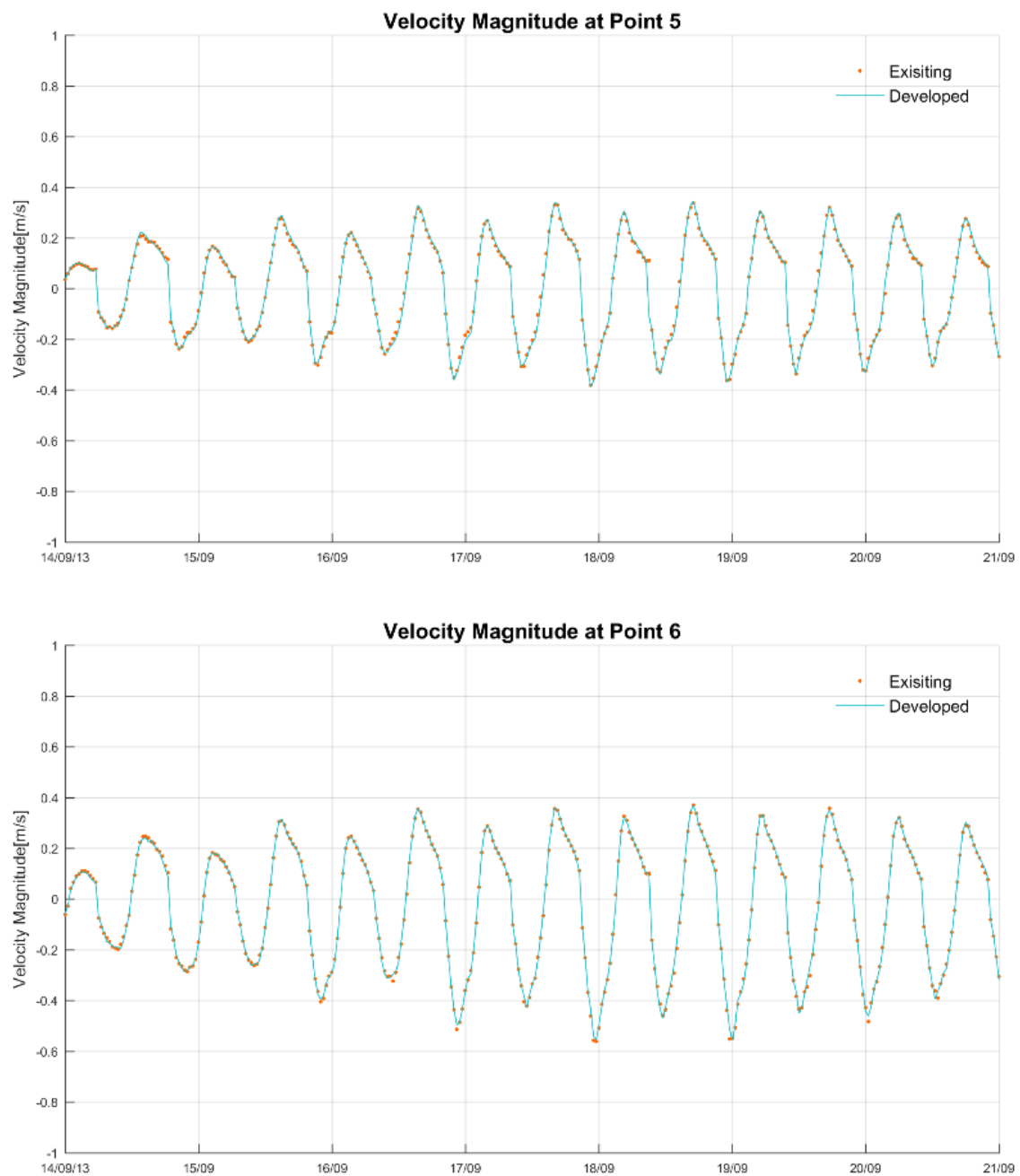
Figure 7-9 Existing and Developed Case Current Speed Timeseries (Points 5 to 6). Positive current speeds are during flooding tides
