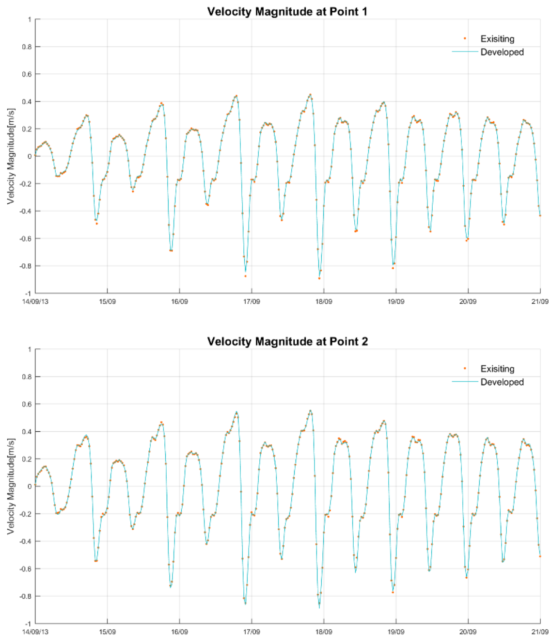
Figure 7-7 Existing and Developed Case Current Speed Timeseries (Points 1 to 2). Positive current speeds are during flooding tides
