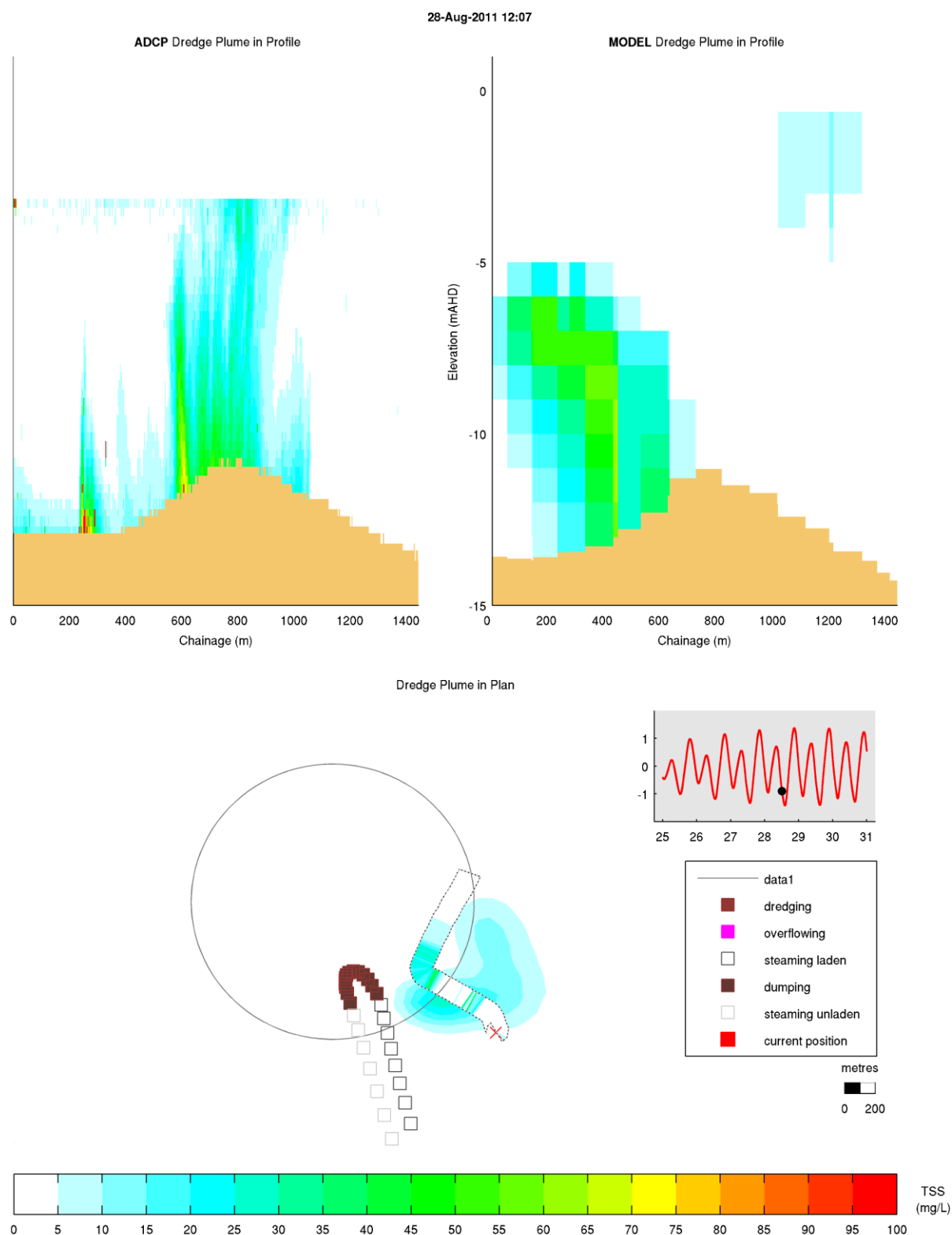
Figure 4-9 DMPA Plume Validation, 28/08/2011 12:07: Recorded Plume (top left) and Modelled Plume (top right) Vertical Distribution; Recorded and Modelled Plume Plan View (bottom)
