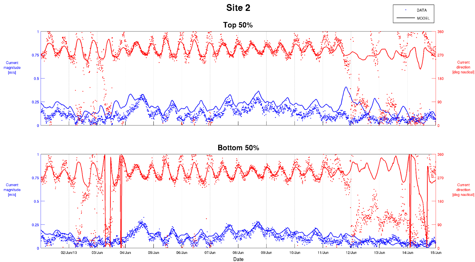
Figure C-14 Top 50% and Bottom 50% Current Calibration – Site 2 01/06/2013 to 15/06/2013
