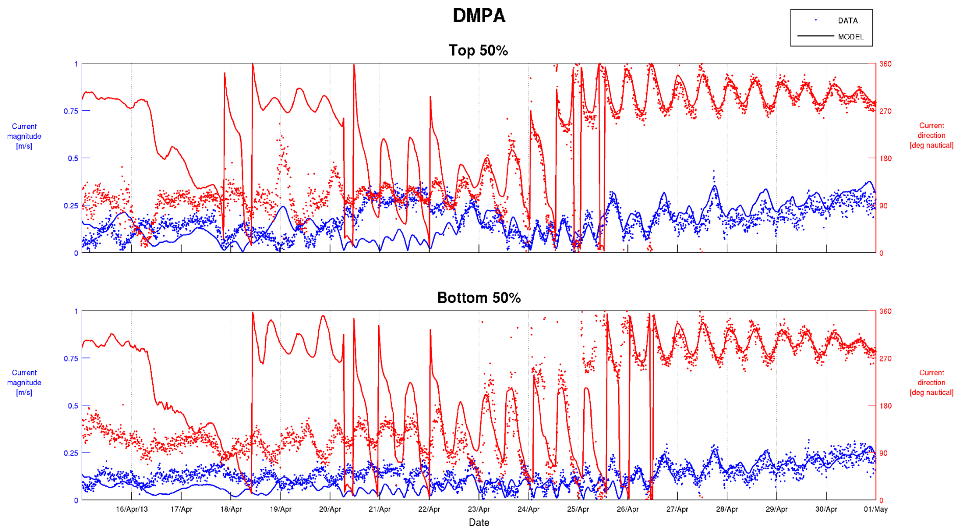
Figure C-4 Top 50% and Bottom 50% Current Calibration – DMPA 15/04/2013 to 01/05/2013
