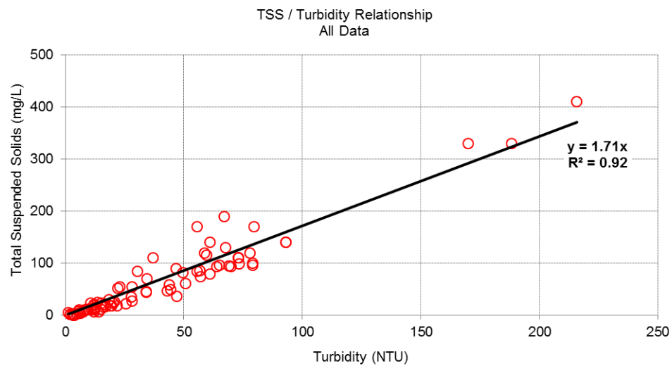
Figure 3-1 NTU-TSS Relationship Established for the Study Area
