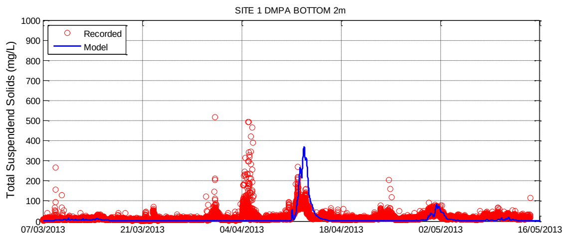
Figure 3-38 Sediment Re-suspension Calibration – DMPA
