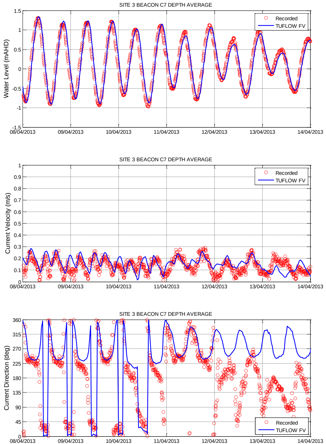
Figure 3-17 Hydrodynamic Model Calibration 3D Depth Average – Site 3 Beacon C7
