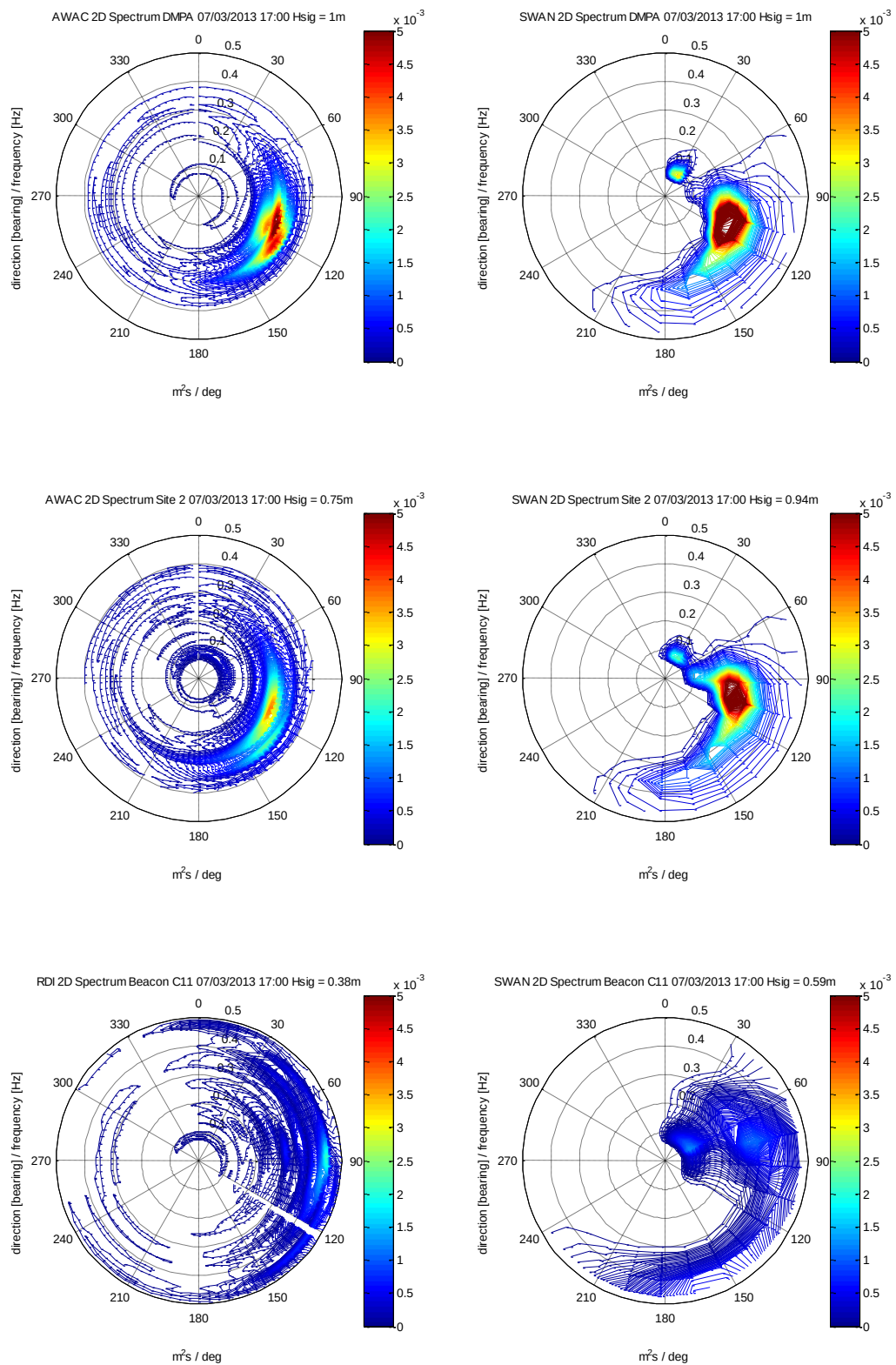
Figure 3-36 Recorded (left) and Predicted (right) 2D Wave Energy Spectrum: Dominant Sea State
