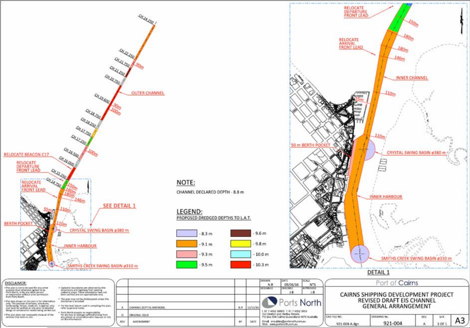
Figure 1-1 Cairns Shipping Development Project Revised General Arrangement
