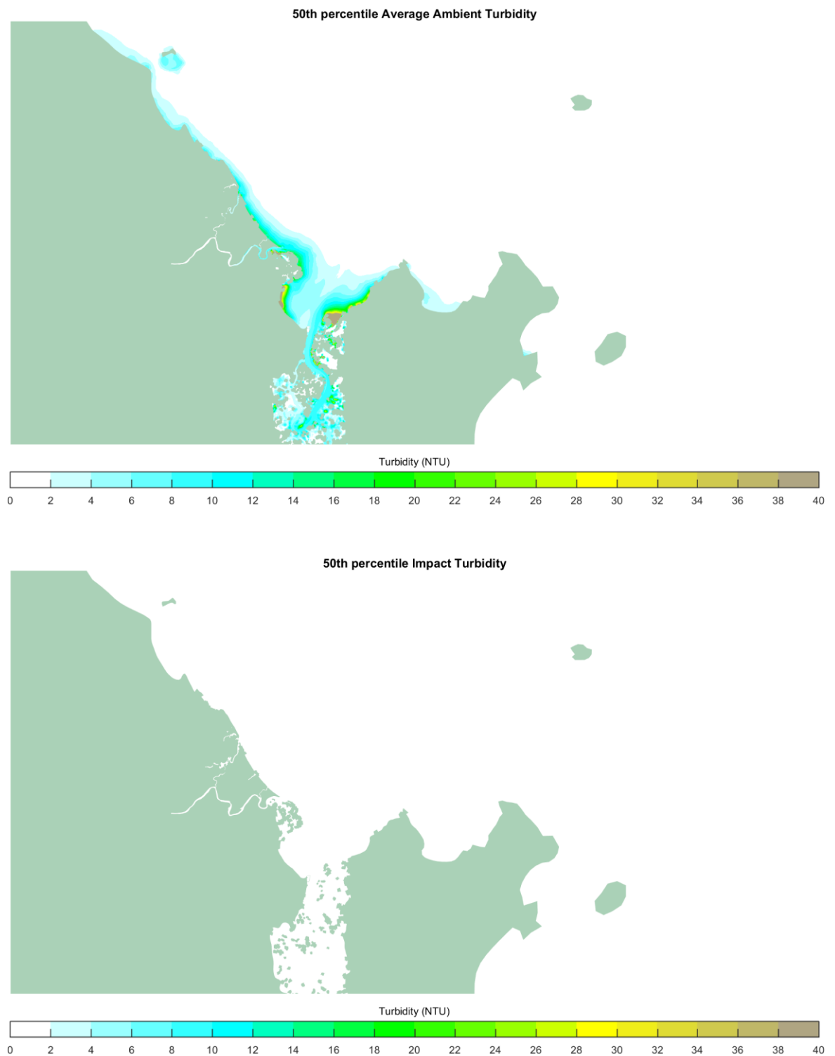
Figure 6-17 Propwash sensitivity 50 th Percentiles Turbidity: Average Ambient (Top), Impact of Dredging (bottom)
