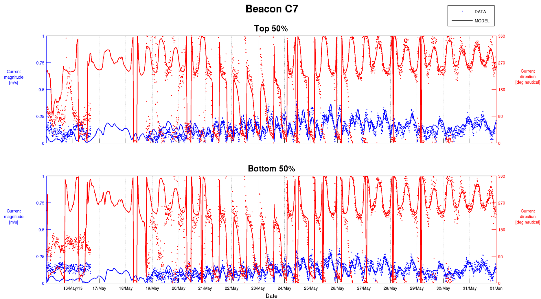
Figure C-20 Top 50% and Bottom 50% Current Calibration – Beacon C7 15/05/2013 to 01/06/2013
