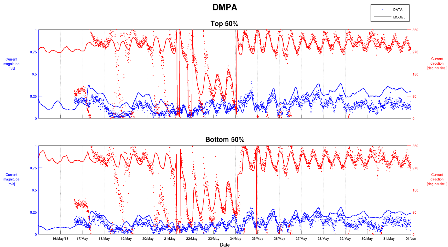
Figure C-6 Top 50% and Bottom 50% Current Calibration – DMPA 15/05/2013 to 01/06/2013
