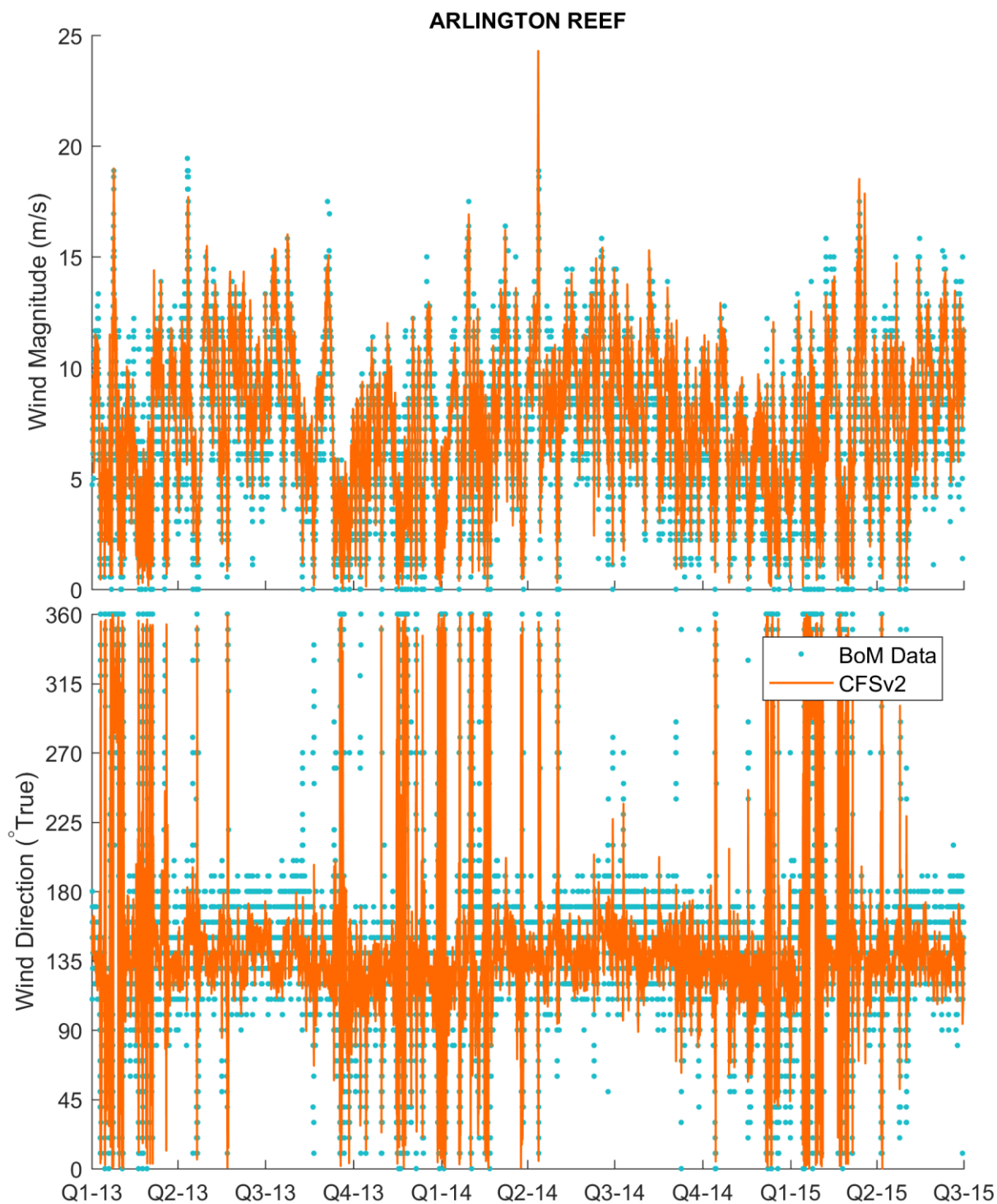
Figure 2-3 Arlington Reef Wind Calibration
