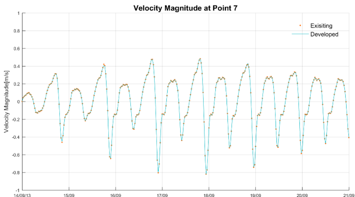
Figure 7-10 Existing and Developed Case Current Speed Timeseries (Point 7). Positive current speeds are during flooding tides
