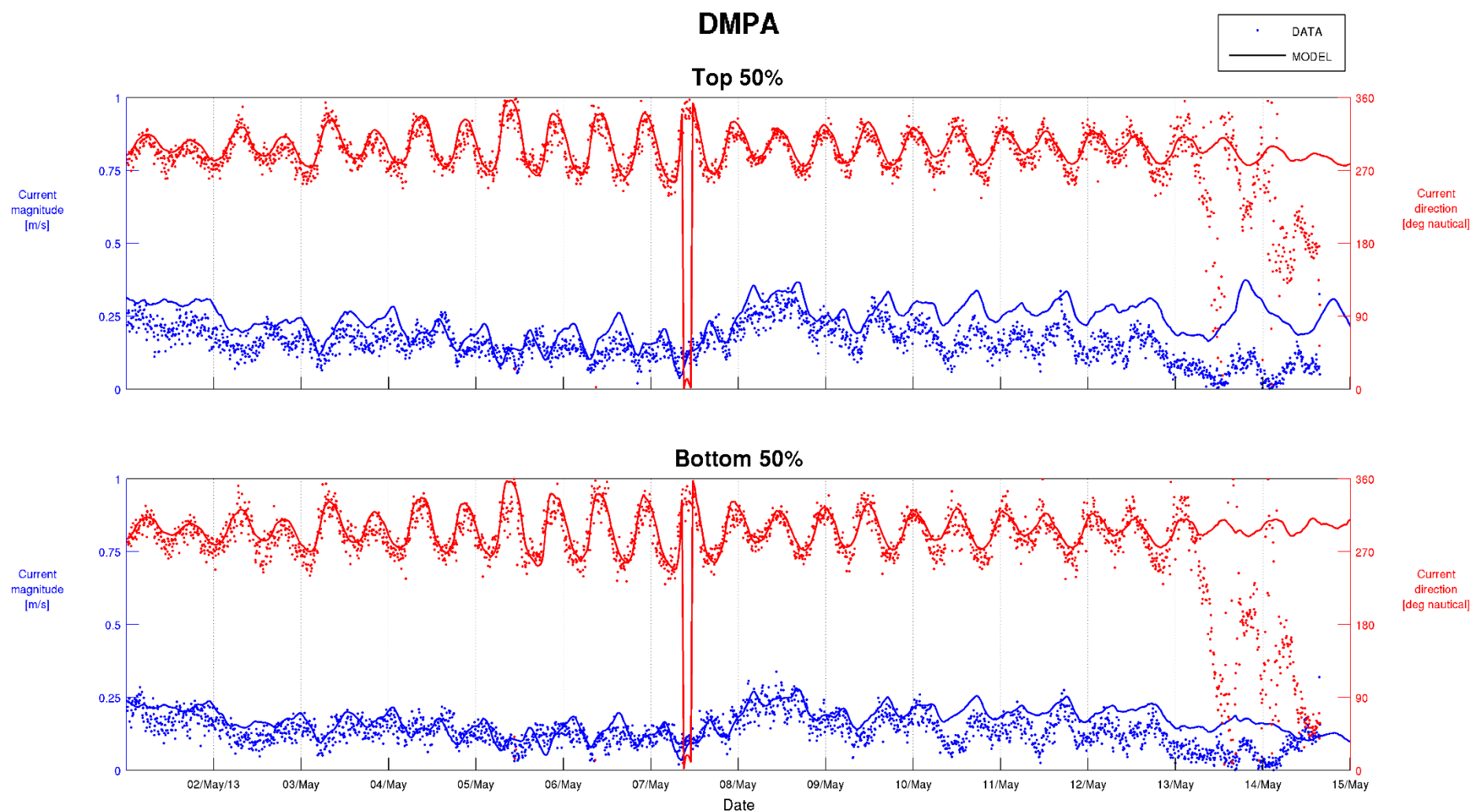
Figure C-5 Top 50% and Bottom 50% Current Calibration – DMPA 01/05/2013 to 15/05/2013
