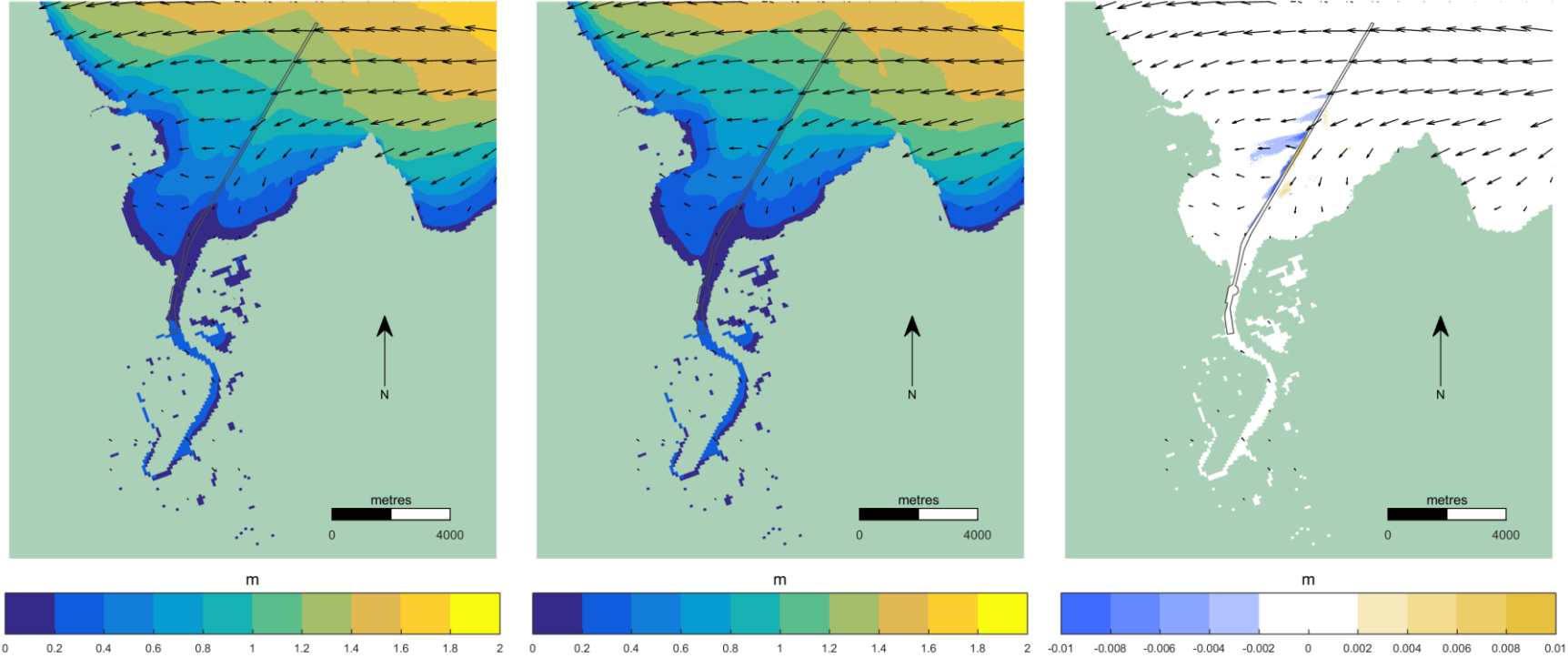
Figure 7-20 25m Grid Typical South-Easterly Wave Case: Base Case (left); Developed Case (middle); Difference (right). Vectors indicate Direction; Contours indicate Magnitude
