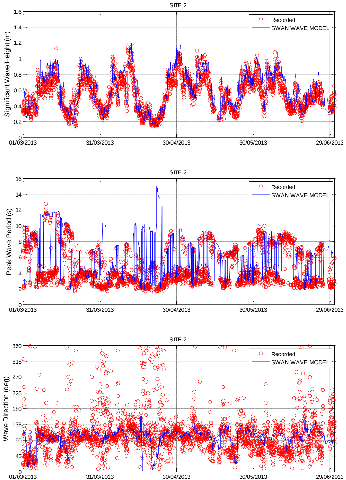
Figure 3-32 SWAN Wave Model Calibration – Site 2
