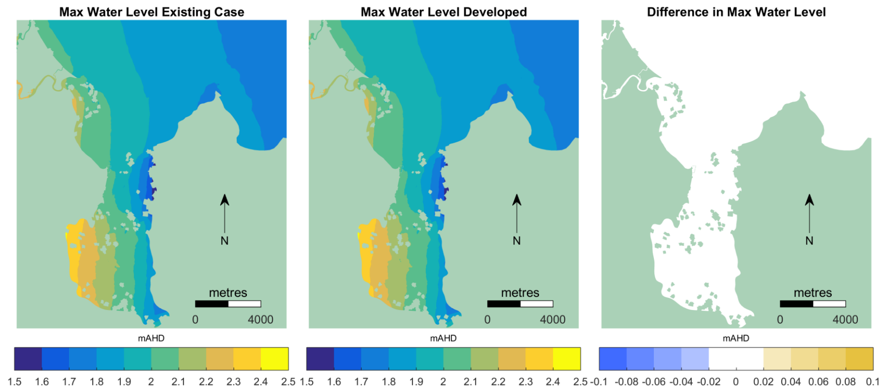
Figure 7-17 Modelled Peak Surge Level (m): Existing case (left); Developed case (middle) and Impacts (right)
