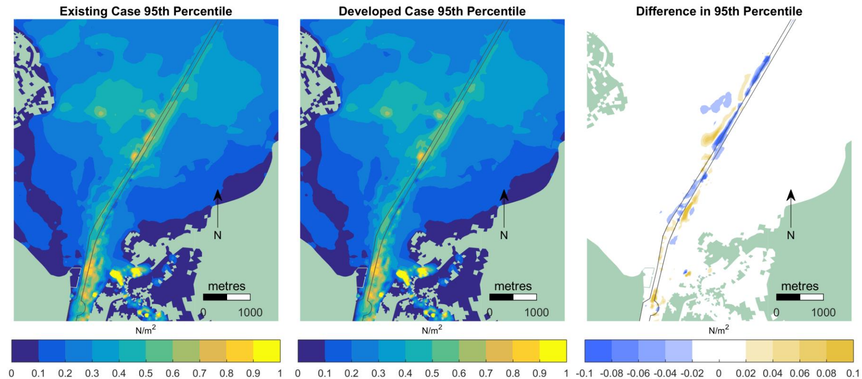
Figure 7-15 Modelled 95%ile Current Related Bed Shear Stress ( N/m^2 ) – zoom. Existing case (left); Developed case (middle) and Impacts (right)
