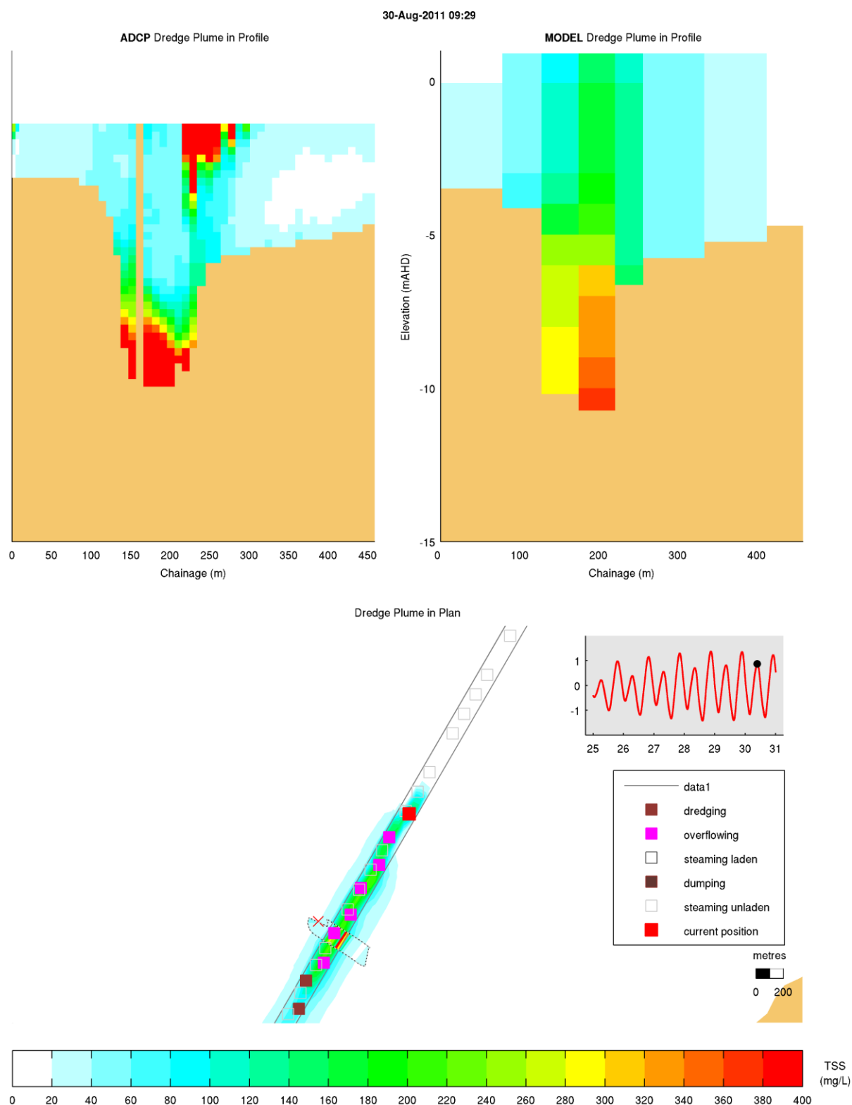
Figure 4-3 Maintenance Dredging Plume Validation, 30/08/2011 09:29: Recorded Plume (top left) and Modelled Plume (top right) Vertical Distribution; Recorded and Modelled Plume Plan View (bottom)
