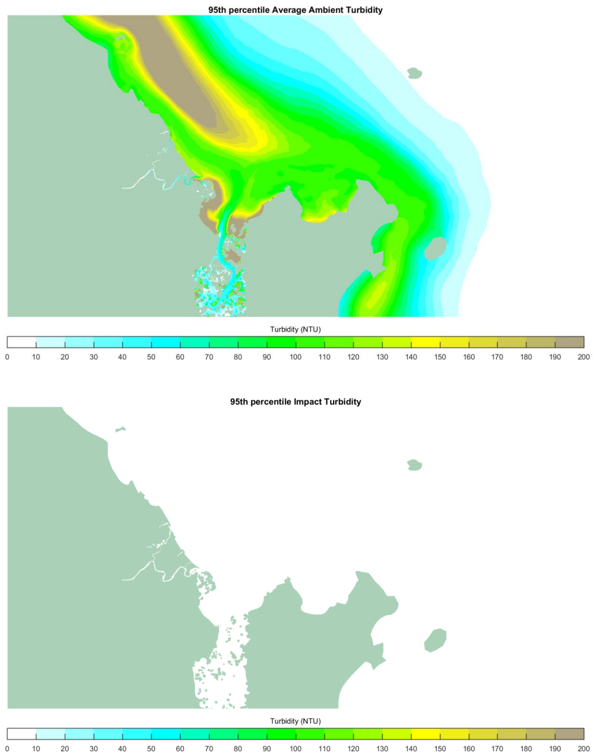
Figure 6-16 Propwash sensitivity 95 th Percentiles Turbidity: Average Ambient (Top), Impact of Dredging (bottom)
