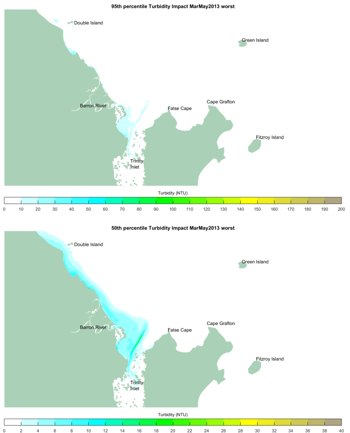
Figure J-5 Scenario 2 MarMay2013: 95 th Percentile (Top), 50 th Percentile (Bottom)
