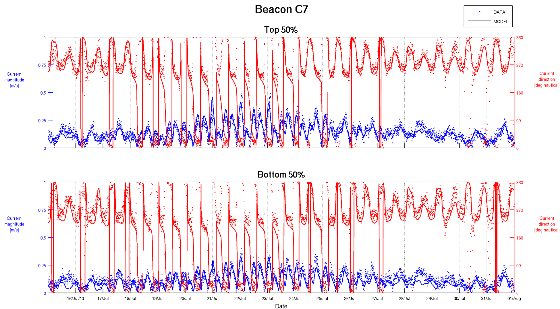
Figure F-10 Top 50% and Bottom 50% Current Validation – Beacon C7 15/07/2013 to 01/08/2013
