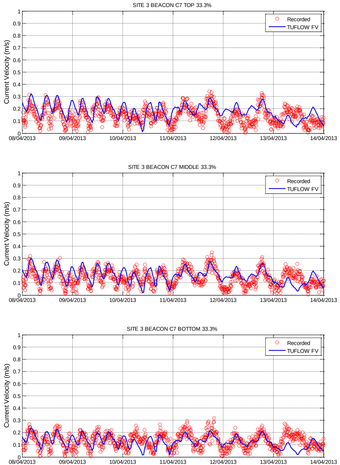
Figure 3-18 Hydrodynamic Model Calibration Current Velocity Layers – Site 3 Beacon C7
