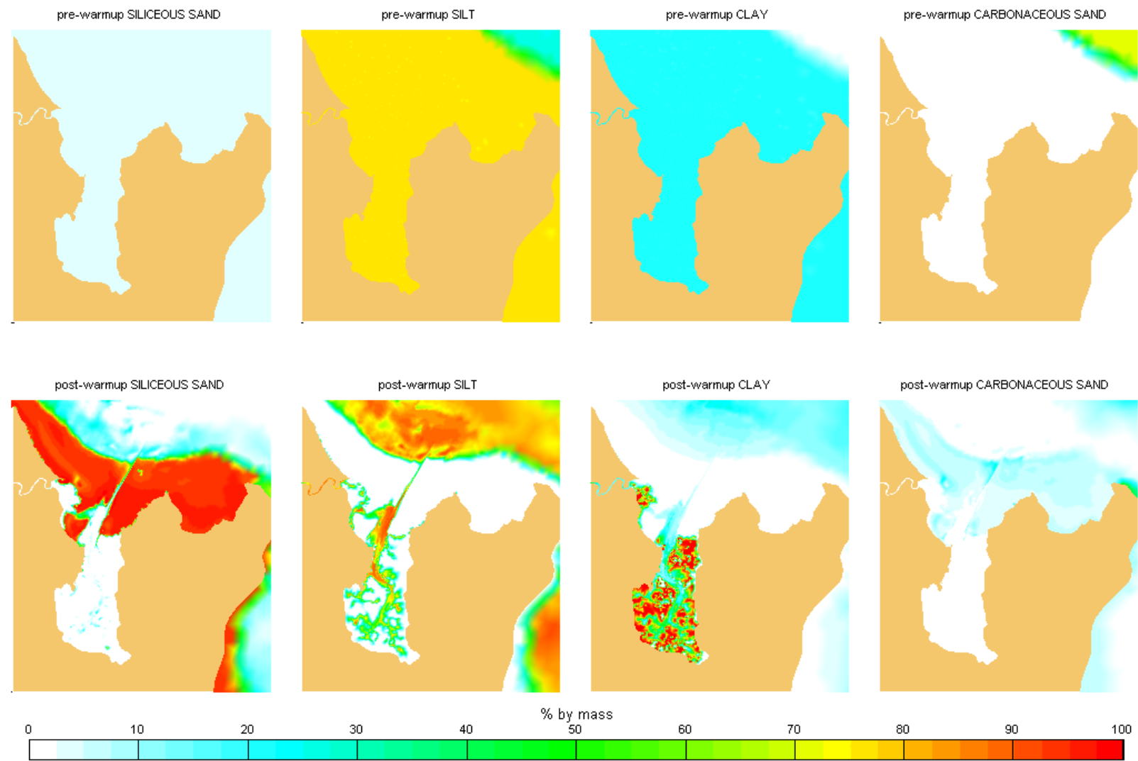
Figure 3-37 “Pre-Warm Up” and “Post-Warm Up” Bed Sediment Distributions
