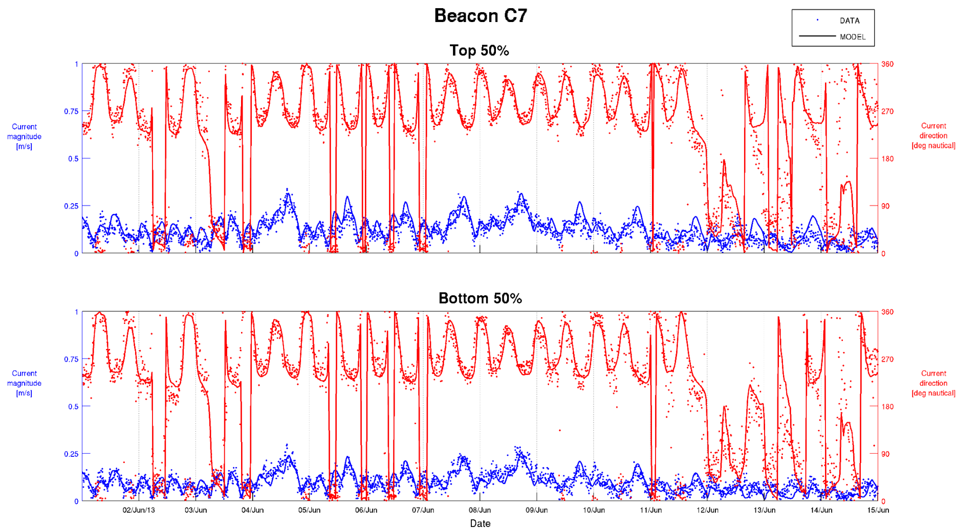
Figure C-21 Top 50% and Bottom 50% Current Calibration – Beacon C7 01/06/2013 to 15/06/2013
