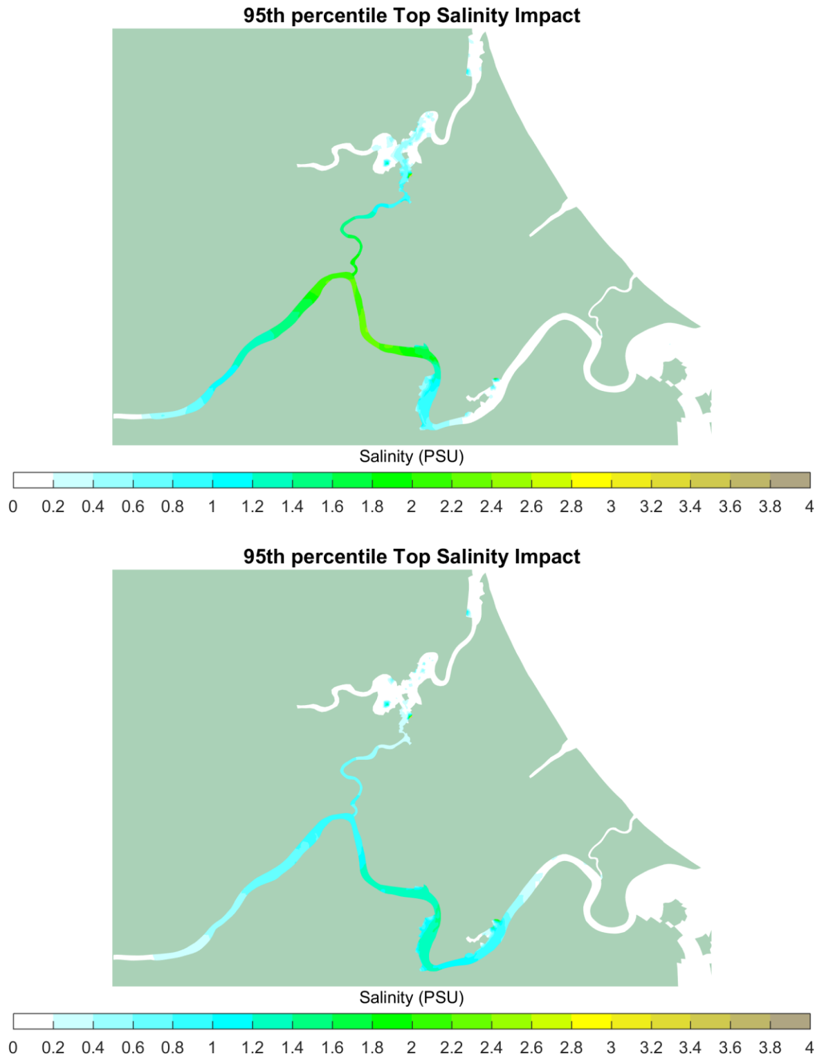
Figure 6-10 Impact to 95 th Percentile Surface Salinity: Site 1 (Top), Site 2 (Bottom)
