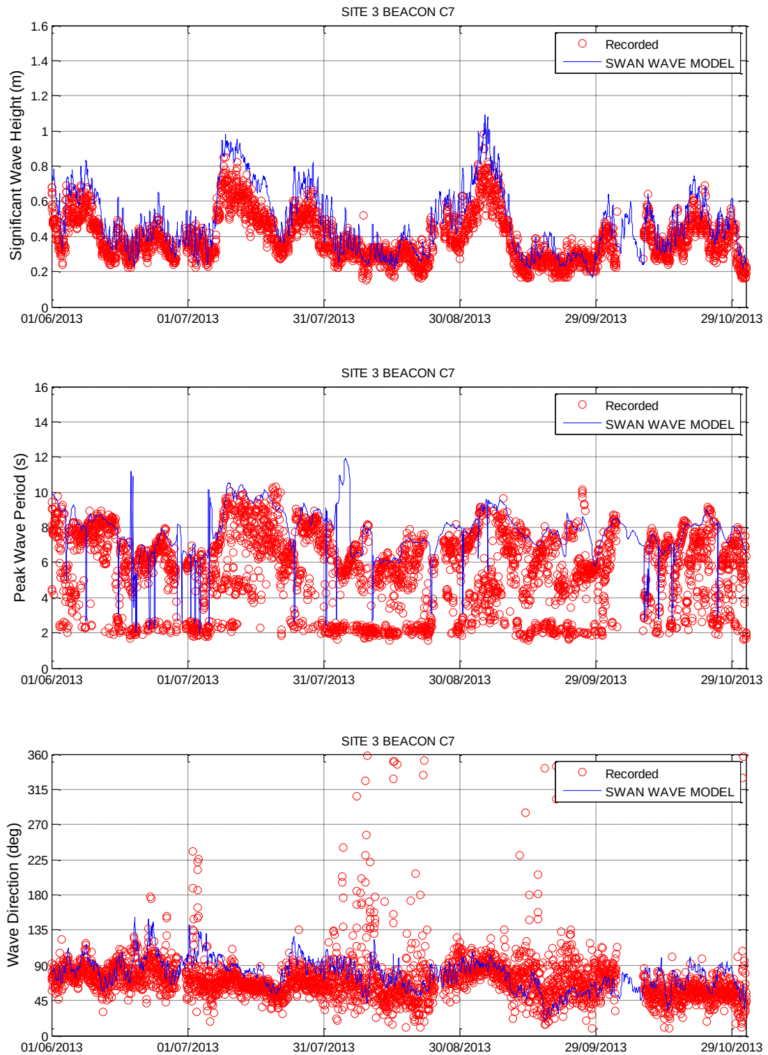
Figure 5-23 SWAN Wave Model Validation – Site 3 Beacon C7
