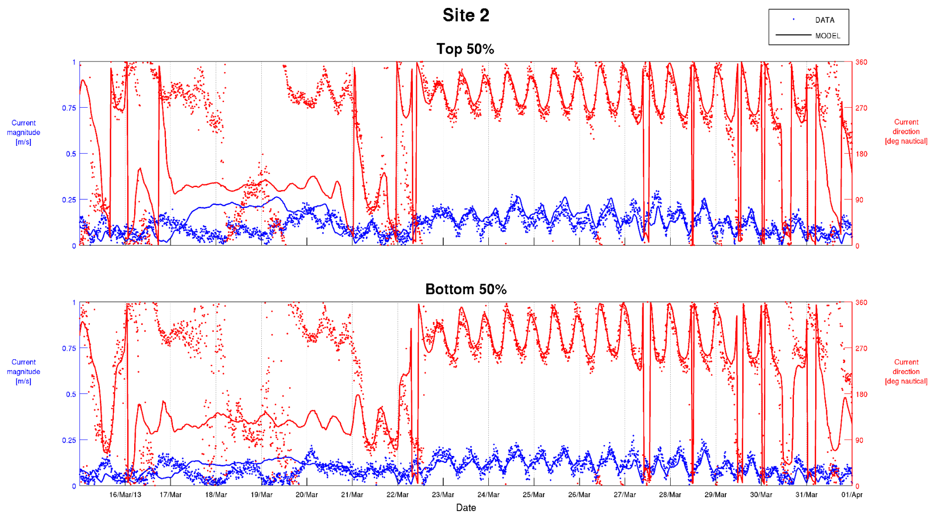
Figure C-9 Top 50% and Bottom 50% Current Calibration – Site 2 15/03/2013 to 01/04/2013
