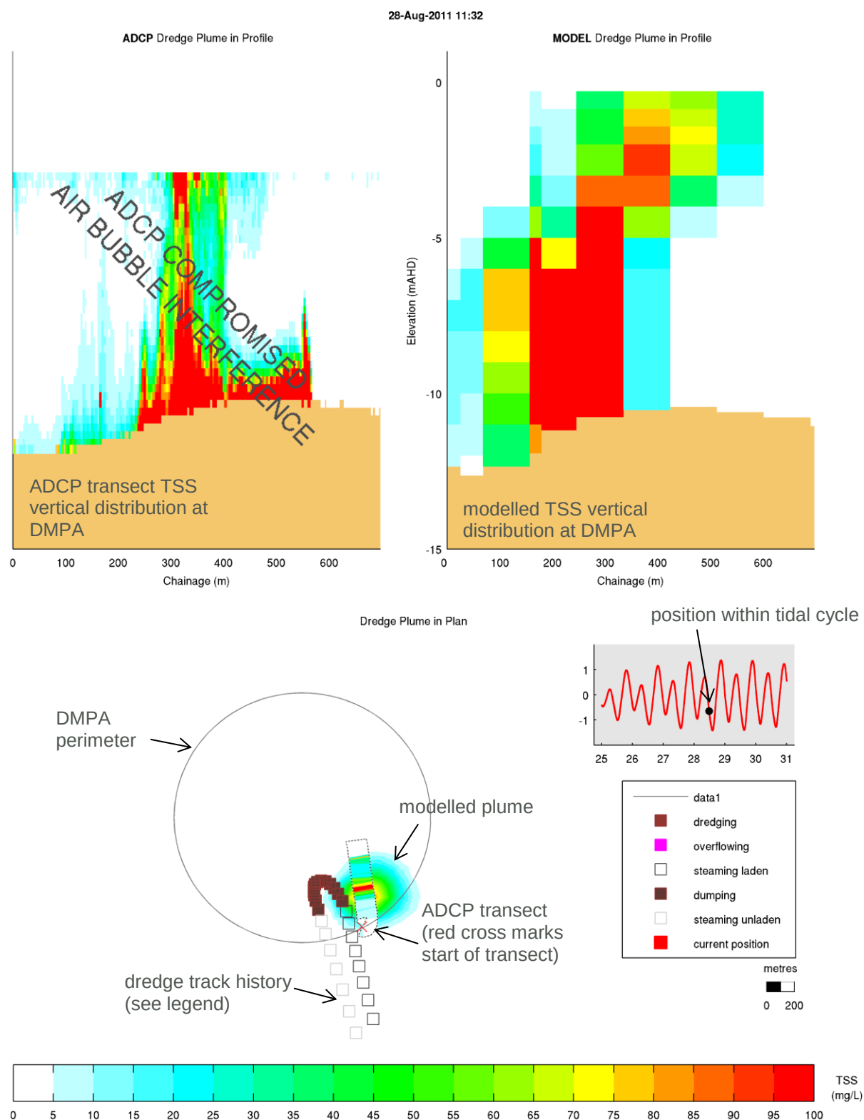
Figure 4-7 DMPA Plume Validation, 28/08/2011 11:32: Recorded Plume (top left) and Modelled Plume (top right) Vertical Distribution; Recorded and Modelled Plume Plan View (bottom)
