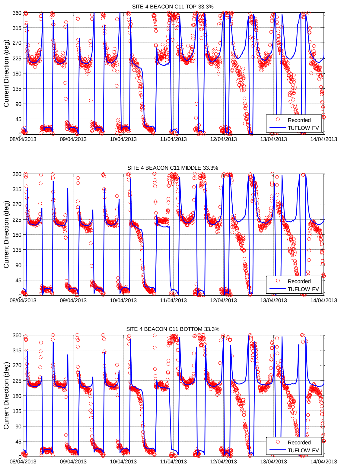
Figure 3-23 Hydrodynamic Model Calibration Current Direction Layers – Site 4 Beacon C11
