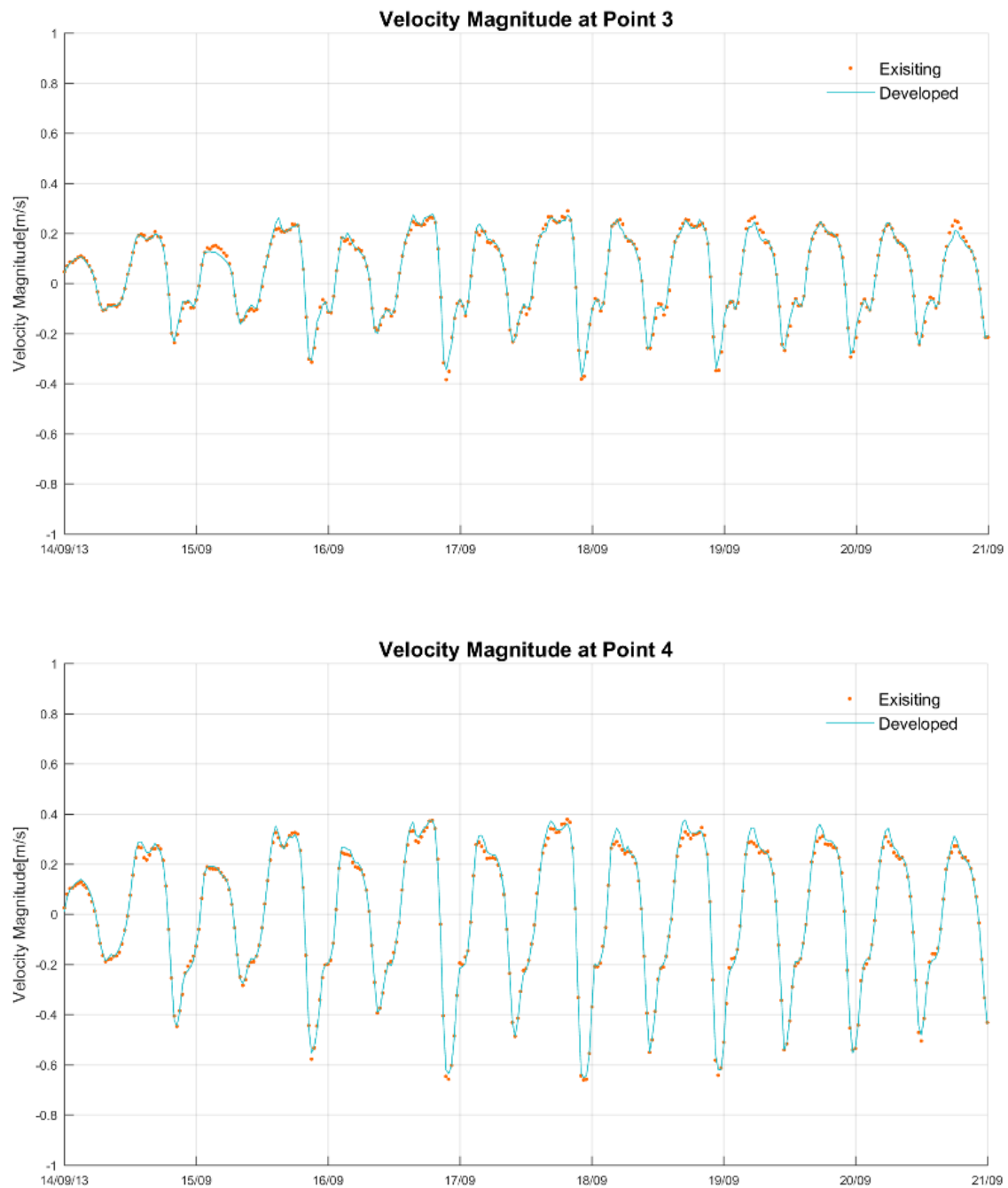
Figure 7-8 Existing and Developed Case Current Speed Timeseries (Points 3 to 4). Positive current speeds are during flooding tides
