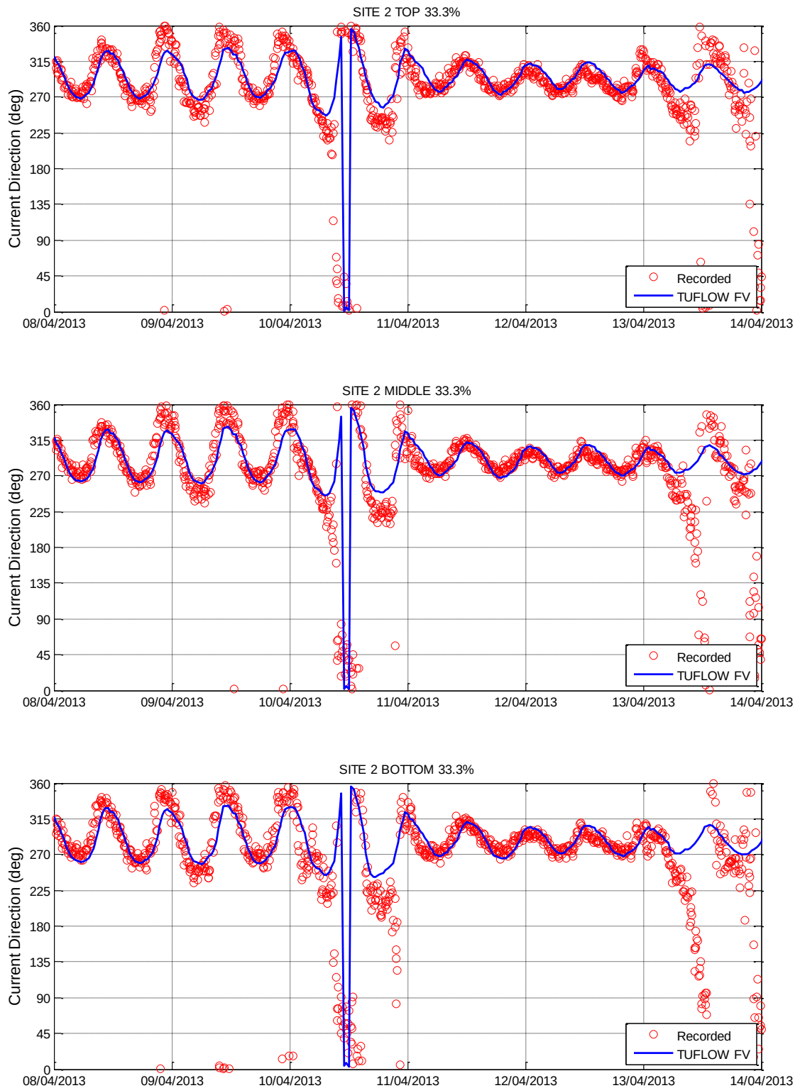
Figure 3-15 Hydrodynamic Model Calibration Current Direction Layers – Site 2
