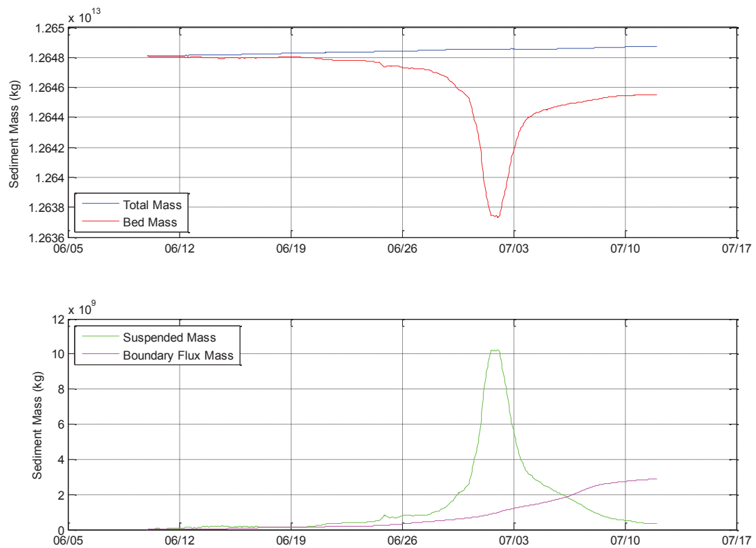
Figure 5. Sediment Mass Balance Checks - Worst Case Stiff Material Dredging
