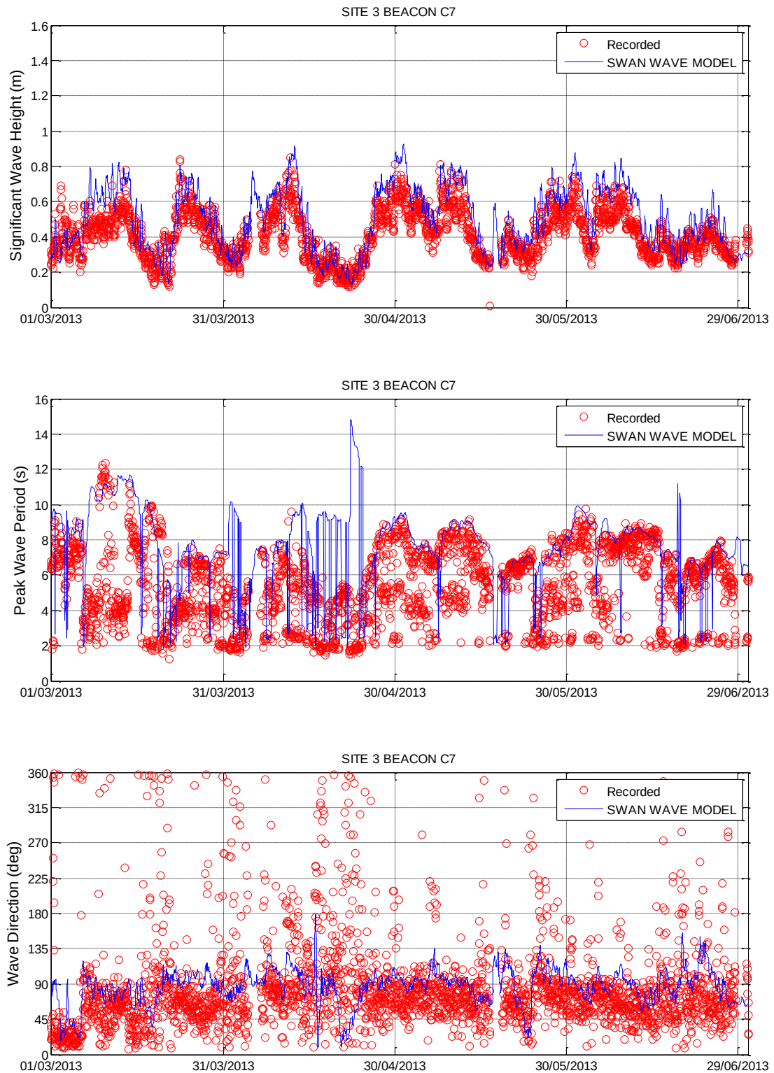
Figure 3-33 SWAN Wave Model Calibration – Site 3 Beacon C7
