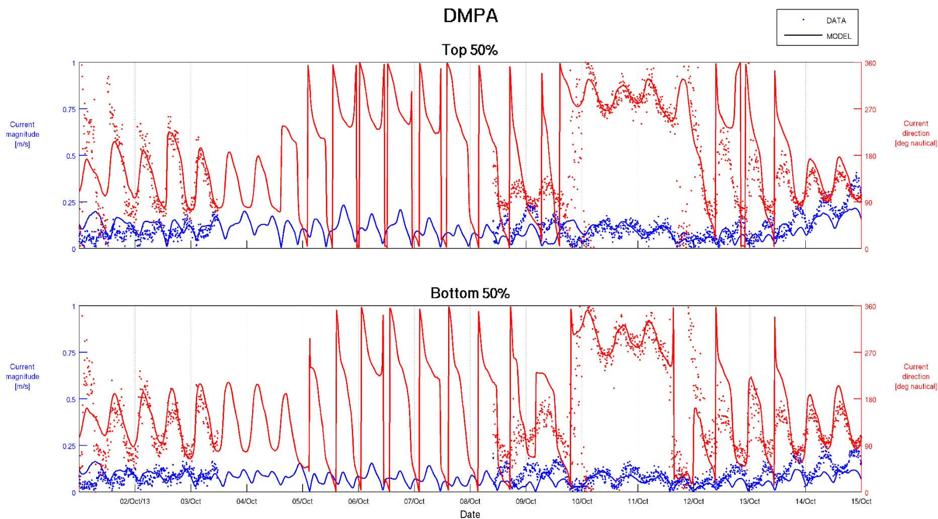
Figure F-8 Top 50% and Bottom 50% Current Validation – DMPA 01/10/2013 to 15/10/2013
