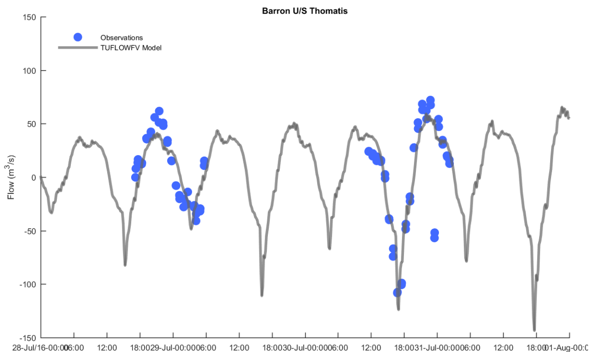
Figure 5-20 Barron River Flows at Transect Upstream of the Richters Creek Confluence
