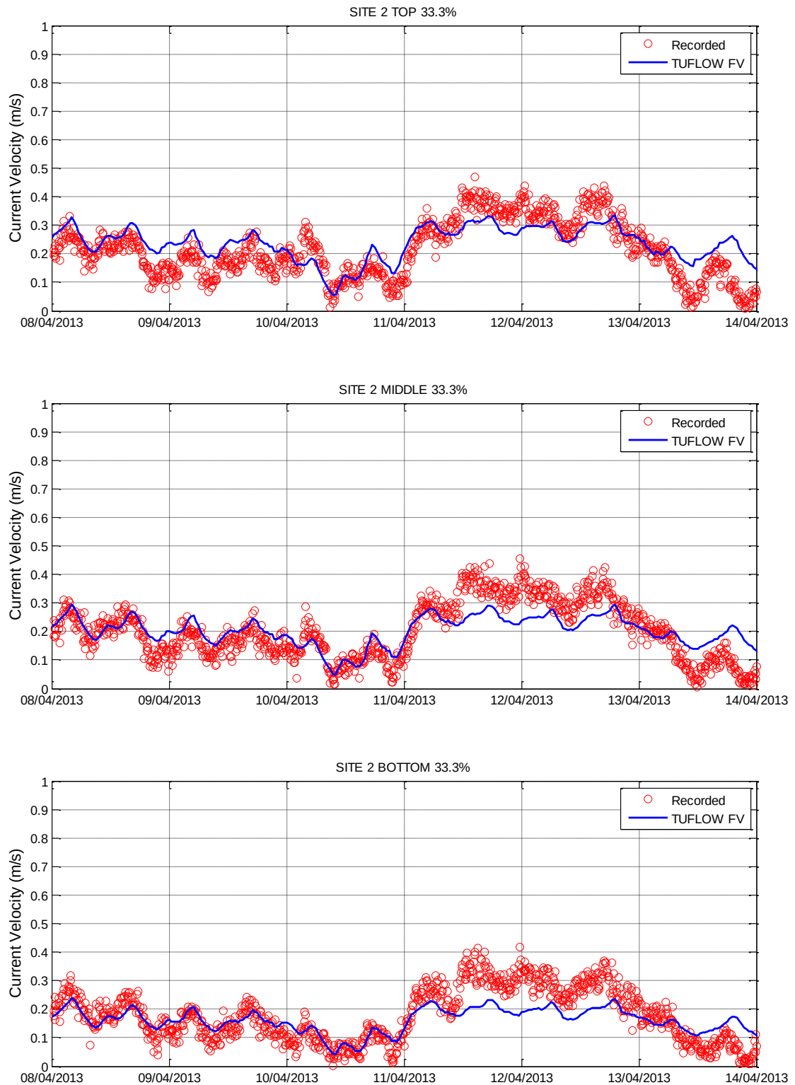
Figure 3-14 Hydrodynamic Model Calibration Current Velocity Layers – Site 2
