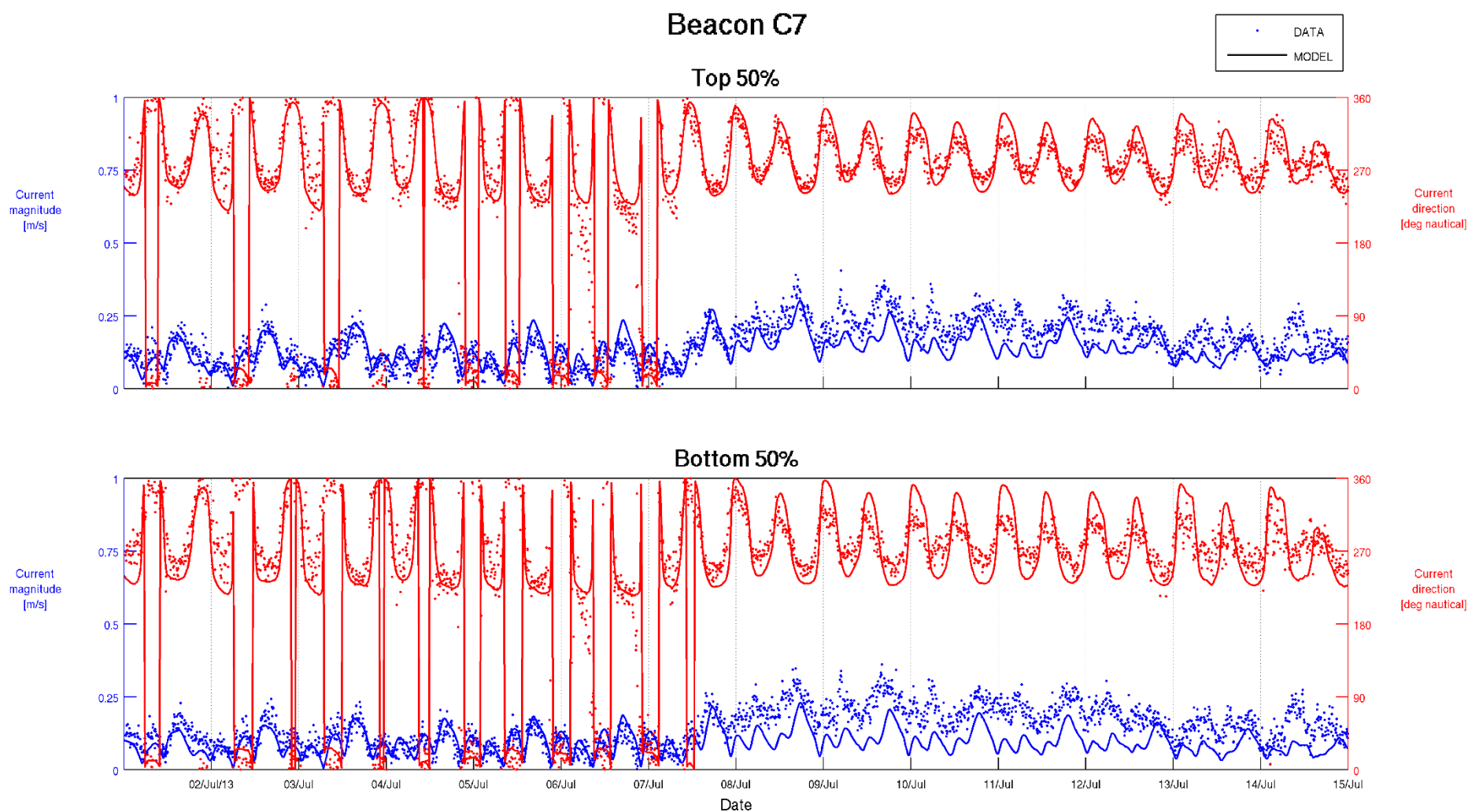
Figure F-9 Top 50% and Bottom 50% Current Validation – Beacon C7 01/07/2013 to 15/07/2013
