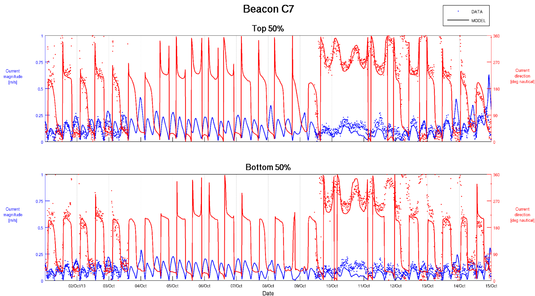
Figure F-15 Top 50% and Bottom 50% Current Validation – Beacon C7 01/10/2013 to 15/10/2013
