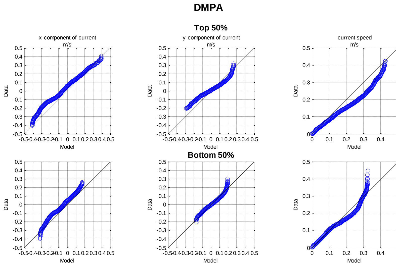
Figure H-1 Current Q-Q Plot – DMPA
