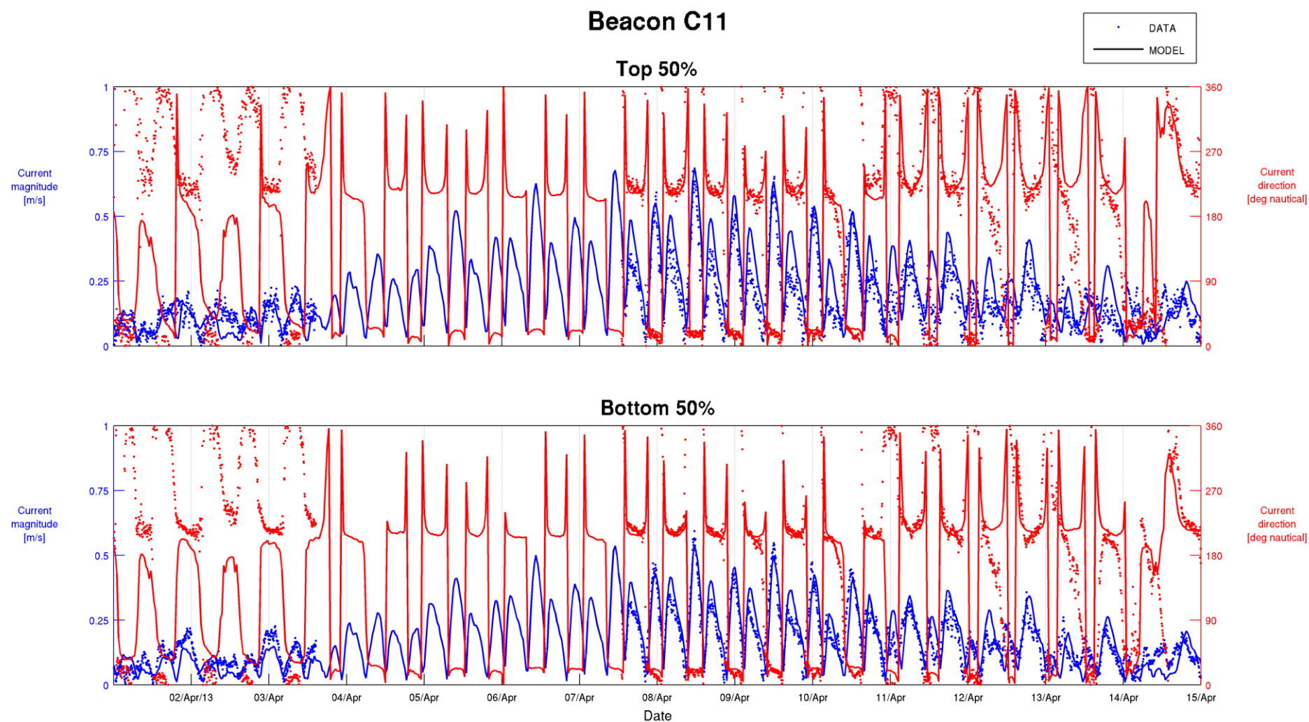
Figure C-24 Top 50% and Bottom 50% Current Calibration – Beacon C11 01/04/2013 to 15/04/2013
