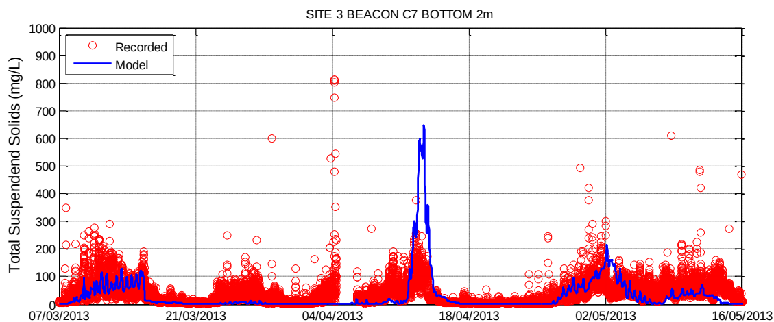
Figure 3-40 Sediment Re-suspension Calibration – Beacon C7
