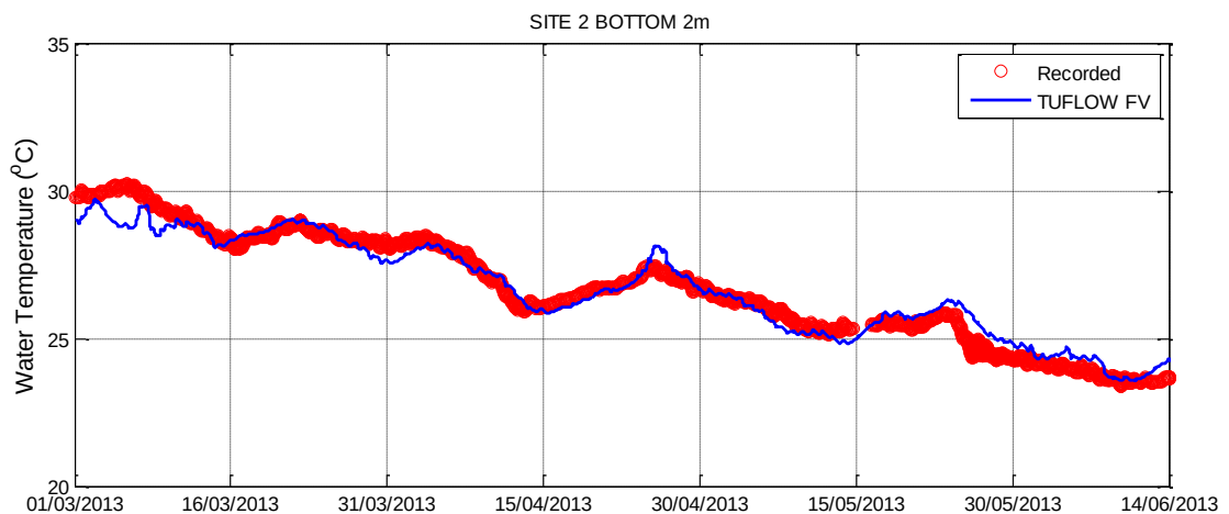
Figure 3-26 Hydrodynamic Model Calibration Near Bed Temperature – Site 2
