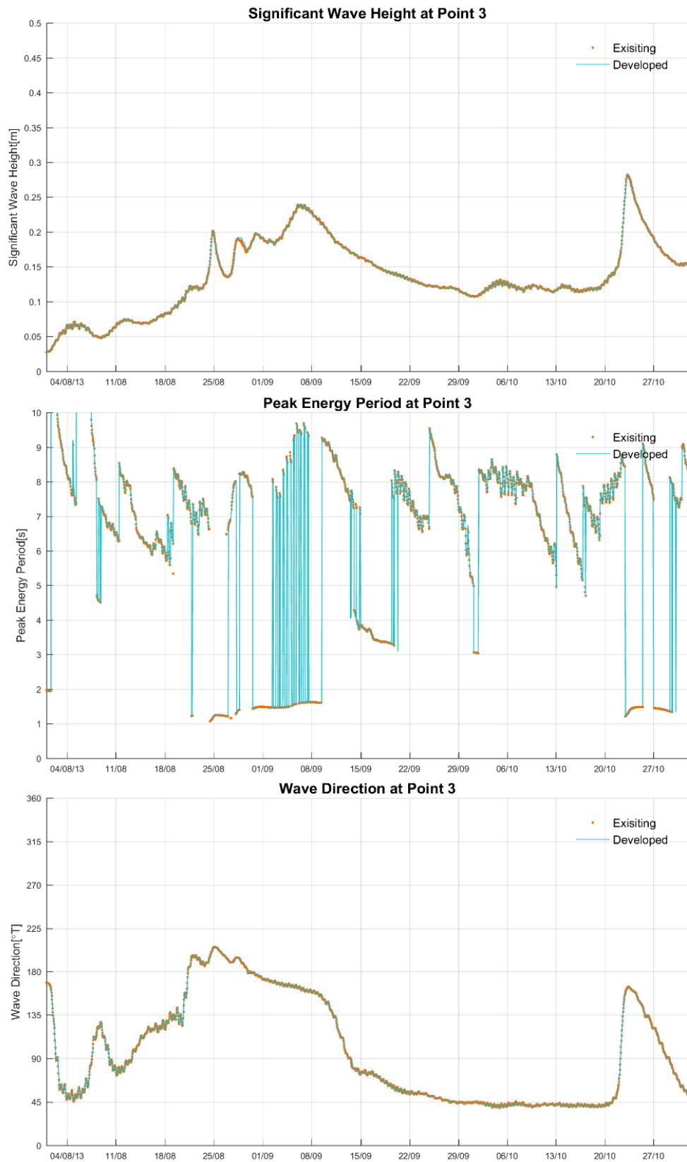
Figure 7-22 Base Case and Developed Case Wave Parameter Timeseries Comparison (Nearshore Location Point 3 in Figure 7-2)
