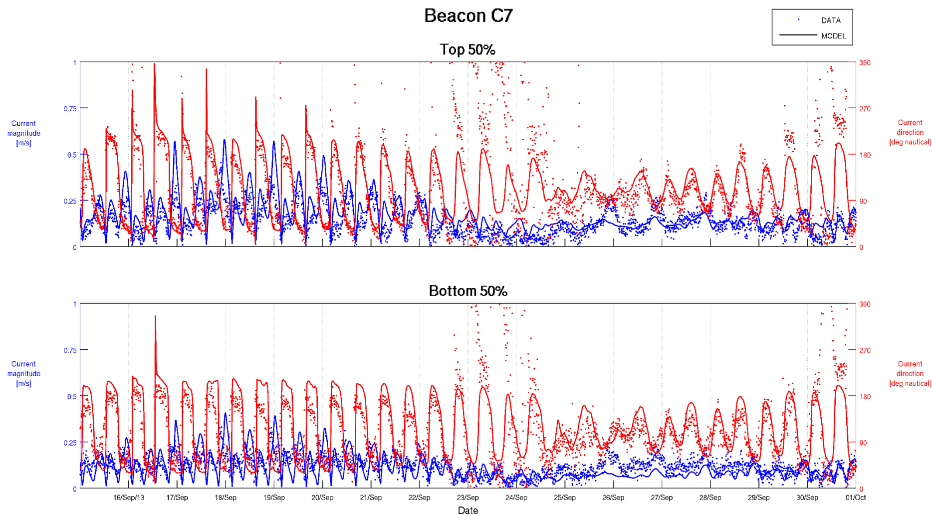
Figure F-14 Top 50% and Bottom 50% Current Validation – Beacon C7 15/09/2013 to 01/10/2013
