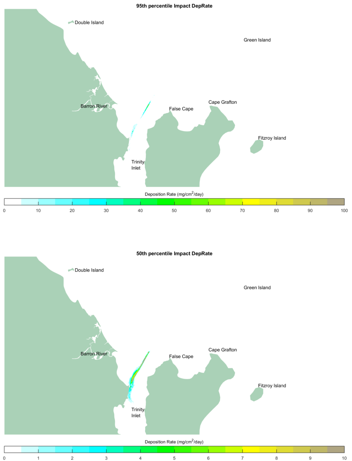
Figure 6-8 Likely Best Case Impact to Sediment Deposition Rate; 95 th Percentile (Top), 50 th Percentile (Bottom)
