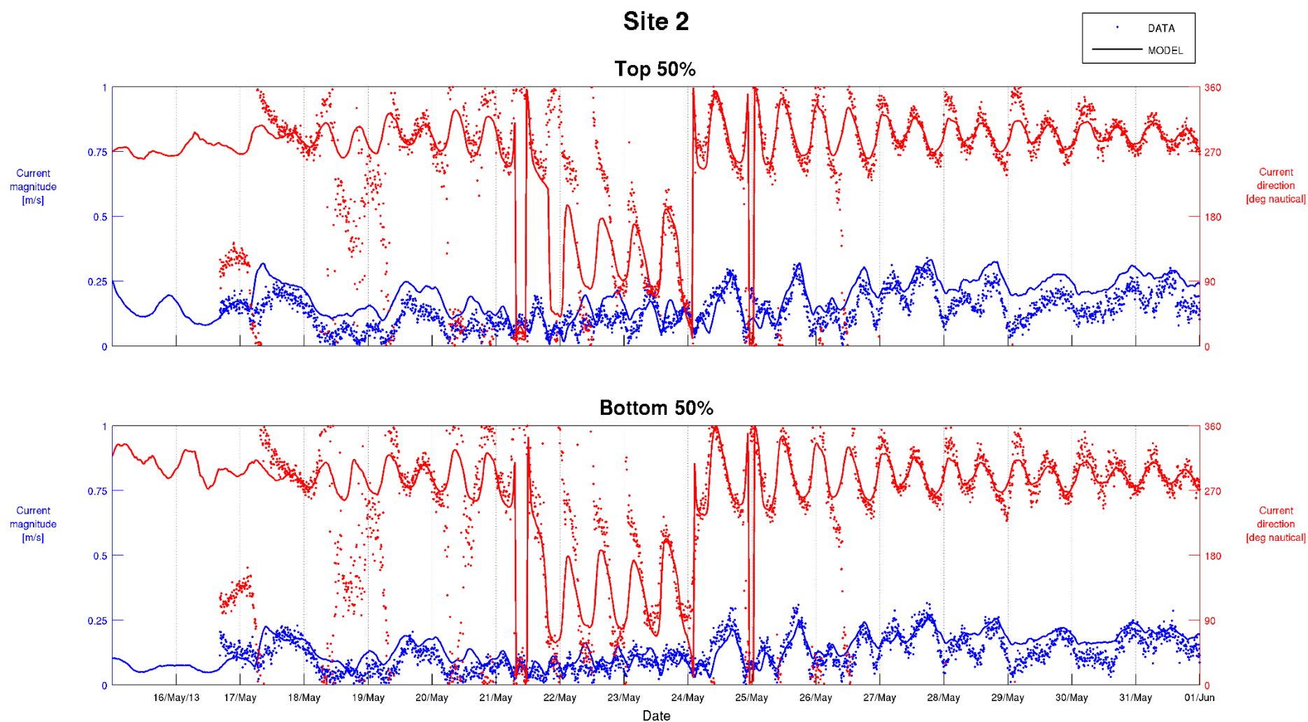
Figure C-13 Top 50% and Bottom 50% Current Calibration – Site 2 15/05/2013 to 01/06/2013
