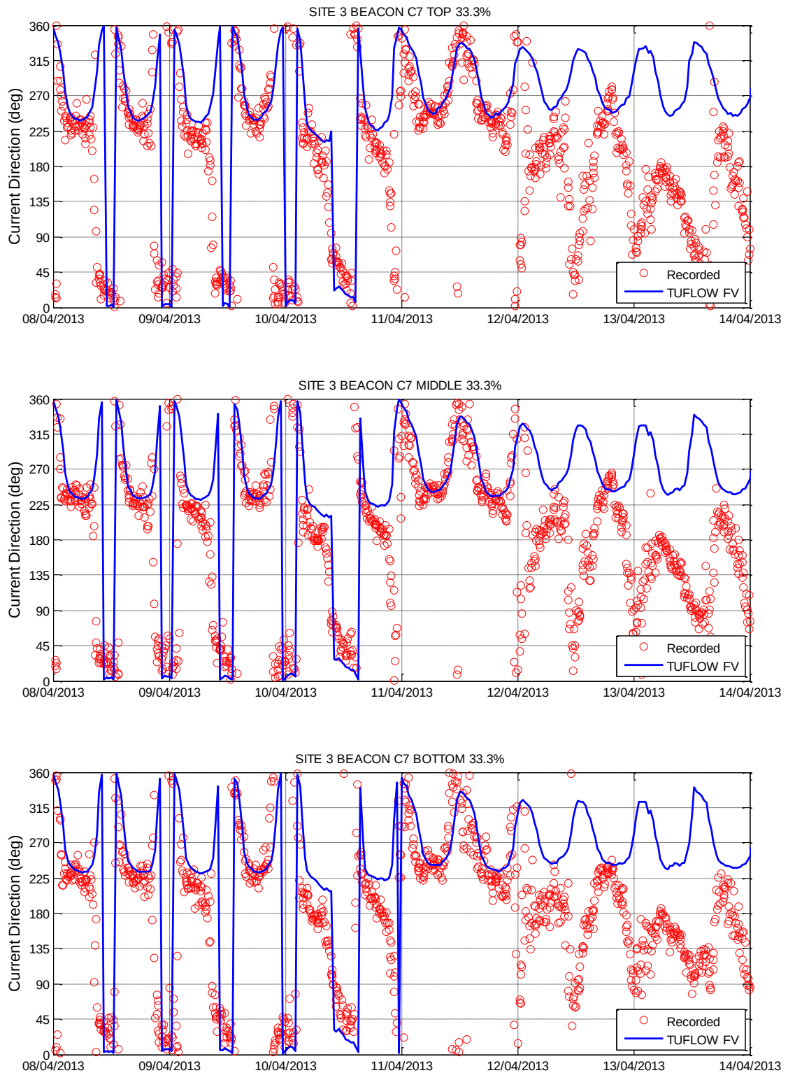
Figure 3-19 Hydrodynamic Model Calibration Current Direction Layers – Site 3 Beacon C7
