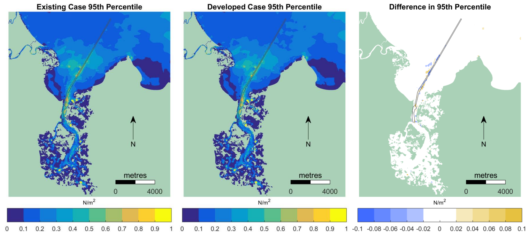
Figure 7-14 Modelled 95%ile Current Related Bed Shear Stress ( N/m^2 ) and Impacts. Existing case (left); Developed case (middle) and Impacts (right)
