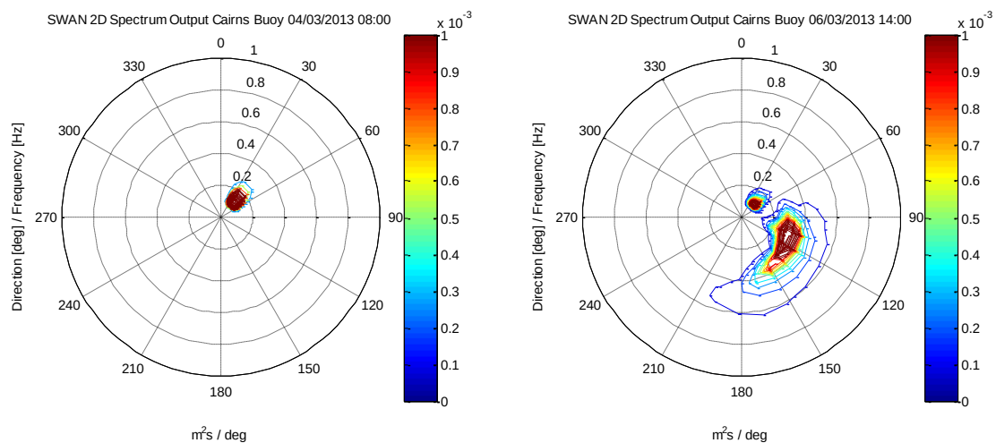
Figure 3-29 Example Wave Energy Spectrum showing Dominant Swell (left) and Wind Generated Sea (right) States
