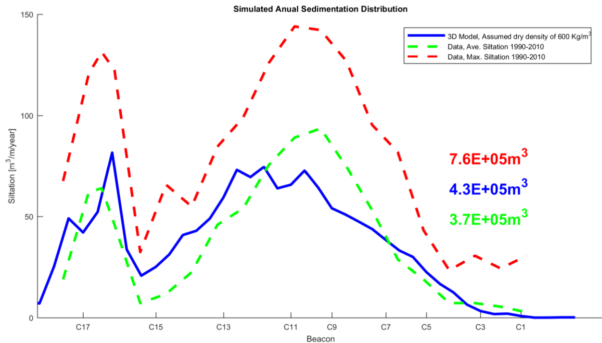
Figure 5-28 Estimated and Measured Annual Siltation of Shipping Channel
