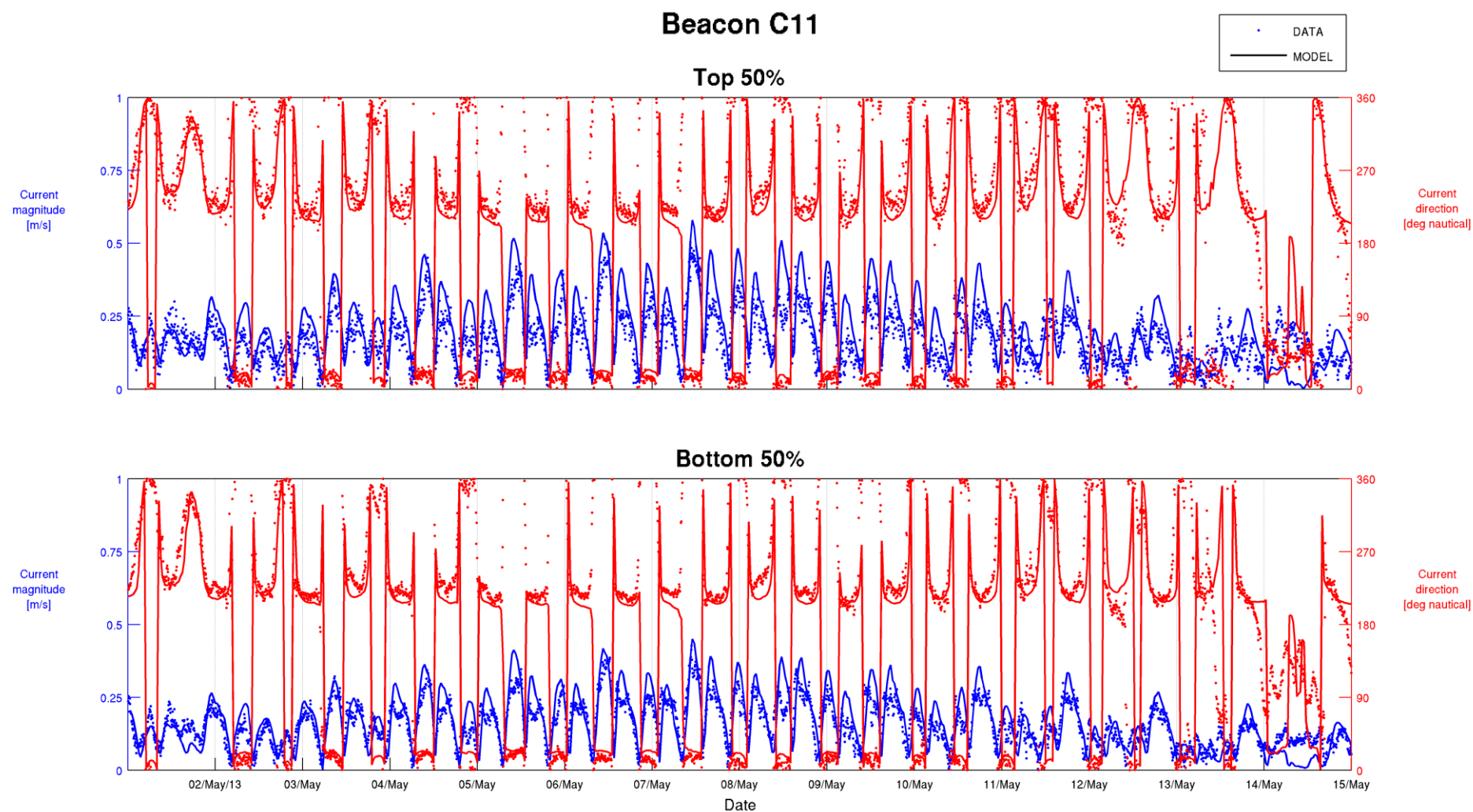
Figure C-26 Top 50% and Bottom 50% Current Calibration – Beacon C11 01/05/2013 to 15/05/2013
