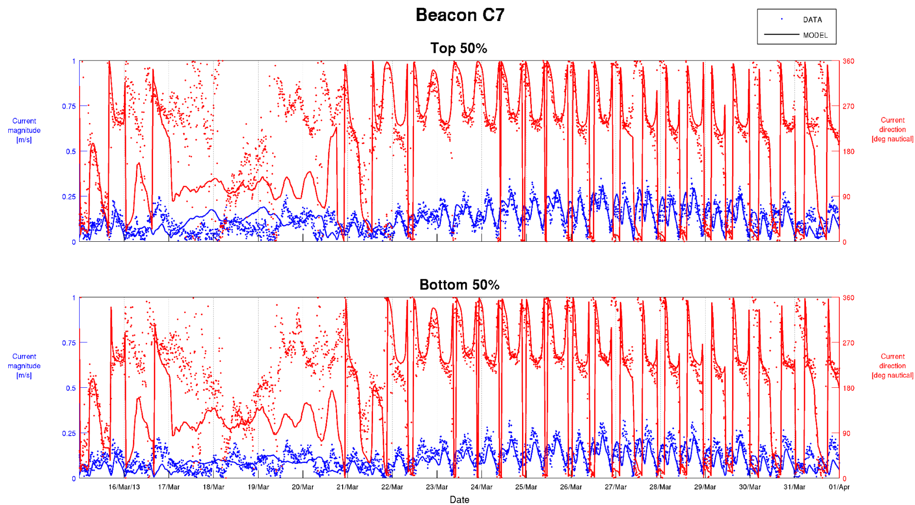
Figure C-16 Top 50% and Bottom 50% Current Calibration – Beacon C7 15/03/2013 to 01/04/2013
