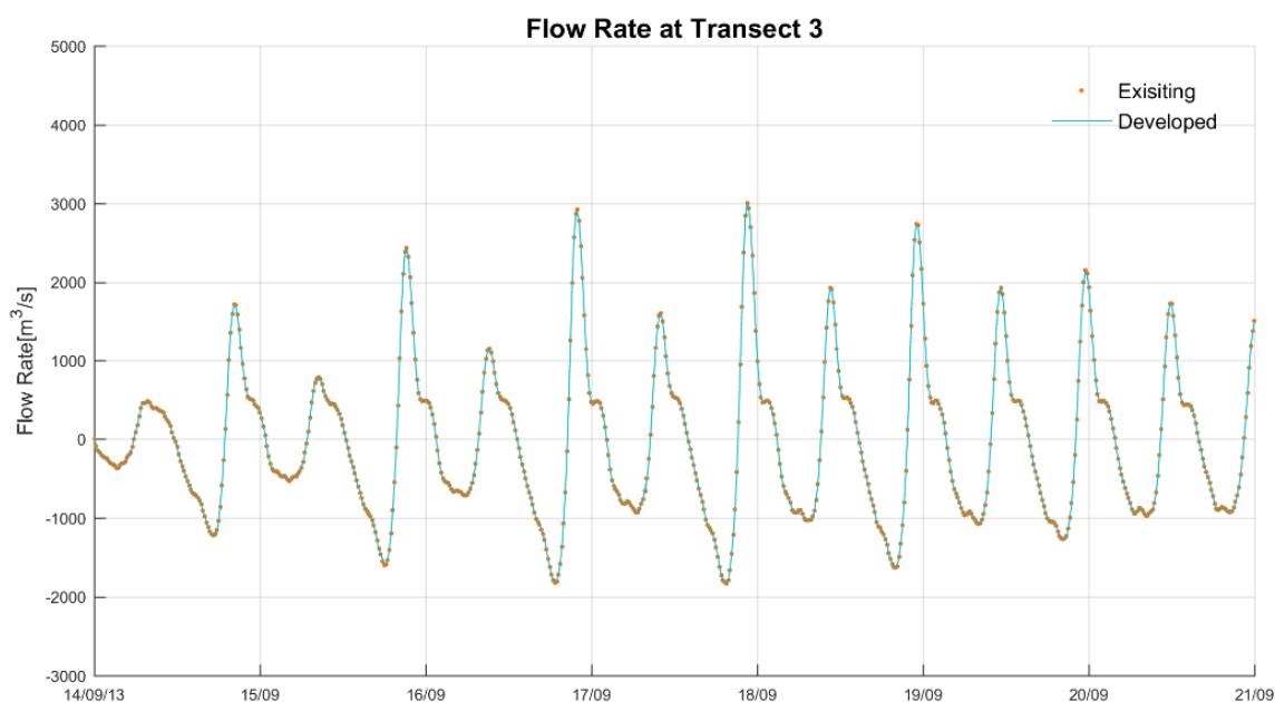
Figure 7-13 Existing and Developed Case Flow Timeseries at Transect 3 (shown in Figure 7-2)
