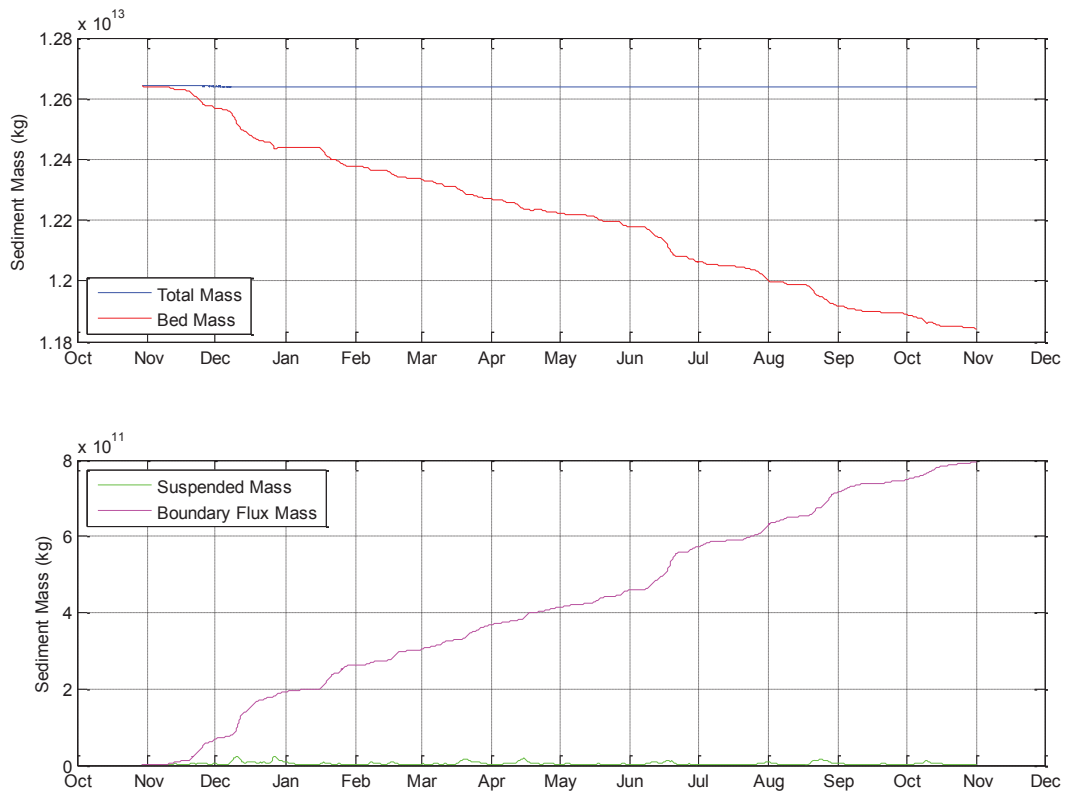
Figure 3. Sediment Mass Balance Checks - Re-suspension Period
