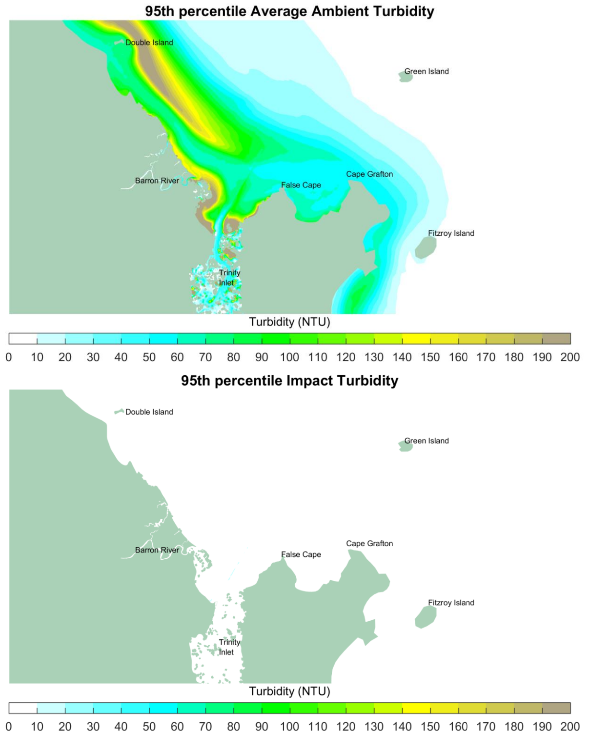
Figure K-2 Likely Best Case 95 th percentile: average ambient (Top), impact of dredging (Bottom)
