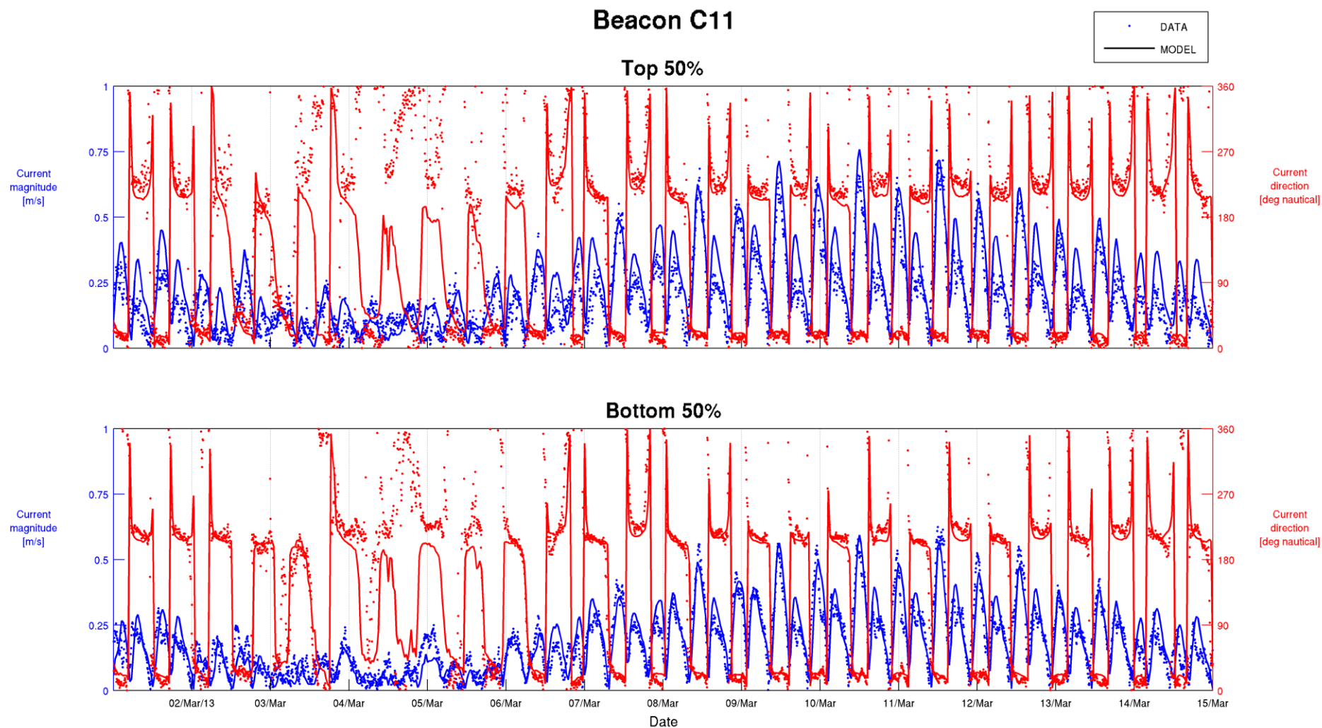
Figure C-22 Top 50% and Bottom 50% Current Calibration – Beacon C11 01/03/2013 to 15/03/2013
