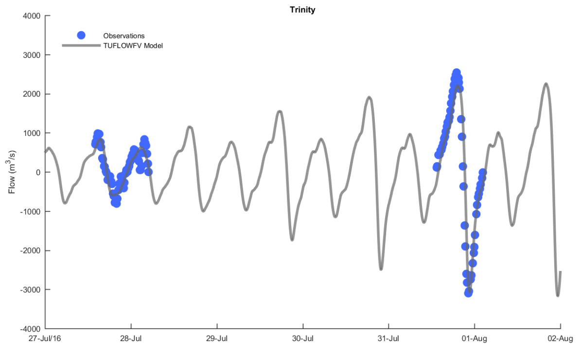
Figure 5-18 Trinity Inlet Flow Comparisons
