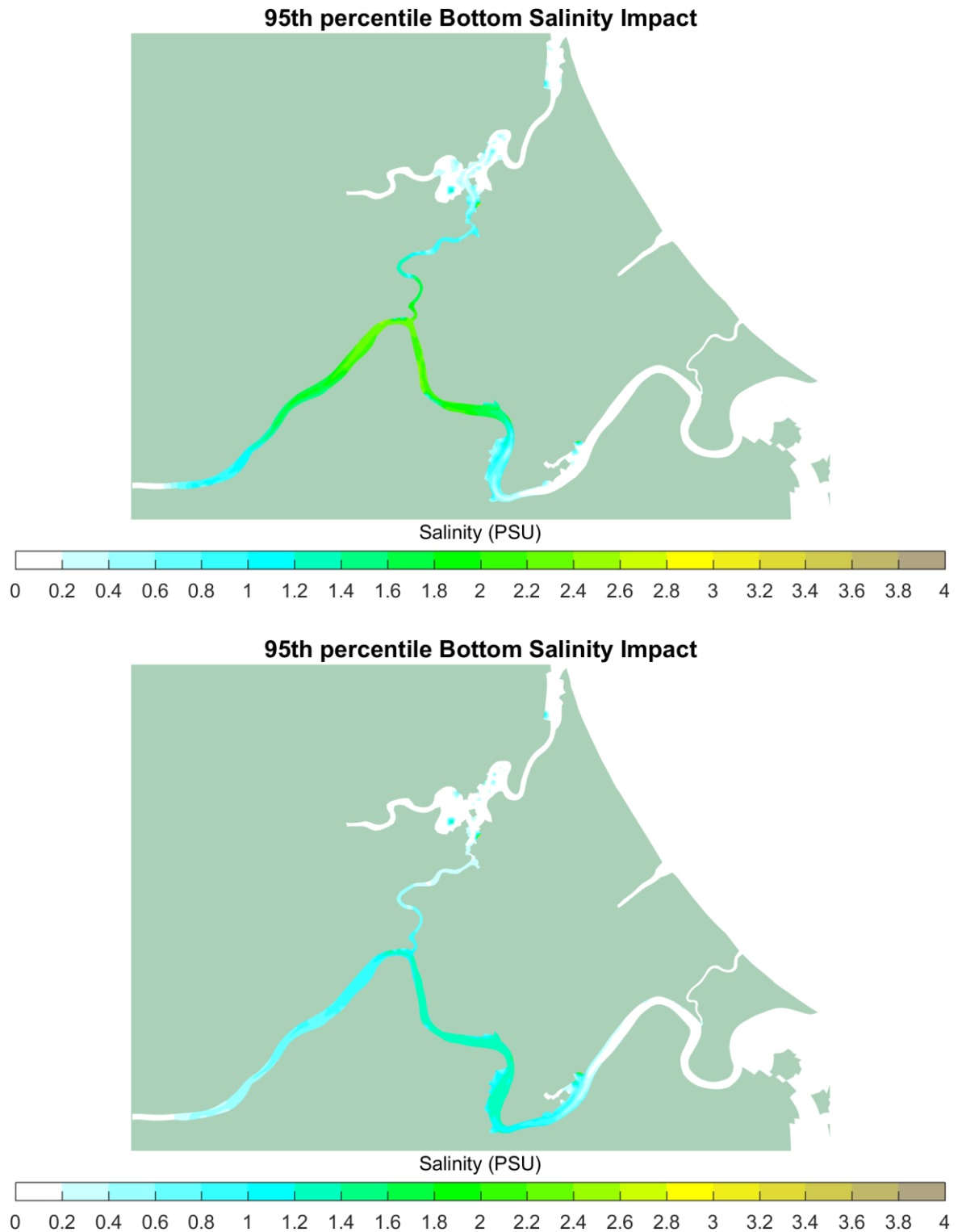
Figure 6-11 Impact to 95 th Percentile Bottom Salinity: Site 1 (Top), Site 2 (Bottom)
