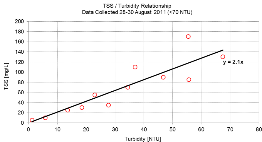
Figure 4-1 TSS-NTU Relationship August 2011 Dredge Plume Monitoring
