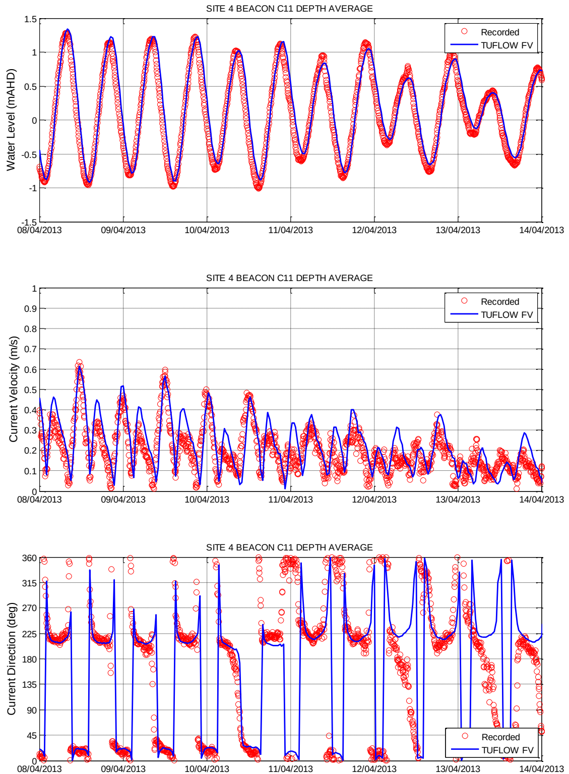
Figure 3-21 Hydrodynamic Model Calibration 3D Depth Average – Site 4 Beacon C11
