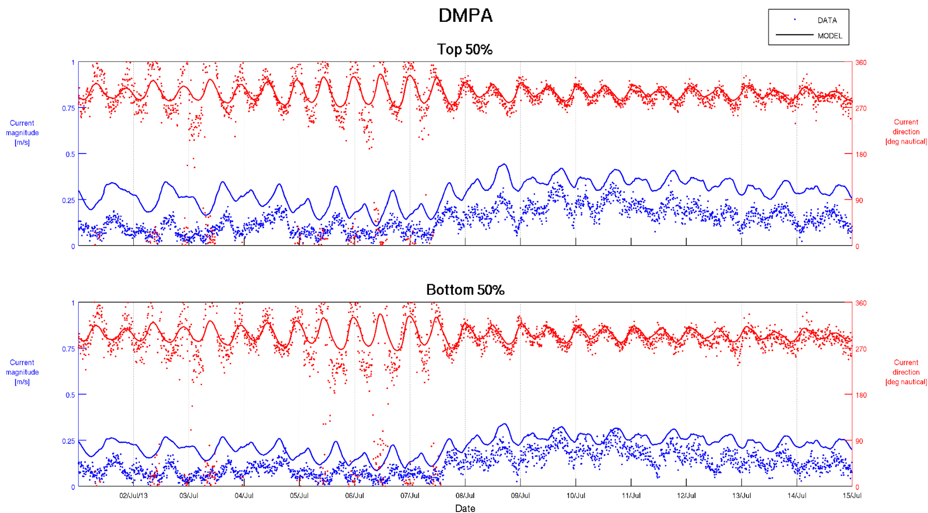
Figure F-2 Top 50% and Bottom 50% Current Validation – DMPA 01/07/2013 to 15/07/2013
