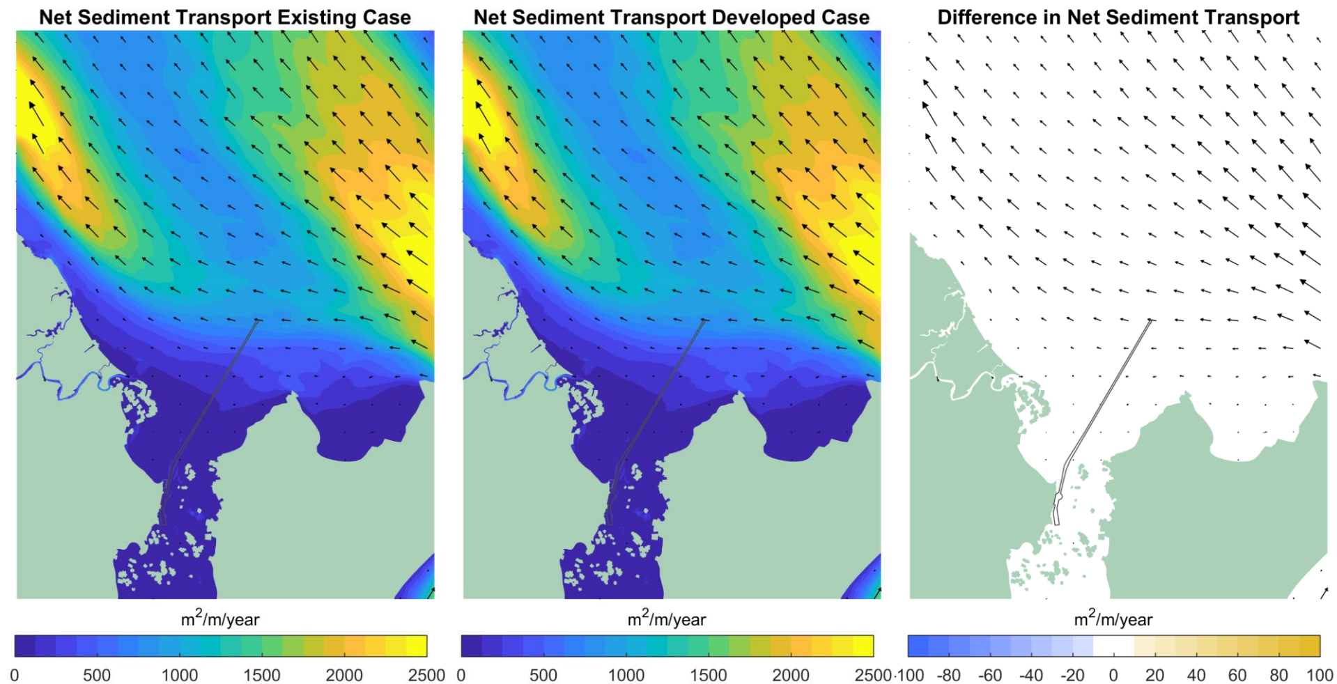
Figure 7-24 Modelled Net Sediment Transport (m 3 /m/year): Existing case (left); Developed case (middle) and Impacts (right)
