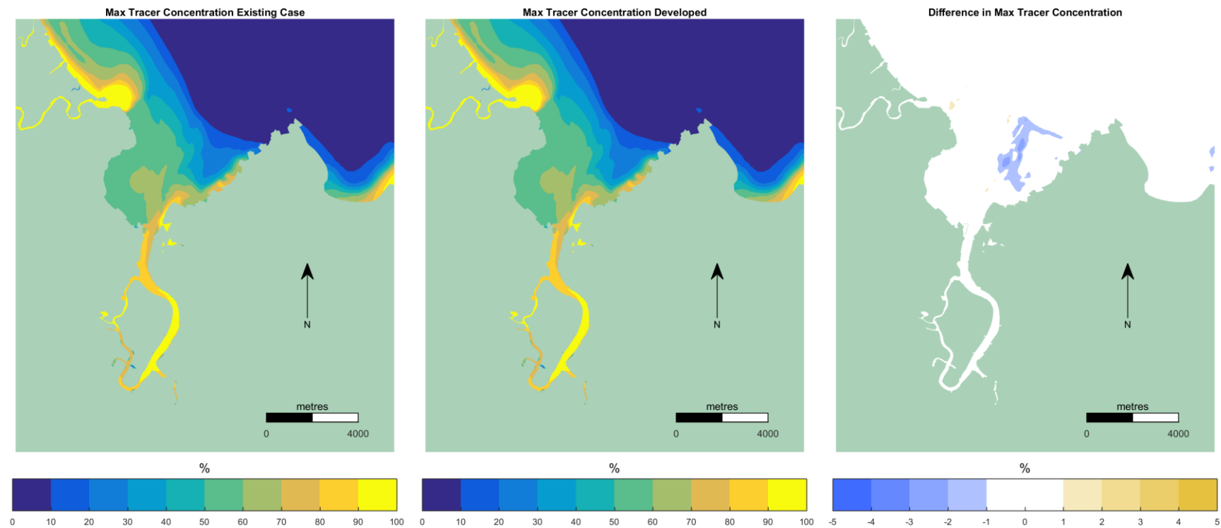
Figure 7-18 Modelled Flood Plume Tracer Concentration (%): Existing case (left); Developed case (middle) and Impacts (right)
