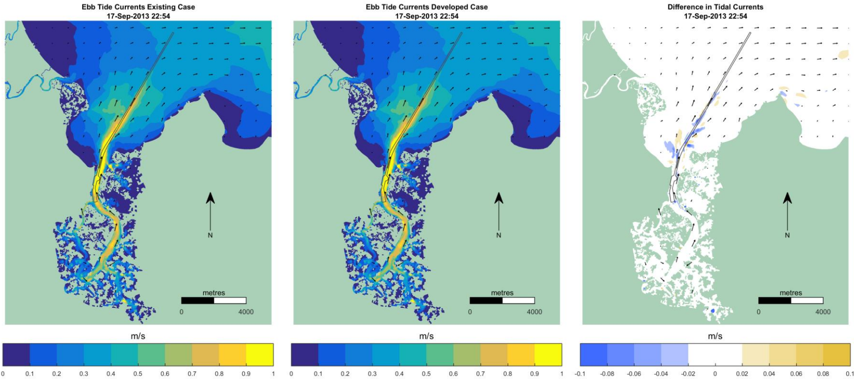
Figure 7-5 Modelled Spring Tide Ebb Currents and Impacts. Existing case (left); Developed case (middle) and Impacts (right)
