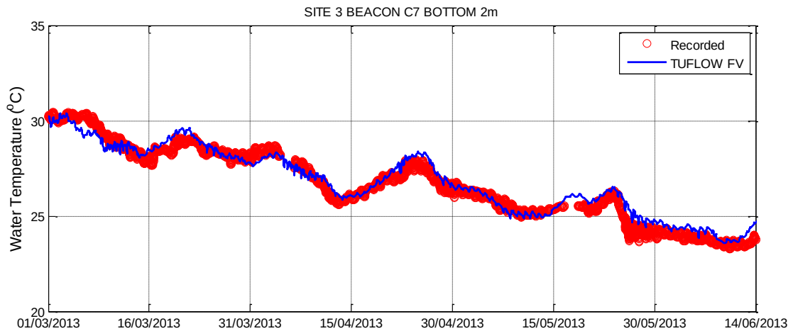
Figure 3-27 Hydrodynamic Model Calibration Near Bed Temperature – Site 3 Beacon C7
