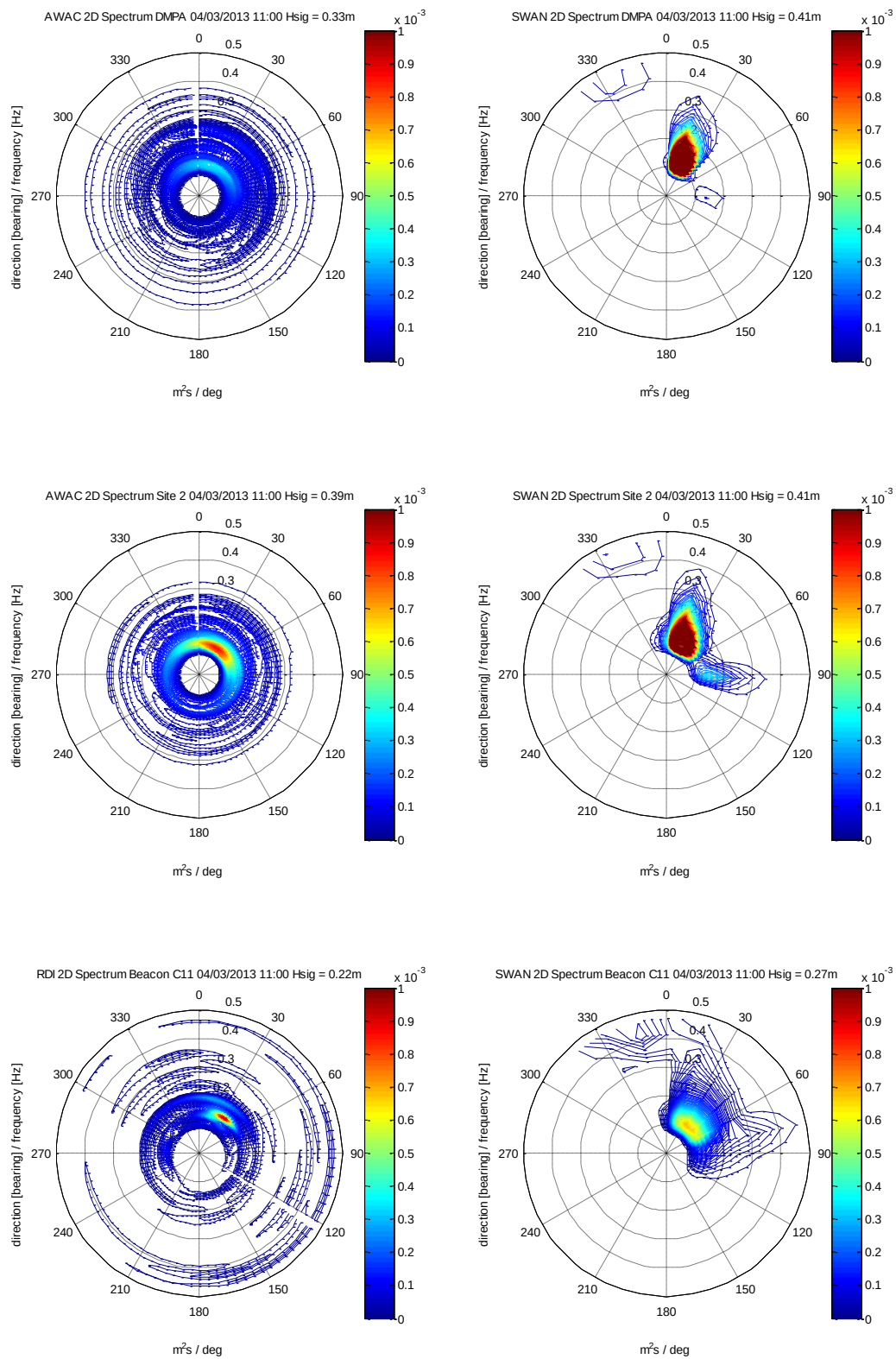
Figure 3-35 Recorded (left) and Predicted (right) 2D Wave Energy Spectrum: Dominant Swell State
