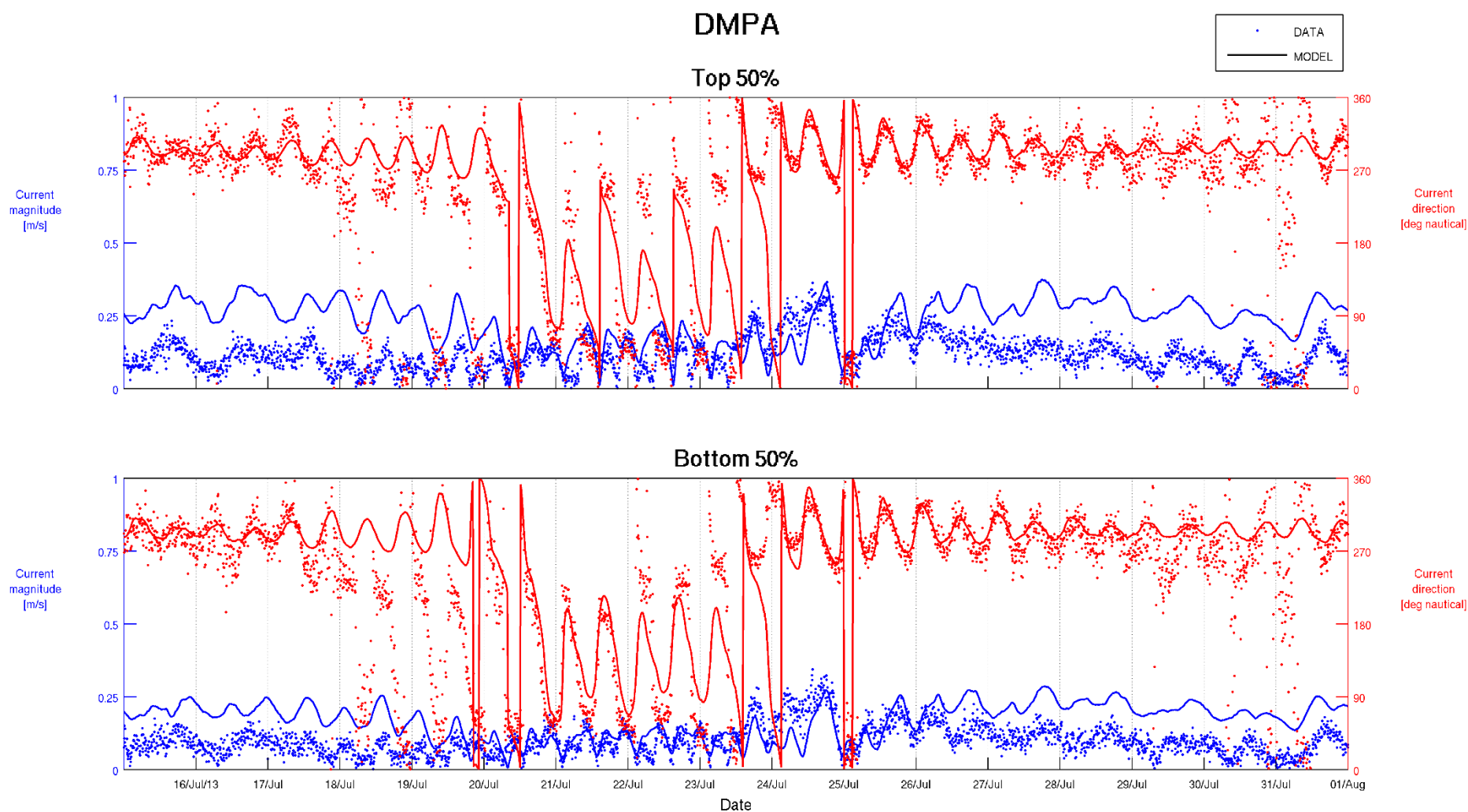
Figure F-3 Top 50% and Bottom 50% Current Validation – DMPA 16/07/2013 to 01/08/2013
