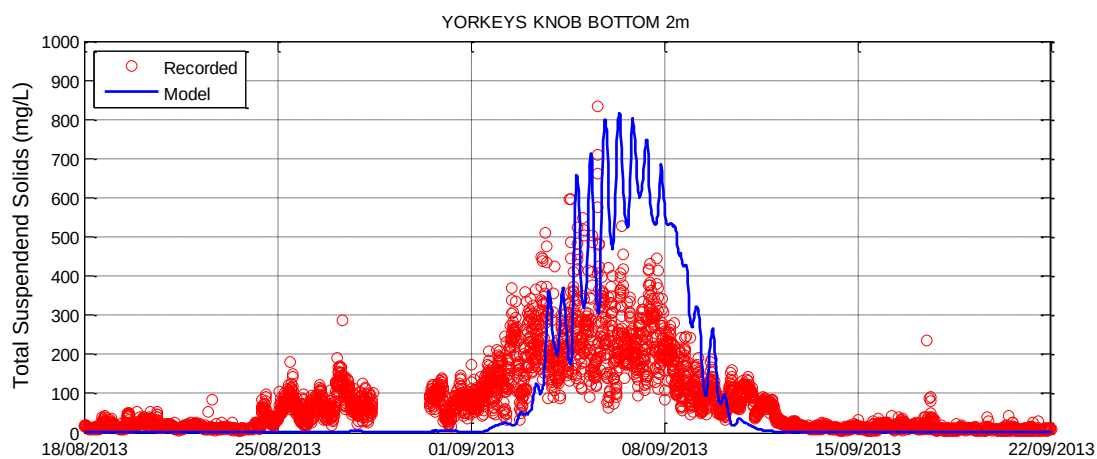
Figure 5-25 Sediment Re-suspension Validation – Yorke's Knob
