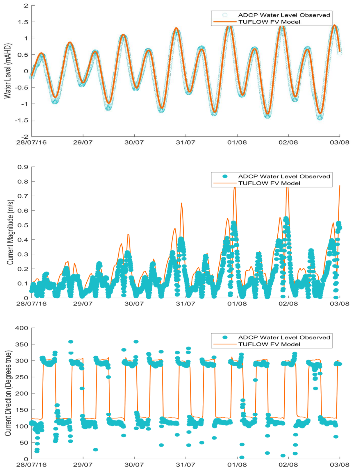
Figure 5-17 Trinity Inlet Validation: Water Level (Top), Current Magnitude (Middle), Current Direction (Bottom)
