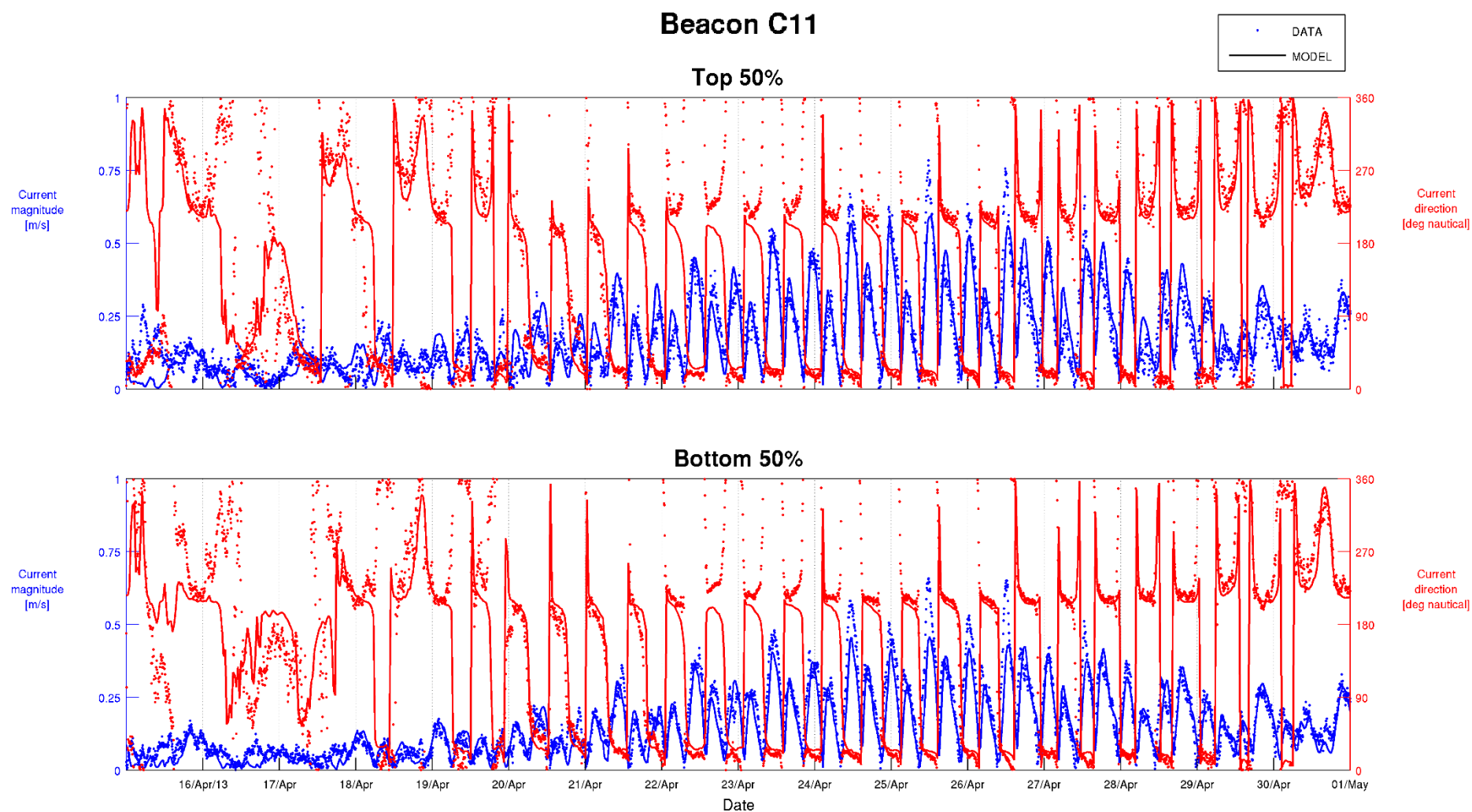
Figure C-25 Top 50% and Bottom 50% Current Calibration – Beacon C11 15/04/2013 to 01/05/2013
