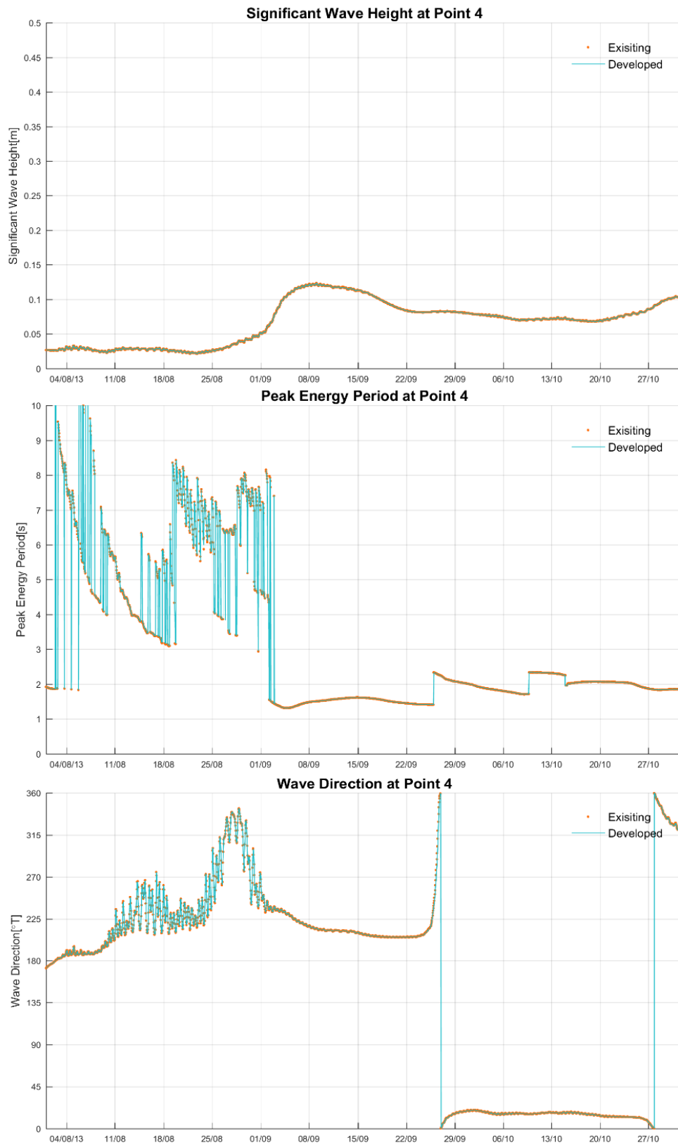
Figure 7-23 Base Case and Developed Case Wave Parameter Timeseries Comparison (Nearshore Location Point 4 in Figure 7-2)
