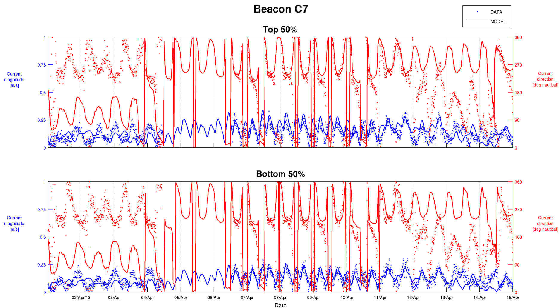
Figure C-17 Top 50% and Bottom 50% Current Calibration – Beacon C7 01/04/2013 to 15/04/2013
