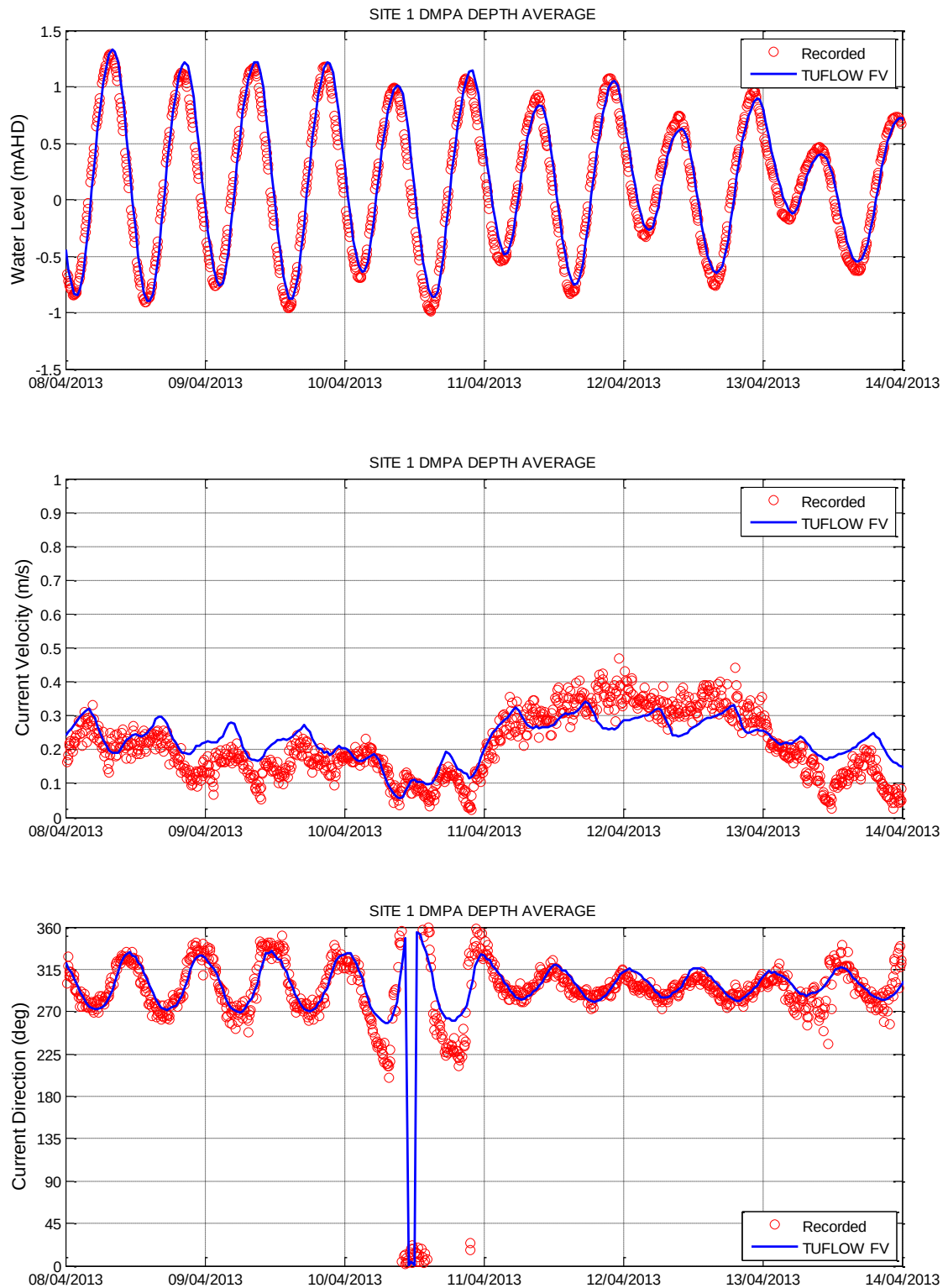
Figure 3-9 Hydrodynamic Model Calibration 3D Depth Average – Site 1 DMPA
