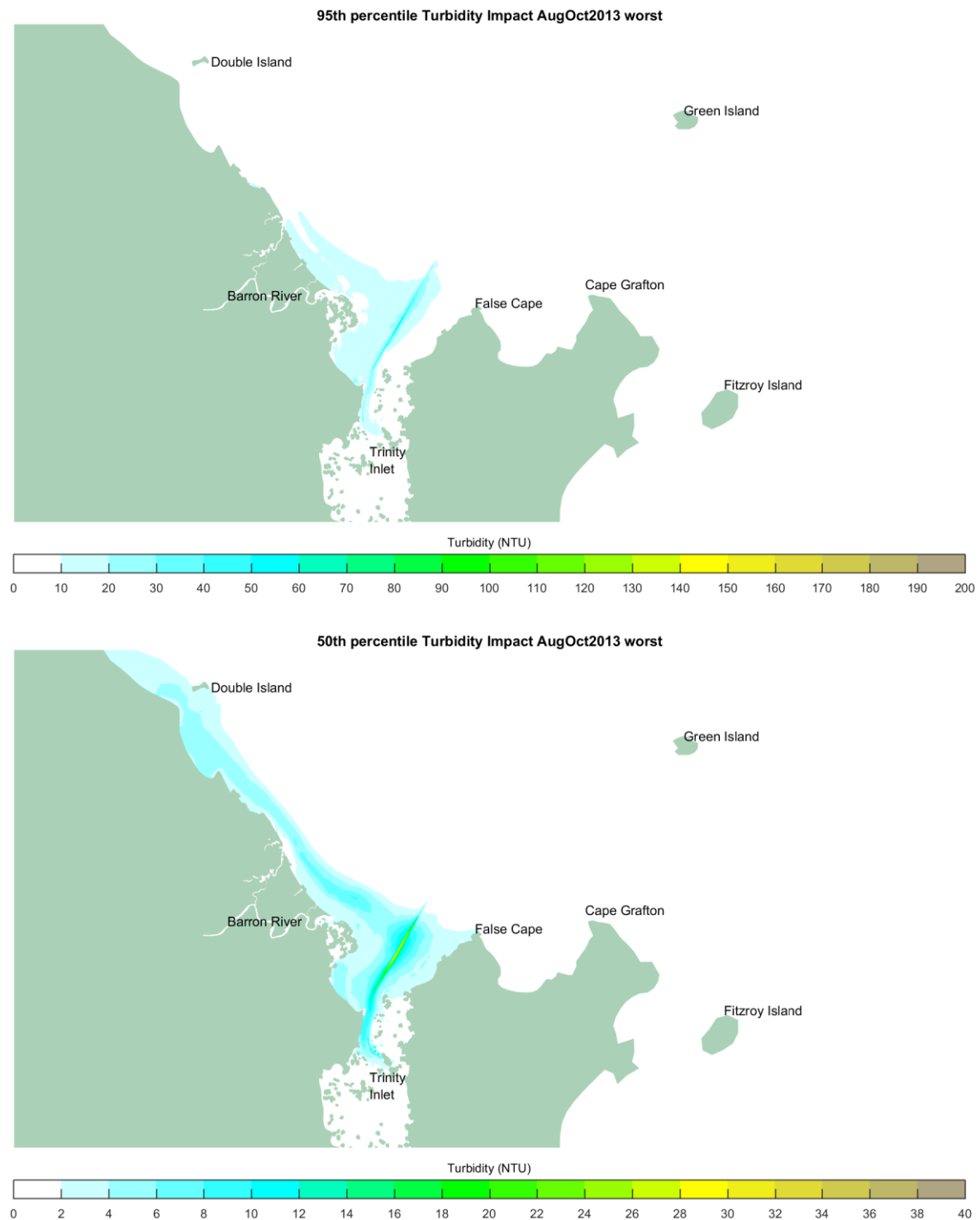
Figure J-4 Scenario 2 AugOct2013: 95 th Percentile (Top), 50 th Percentile (Bottom)
