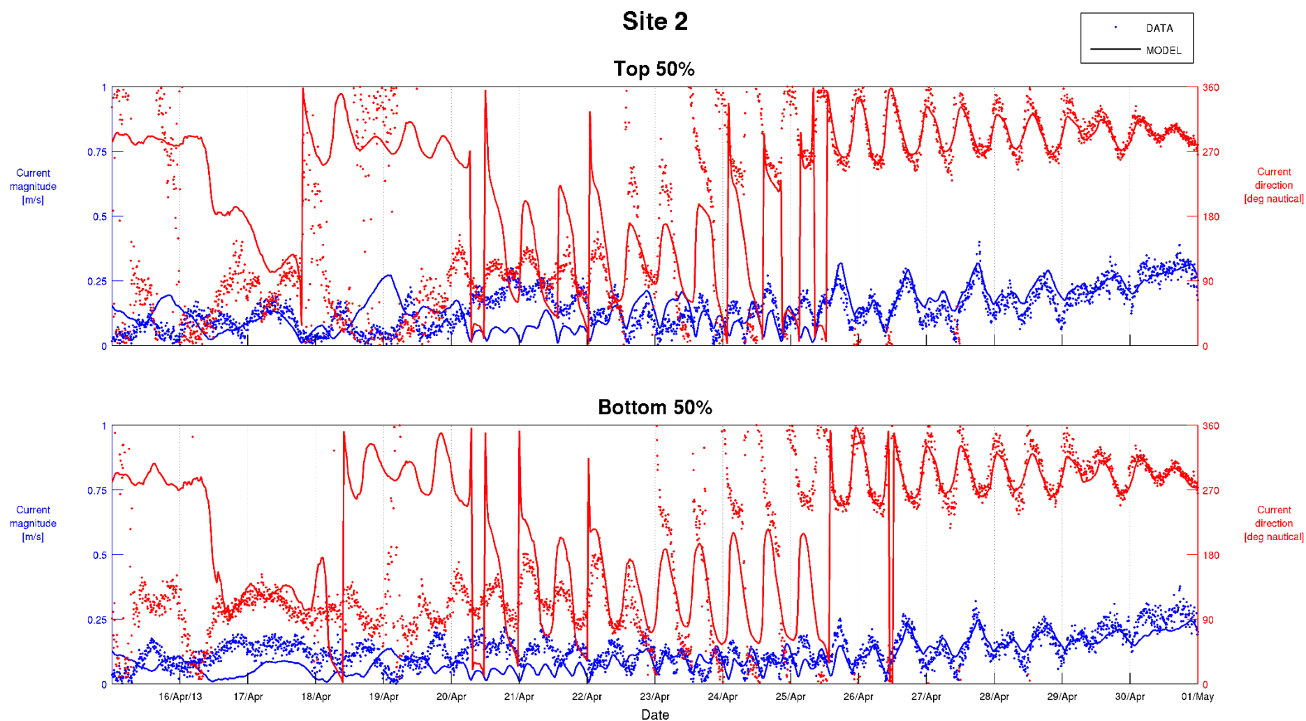
Figure C-11 Top 50% and Bottom 50% Current Calibration – Site 2 15/04/2013 to 01/05/2013
