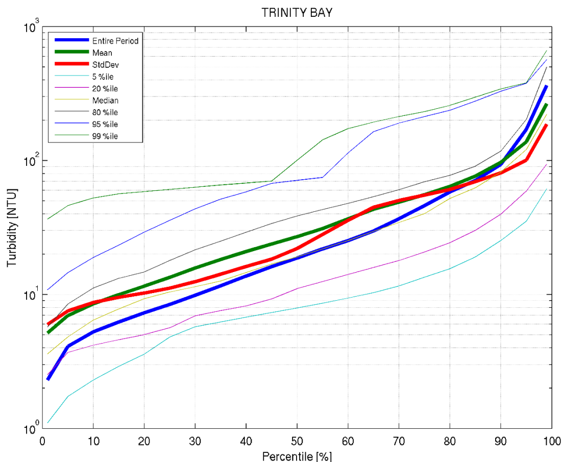
Figure 6-2 Trinity Bay Baseline Turbidity Statistics
