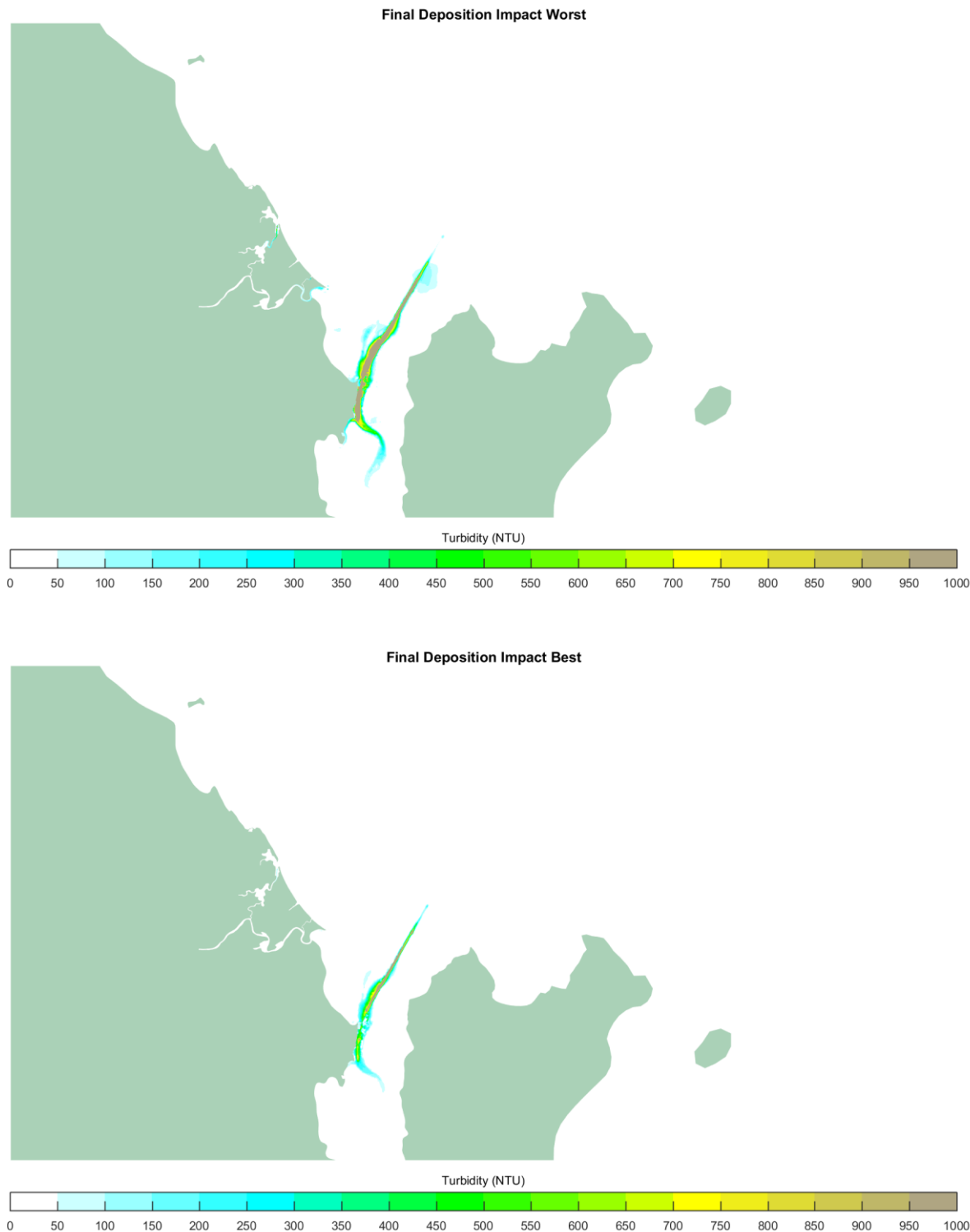
Figure 6-9 Capital Program Final Deposition: Worst (Top), Best (Bottom)
