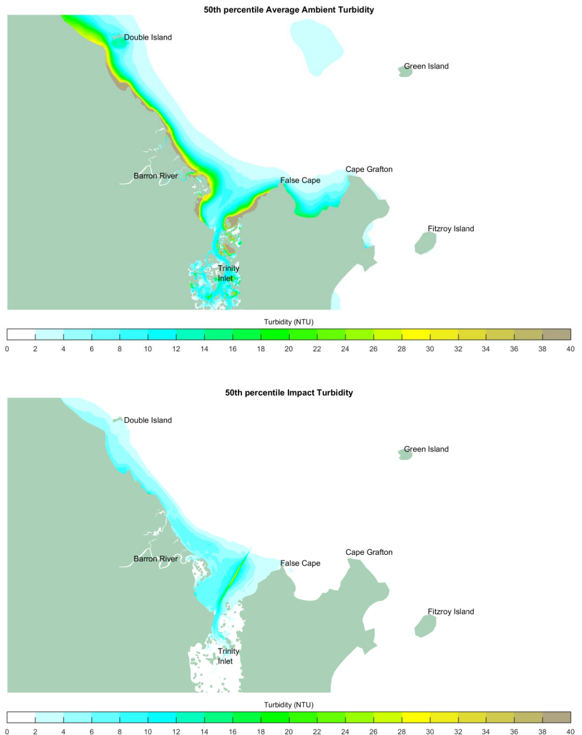
Figure 6-5 Likely Worst Case Capital Program 50 th Percentiles Turbidity; Average Ambient Turbidity (Top), Impact of Dredging (Bottom)
