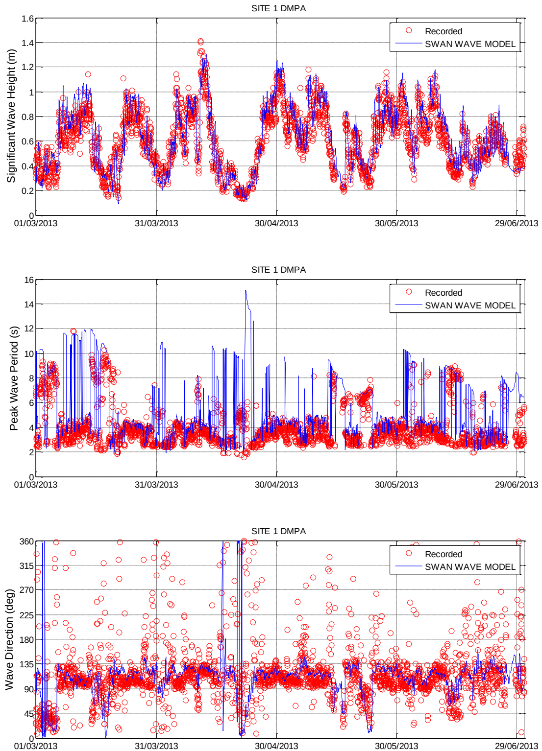
Figure 3-31 SWAN Wave Model Calibration – Site 1 DMPA
