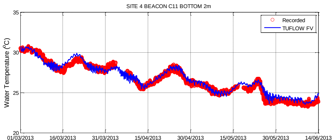
Figure 3-28 Hydrodynamic Model Calibration Near Bed Temperature – Site 4 Beacon C11
