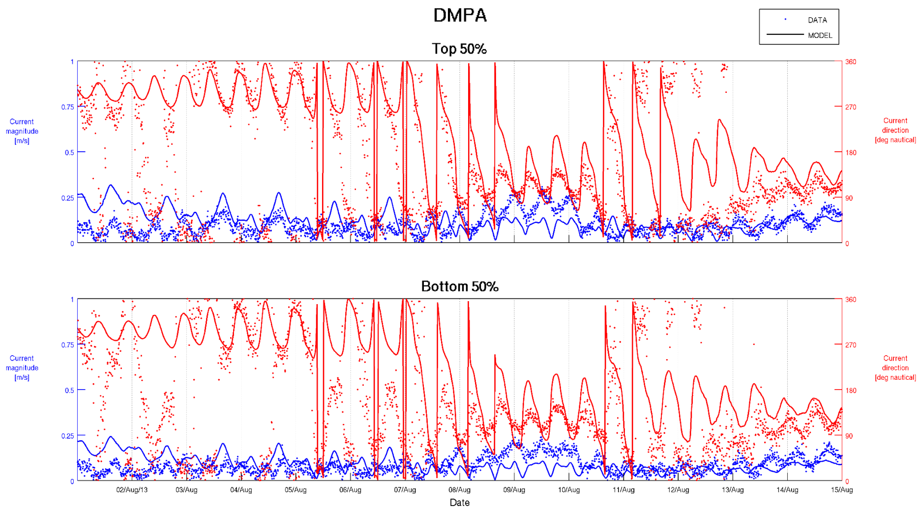
Figure F-4 Top 50% and Bottom 50% Current Validation – DMPA 01/08/2013 to 15/08/2013
