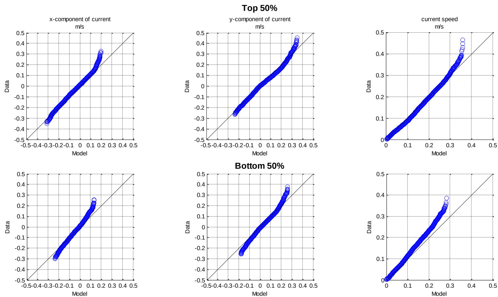
Figure E-3 Current Q-Q Plot – Beacon C7
