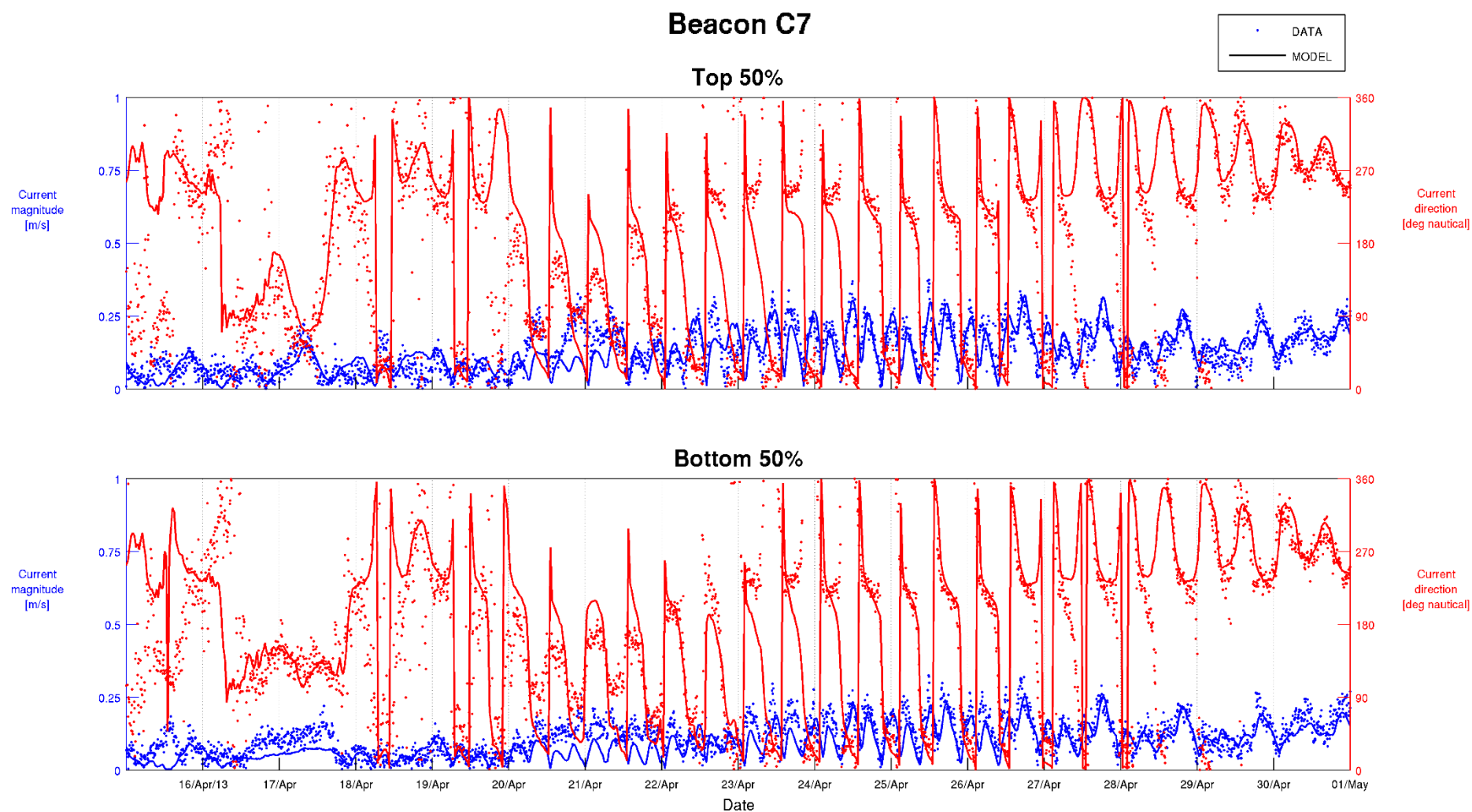
Figure C-18 Top 50% and Bottom 50% Current Calibration – Beacon C7 15/04/2013 to 01/05/2013
