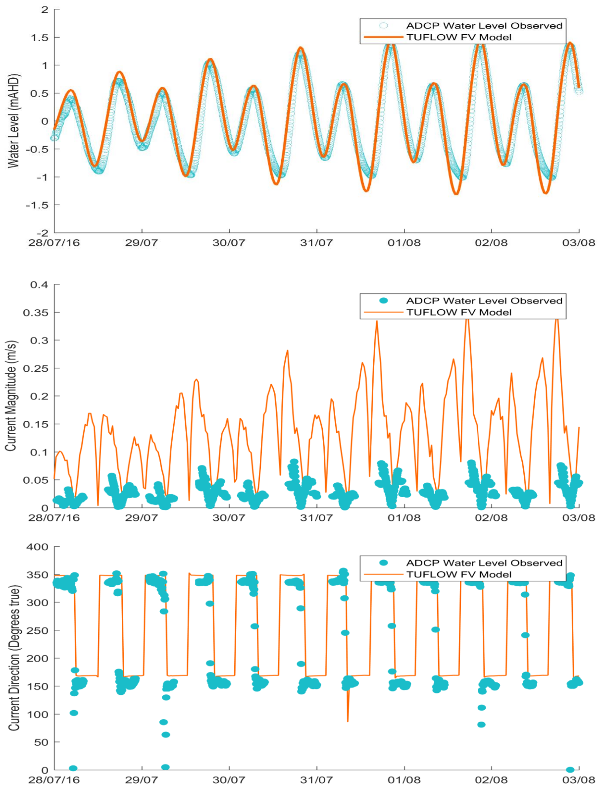
Figure 5-19 Barron River Validation: Water Level (Top), Current Magnitude (Middle), Current Direction (Bottom)
