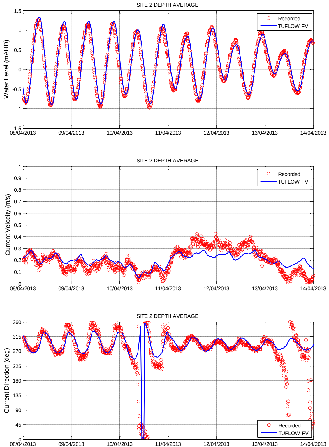
Figure 3-13 Hydrodynamic Model Calibration 3D Depth Average – Site 2
