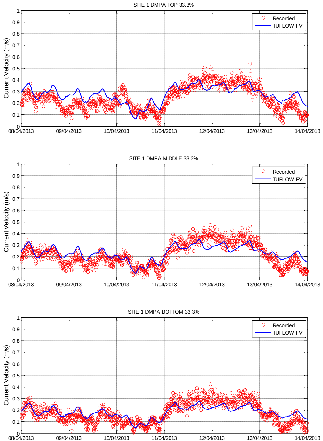
Figure 3-10 Hydrodynamic Model Calibration Current Velocity Layers – Site 1 DMPA
