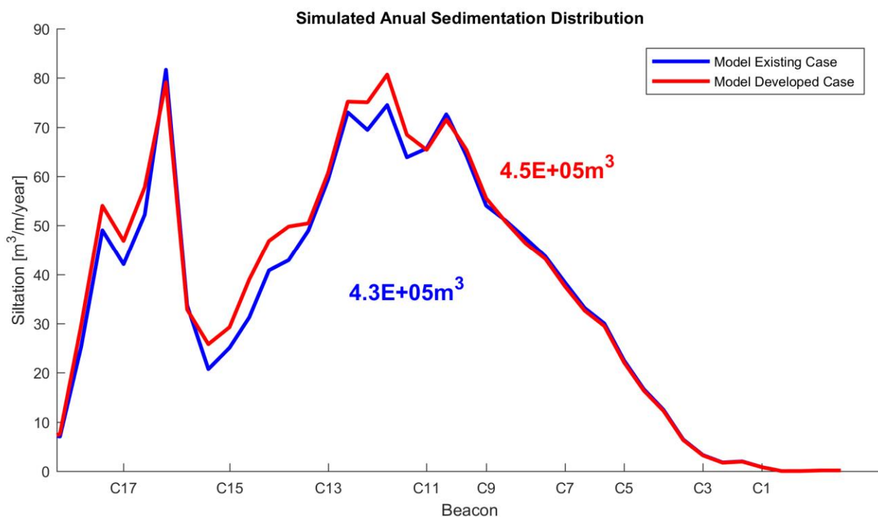
Figure 7-25 Modelled Existing Case and Developed Case Channel Siltation
