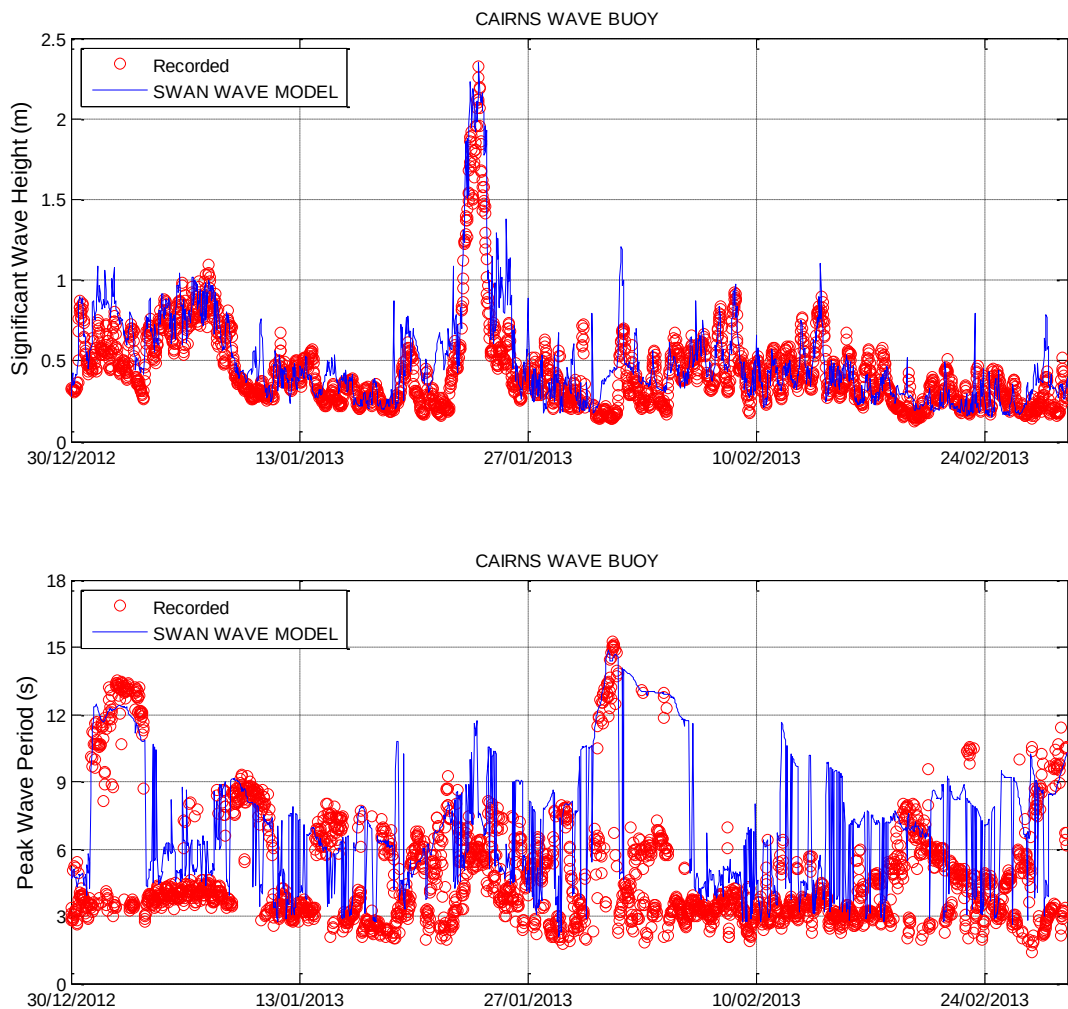
Figure 3-30 SWAN Wave Model Calibration – Cairns Wave Buoy
