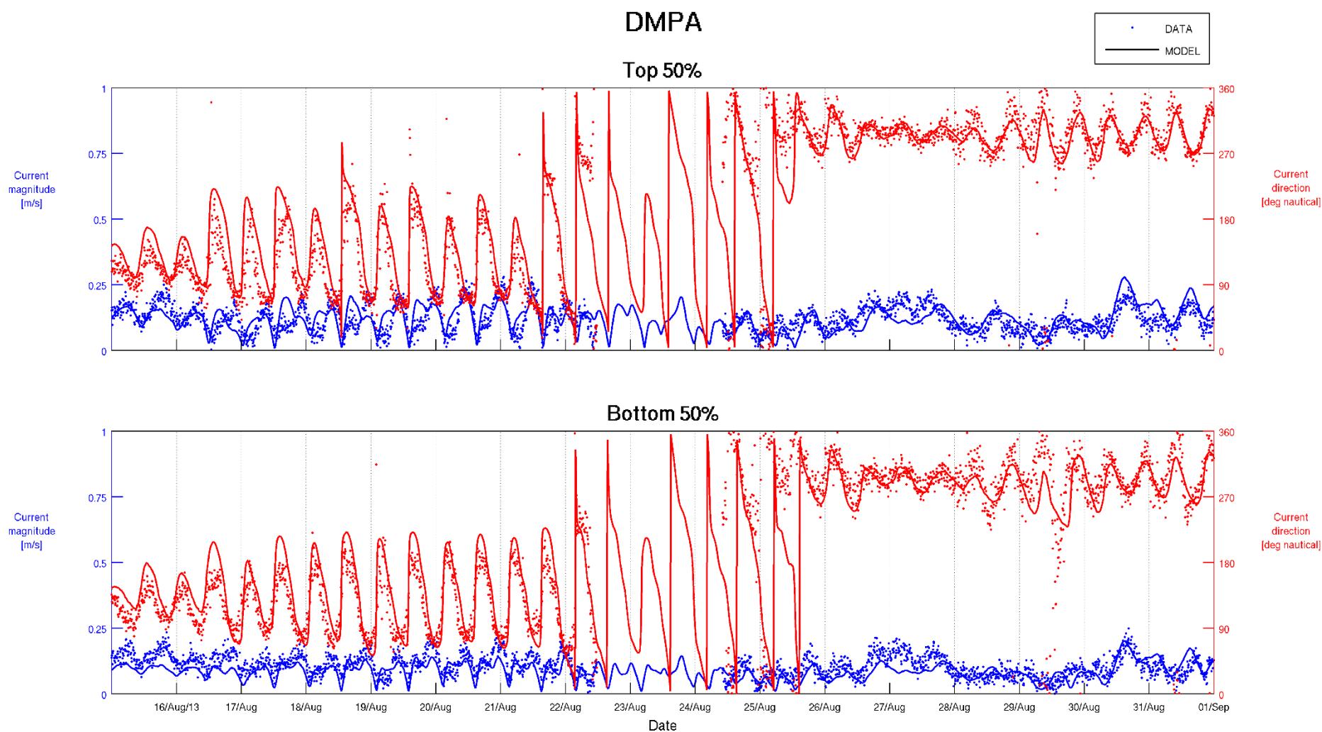
Figure F-5 Top 50% and Bottom 50% Current Validation – DMPA 15/08/2013 to 01/09/2013
