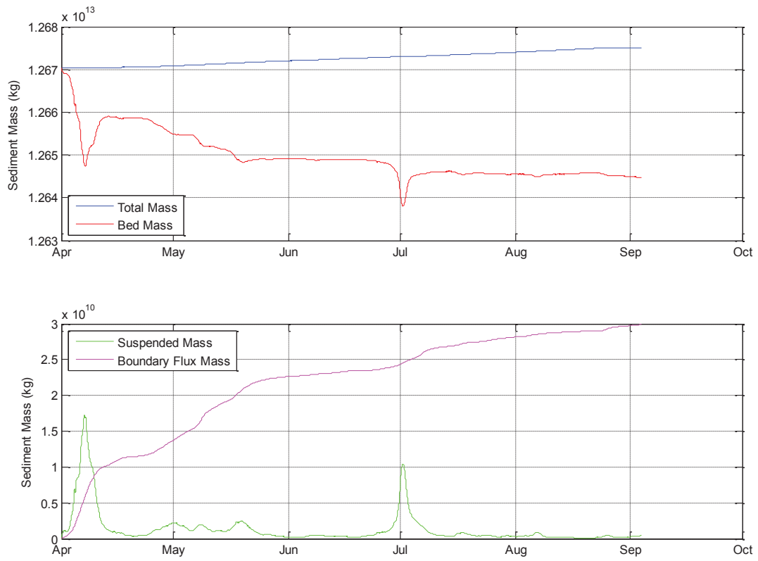
Figure 2. Sediment Mass Balance Checks - Capital Alternative Case
