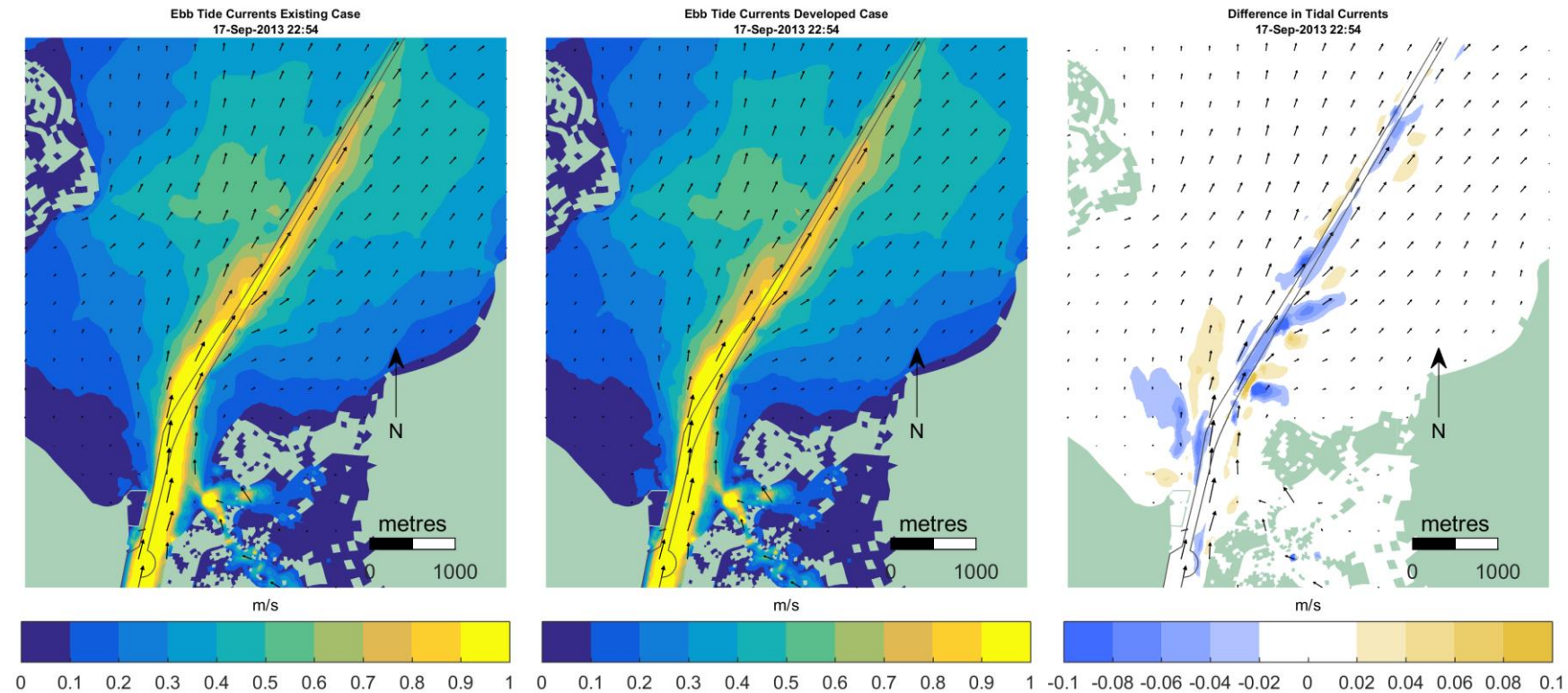
Figure 7-6 Modelled Spring Tide Ebb Currents and Impacts – zoomed. Existing case (left); Developed case (middle) and Impacts (right)
