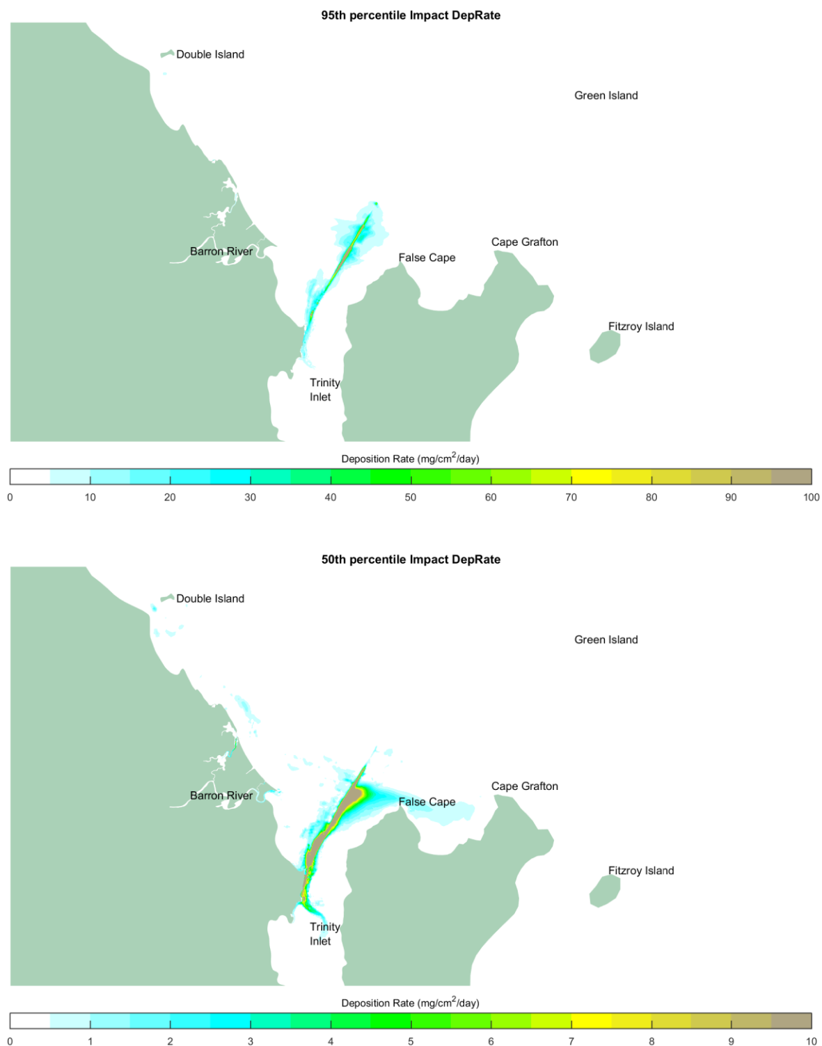
Figure 6-7 Likely Worst Case Impact to Sediment Deposition Rate; 95 th Percentile (Top), 50 th Percentile (Bottom)
