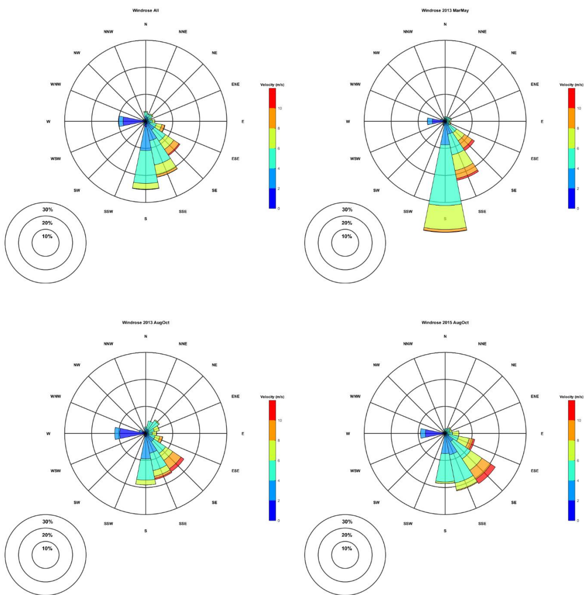
Figure 6-1 Cairns Aero Windroses: All March to October Data (Top Left), March – May 2013 (Top Right) August – October 2013 (Bottom Left), August – October 2015 (Bottom Right)
