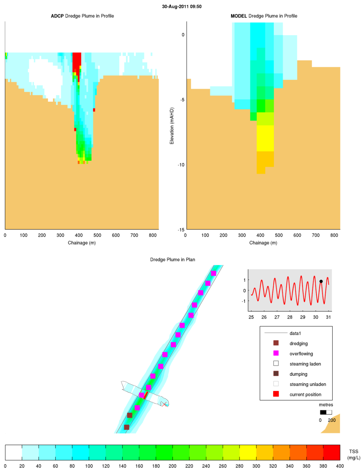
Figure 4-5 Maintenance Dredging Plume Validation, 30/08/2011 09:50: Recorded Plume (top left) and Modelled Plume (top right) Vertical Distribution; Recorded and Modelled Plume Plan View (bottom)
