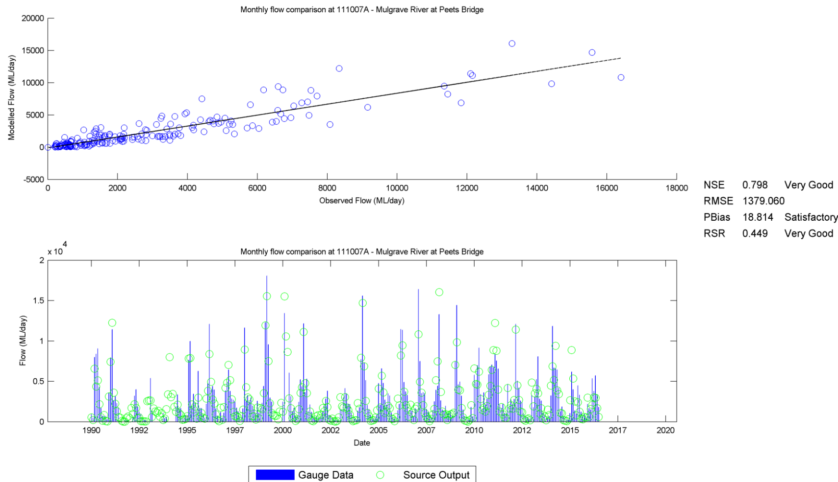
Figure 5-30 Catchment Model Comparison to Mulgrave River Gauge
