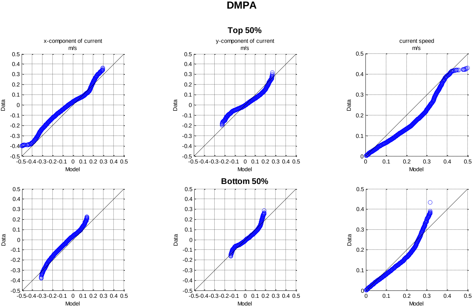
Figure E-1 Current Q-Q Plot – DMPA
