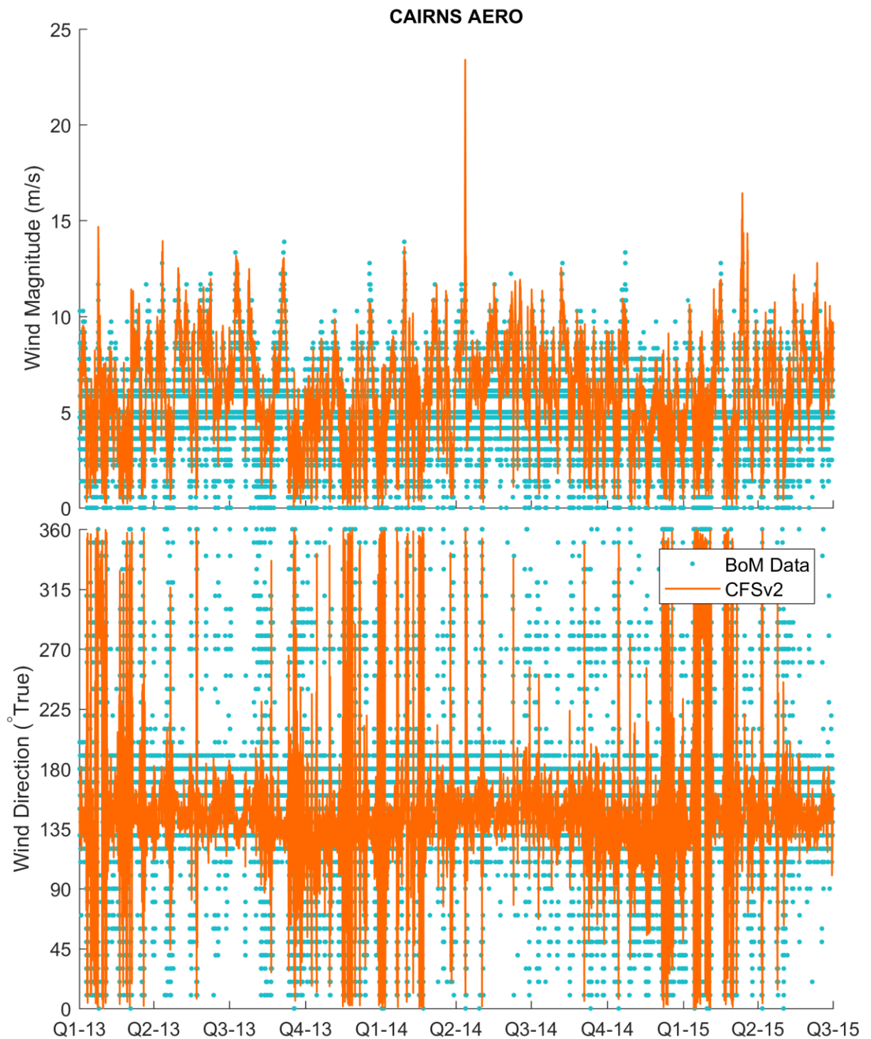
Figure 2-4 Cairns Aero Wind Calibration
