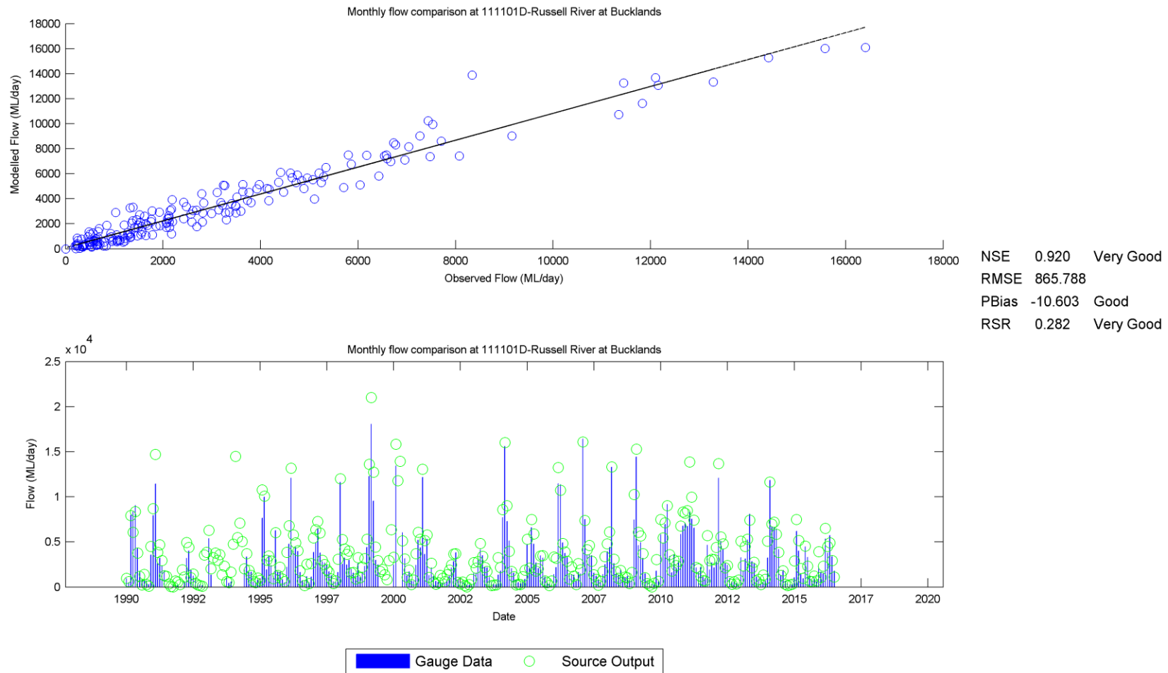
Figure 5-29 Catchment Model Comparison to Russel River Gauge
