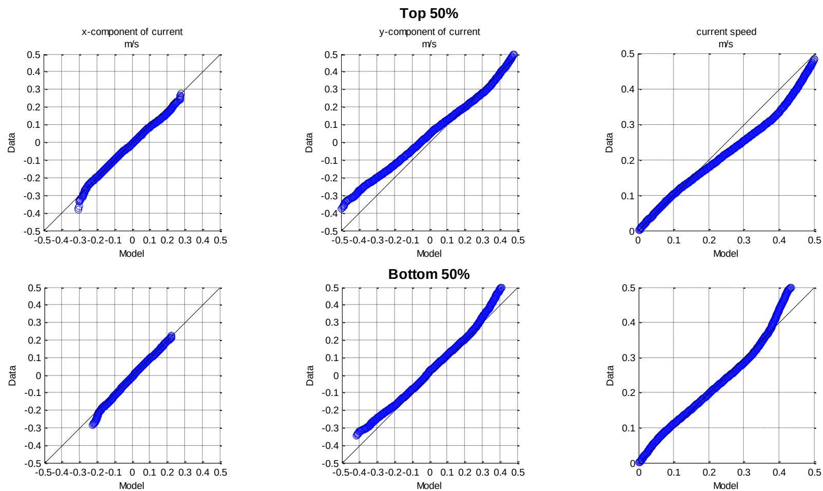
Figure E-4 Current Q-Q Plot – Beacon C11
