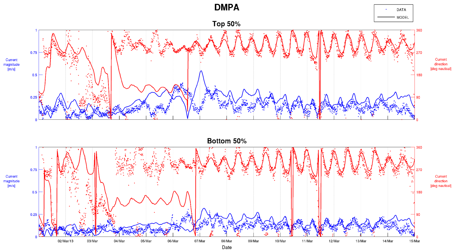
Figure C-1 Top 50% and Bottom 50% Current Calibration – DMPA 01/03/2013 to 15/03/2013
