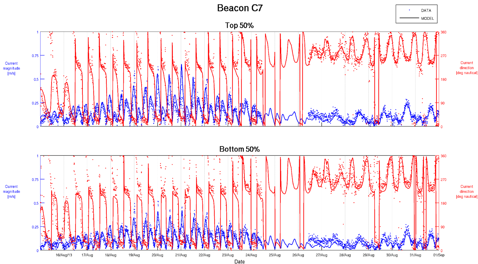
Figure F-12 Top 50% and Bottom 50% Current Validation – Beacon C7 15/08/2013 to 01/09/2013
