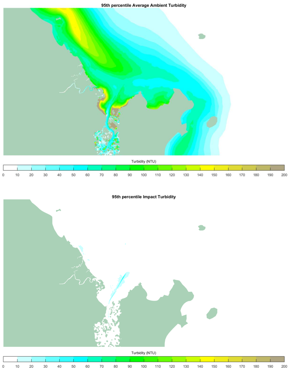
Figure 6-18 Maintenance 95 th Percentiles Turbidity: Average Ambient (Top), Impact of Dredging (bottom)
