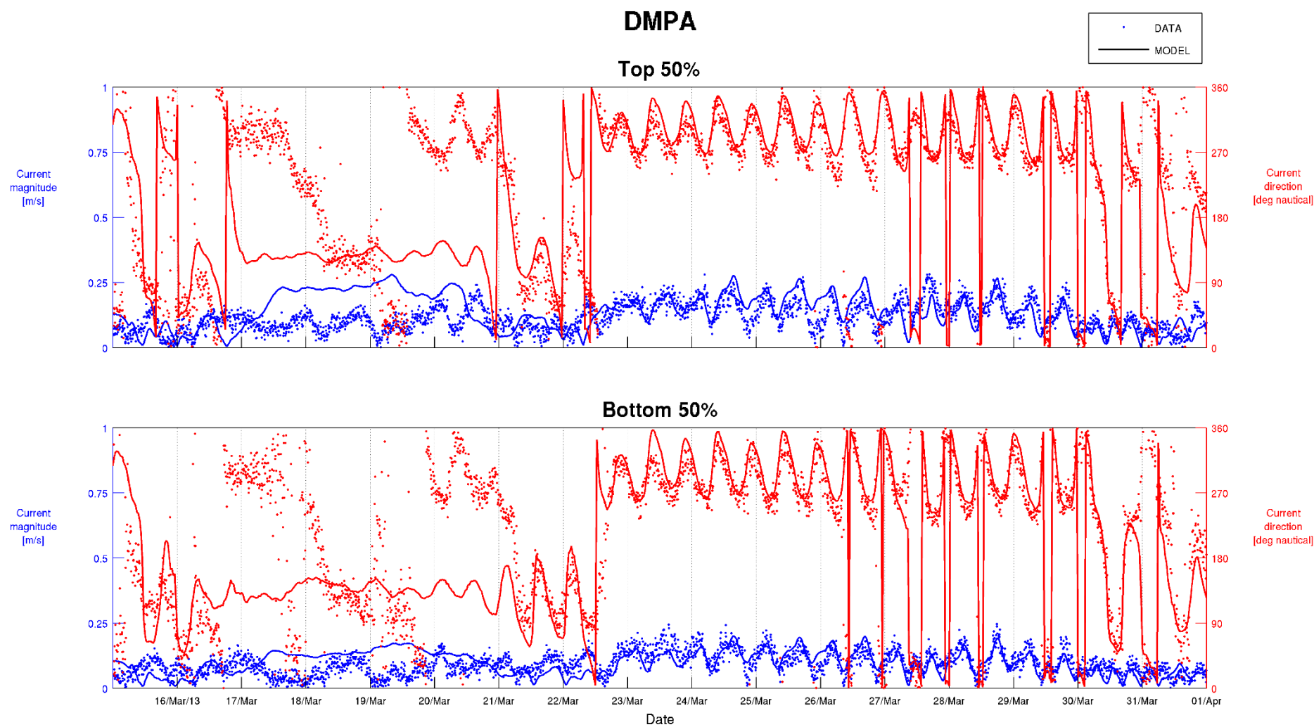
Figure C-2 Top 50% and Bottom 50% Current Calibration – DMPA 15/03/2013 to 01/04/2013
