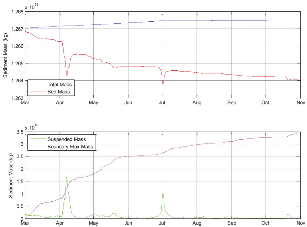
Figure 1. Sediment Mass Balance Checks - Capital Base Case
