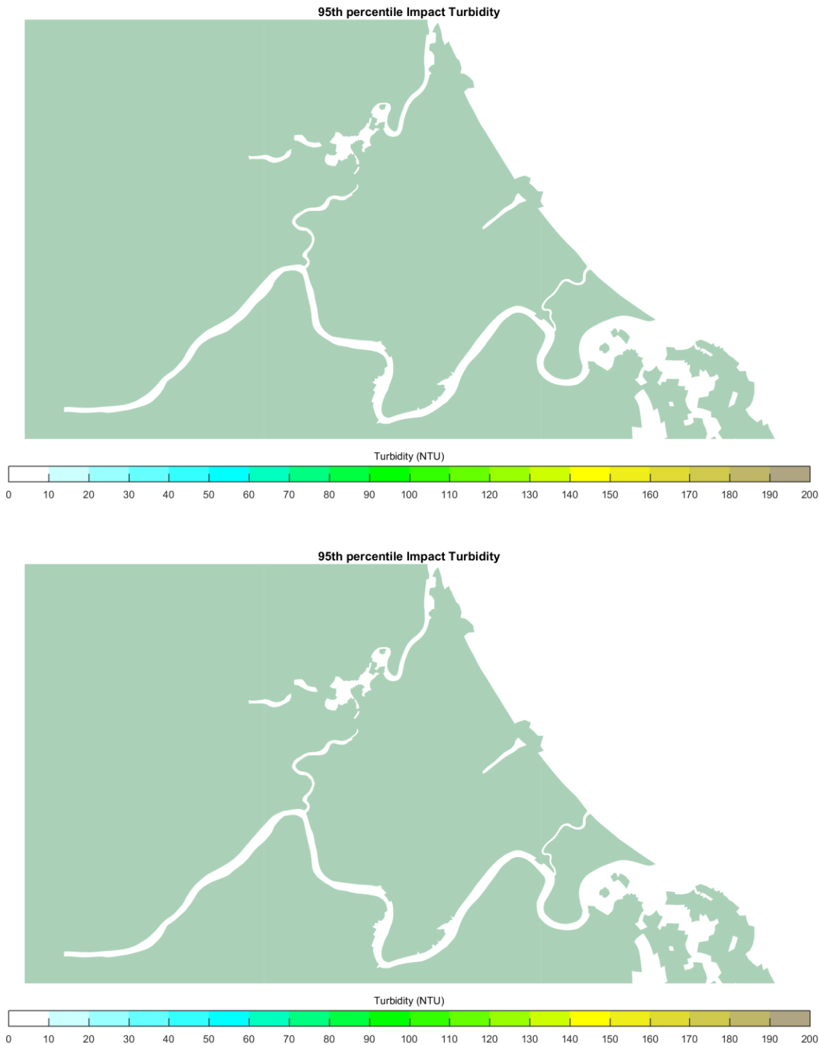
Figure 6-14 Impact to 95 th Percentile Turbidity: Site 1 (Top), Site 2 (Bottom)
