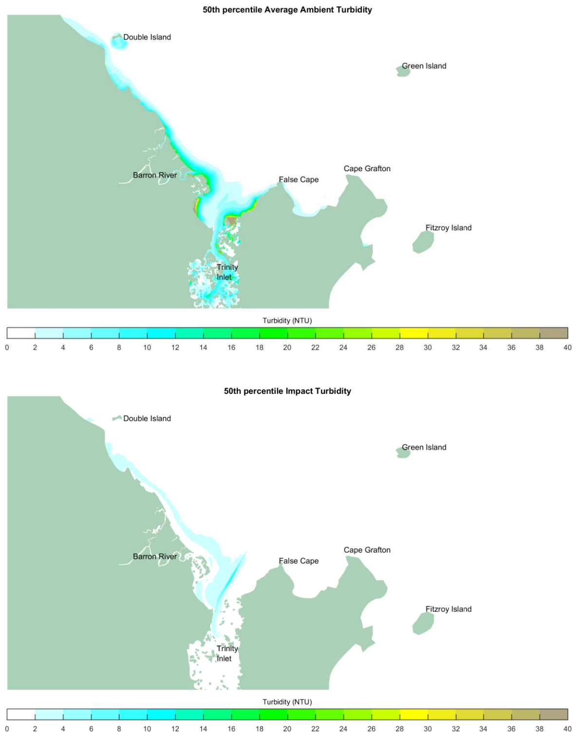
Figure 6-6 Likely Best Case Capital Program 50 th Percentiles Turbidity; Average Ambient Turbidity (Top), Impact of Dredging (Bottom)
