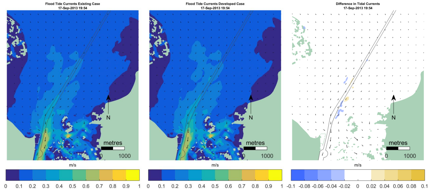
Figure 7-4 Modelled Spring Tide Flood Currents and Impacts – zoomed. Existing case (left); Developed case (middle) and Impacts (right)
