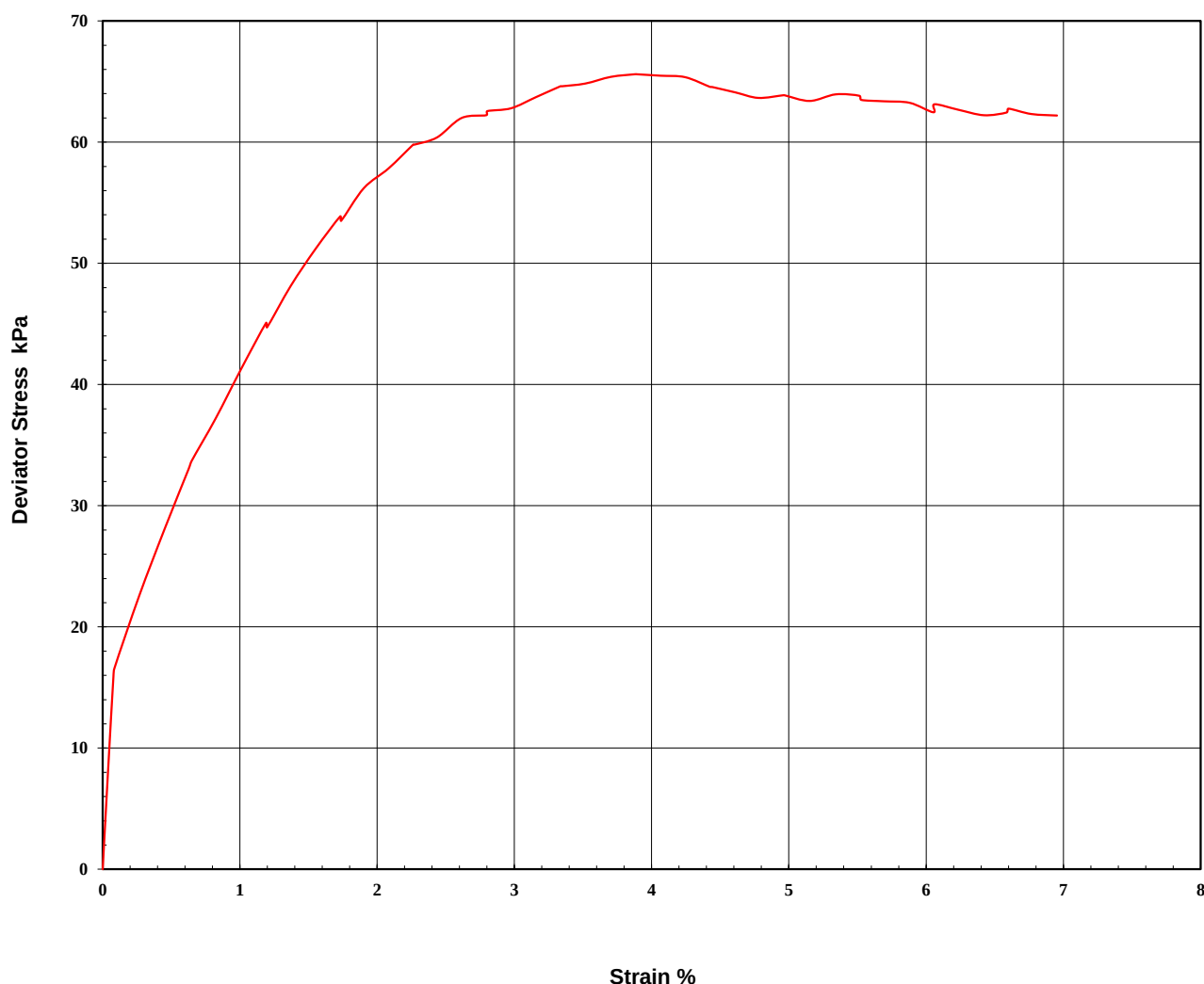
Stress/Strain Diagram
