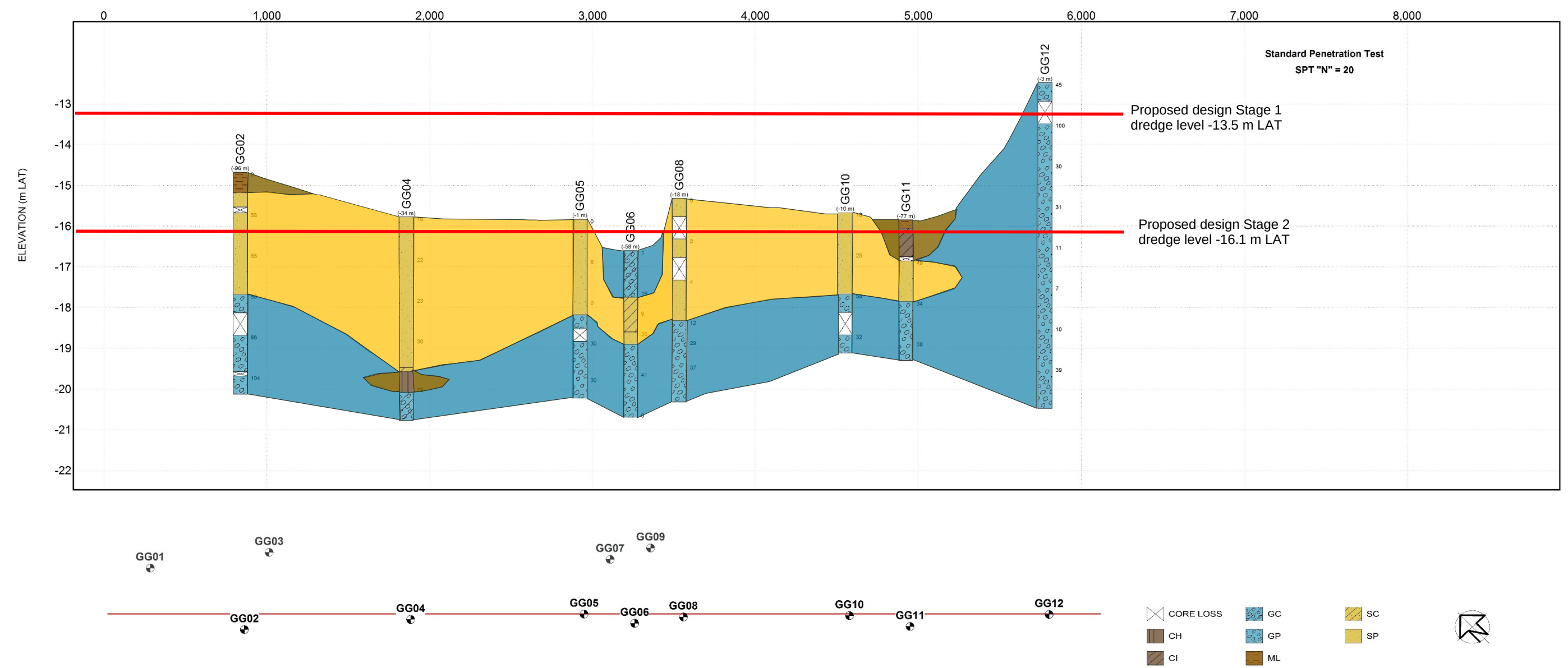
Figure 26 Sketch of the interpreted geological section for Gatcombe Channel (south) (NTS)
