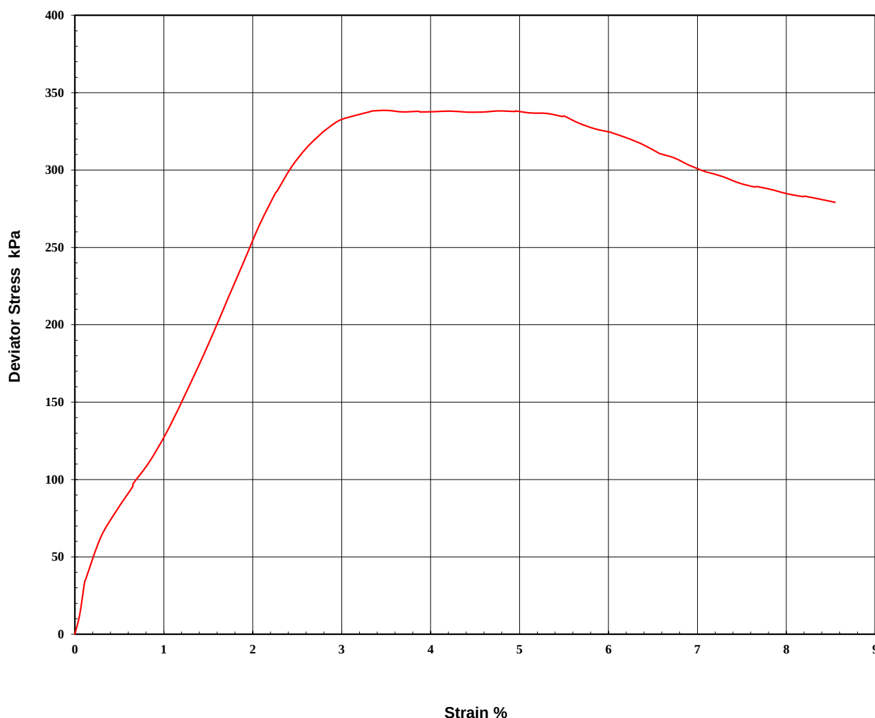
Stress/Strain Diagram
