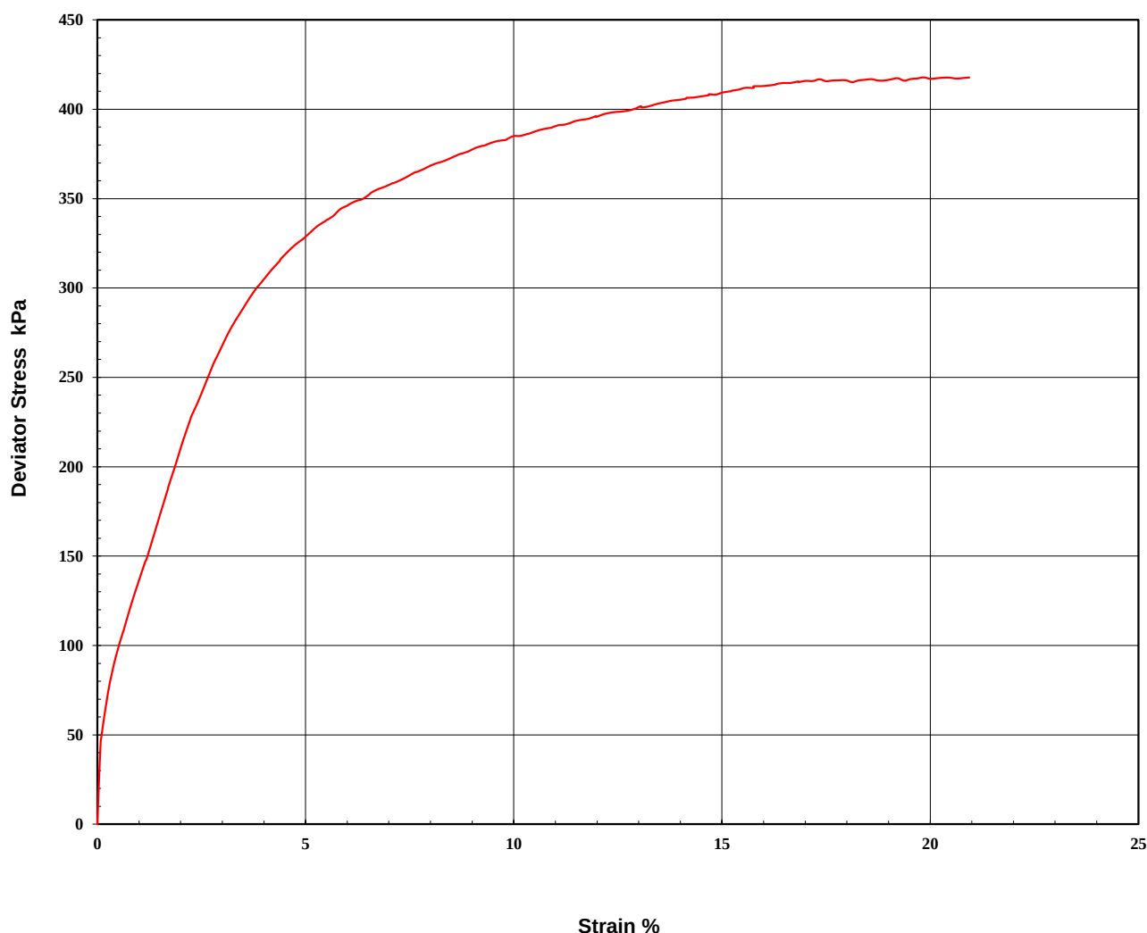
Stress/Strain Diagram
