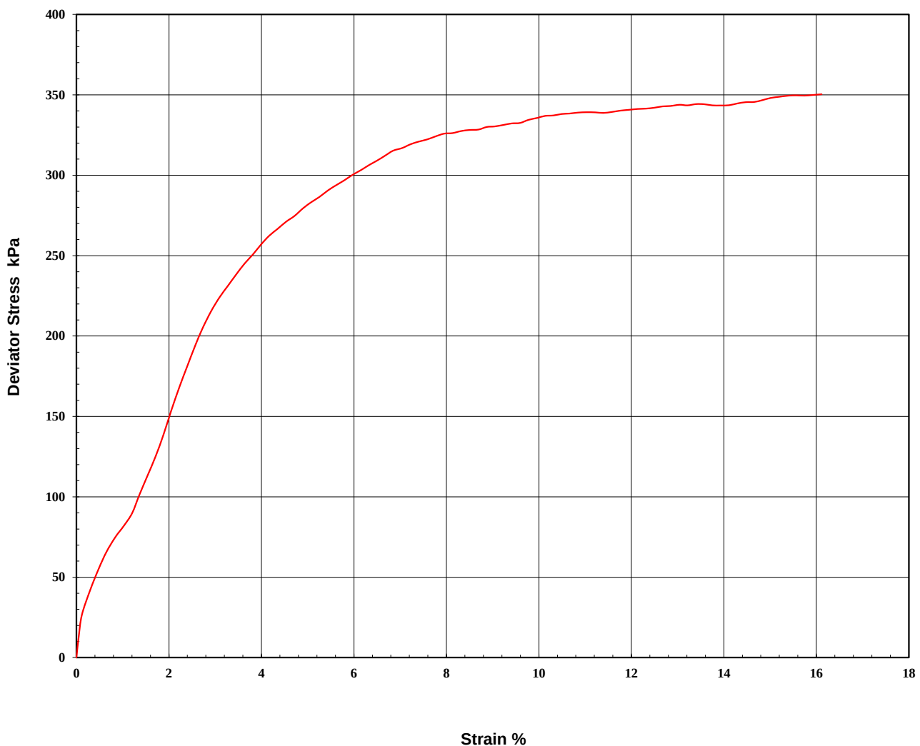
Stress/Strain Diagram
