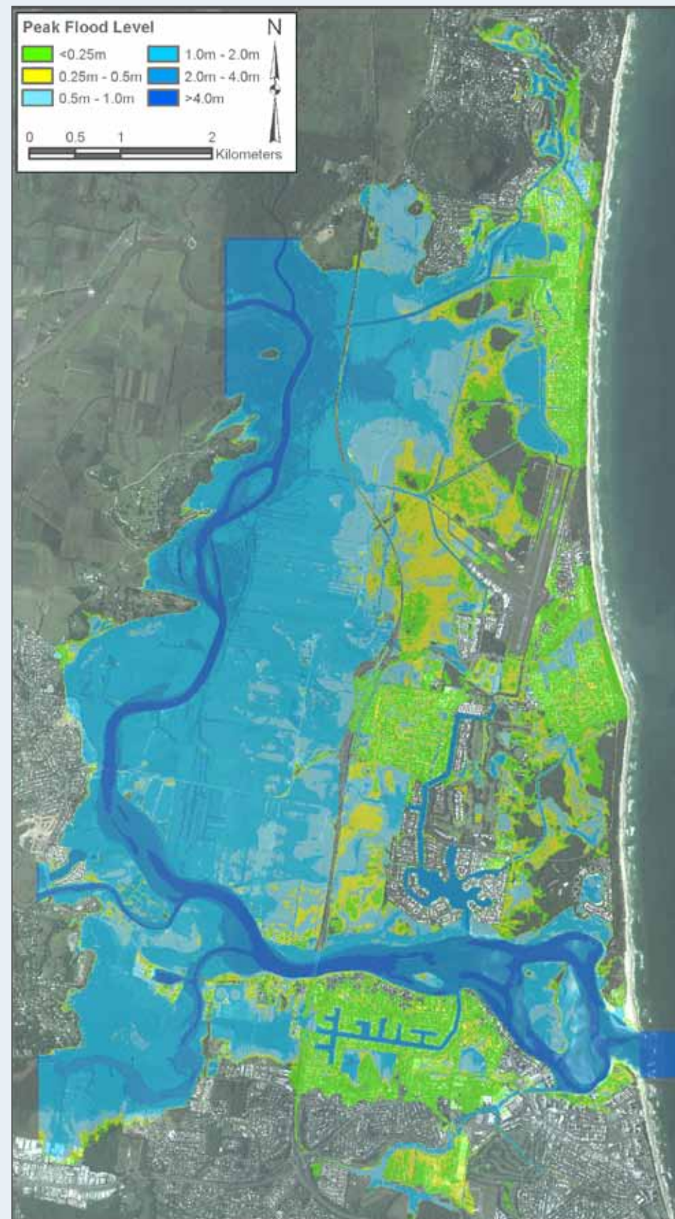
Figure 5.5m: Existing peak flood depth and extent, 50-year ARI
