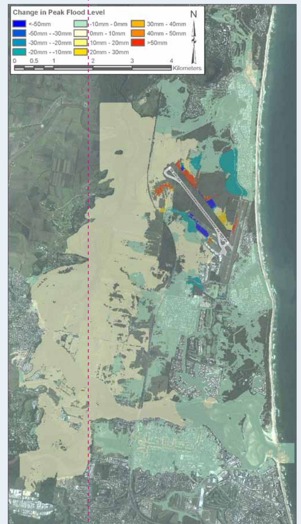
Figure 5.5c: Change in peak flood depth and extent, 2-year ARI
