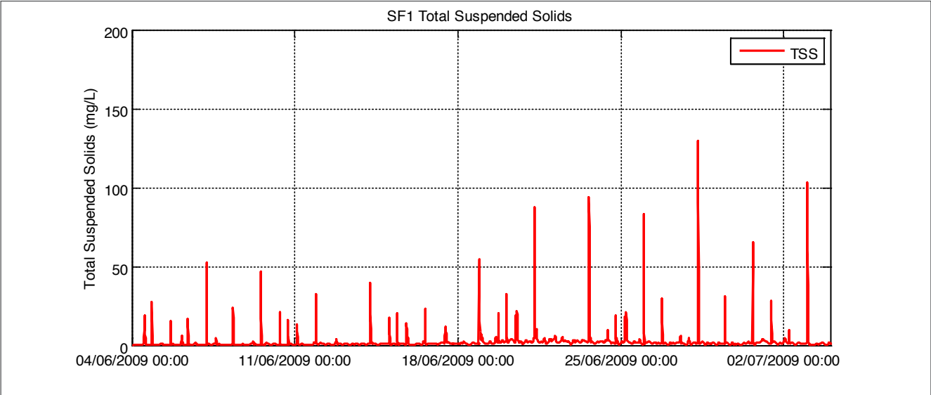
Figure C24: Winter period increase to total suspended solids – location SF1
