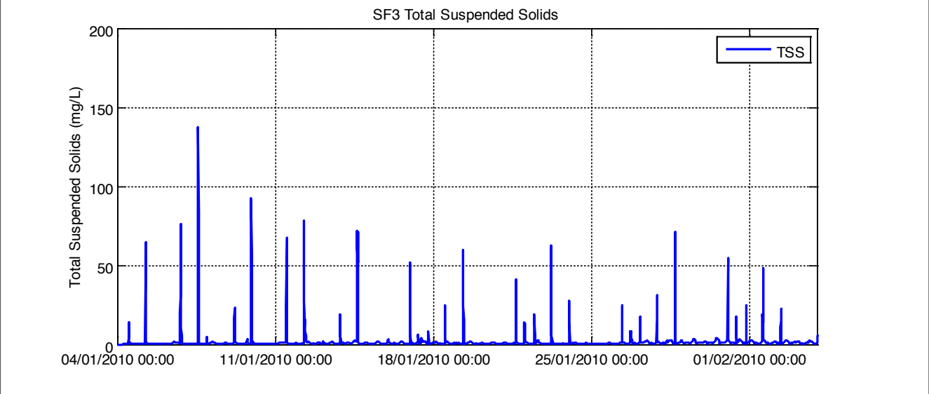
Figure C27: Summer period increase to total suspended solids – location SF3
