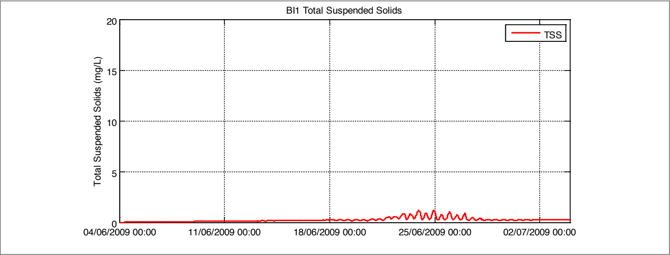
Figure C2: Winter period increase to total suspended solids – location BI1
