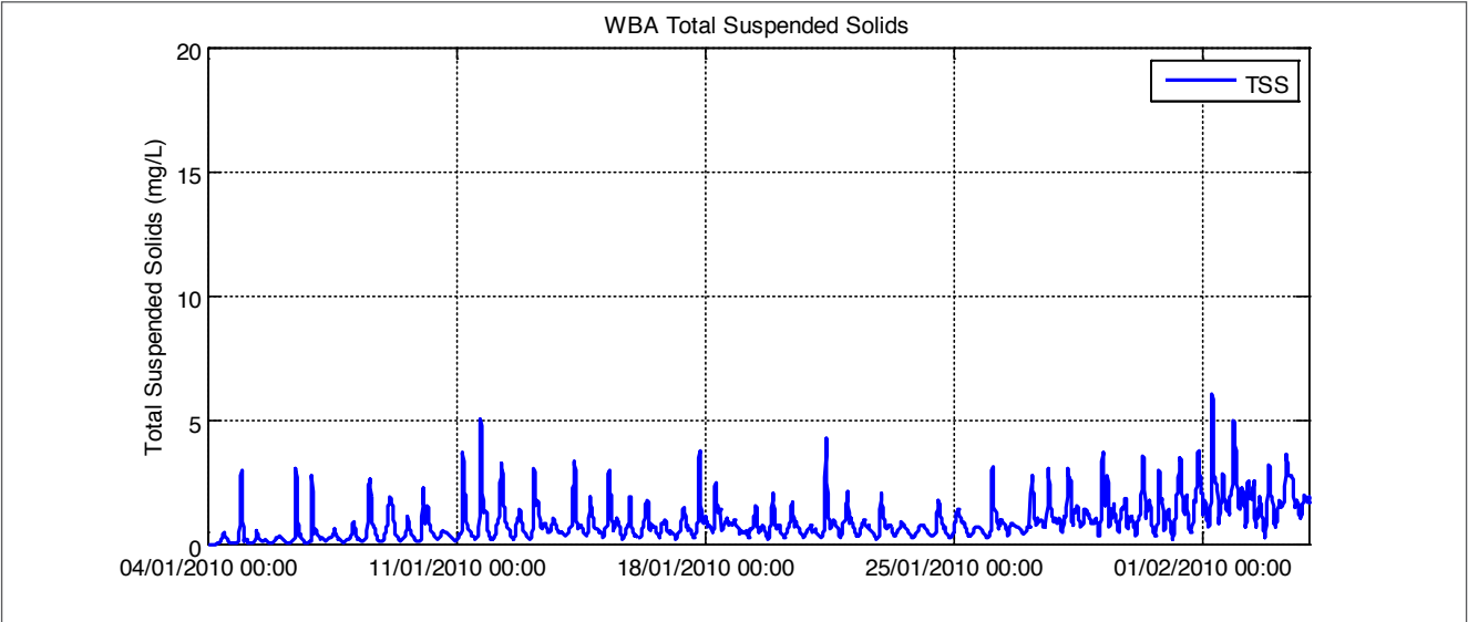
Figure C21: Summer period increase to total suspended solids – location WBA
