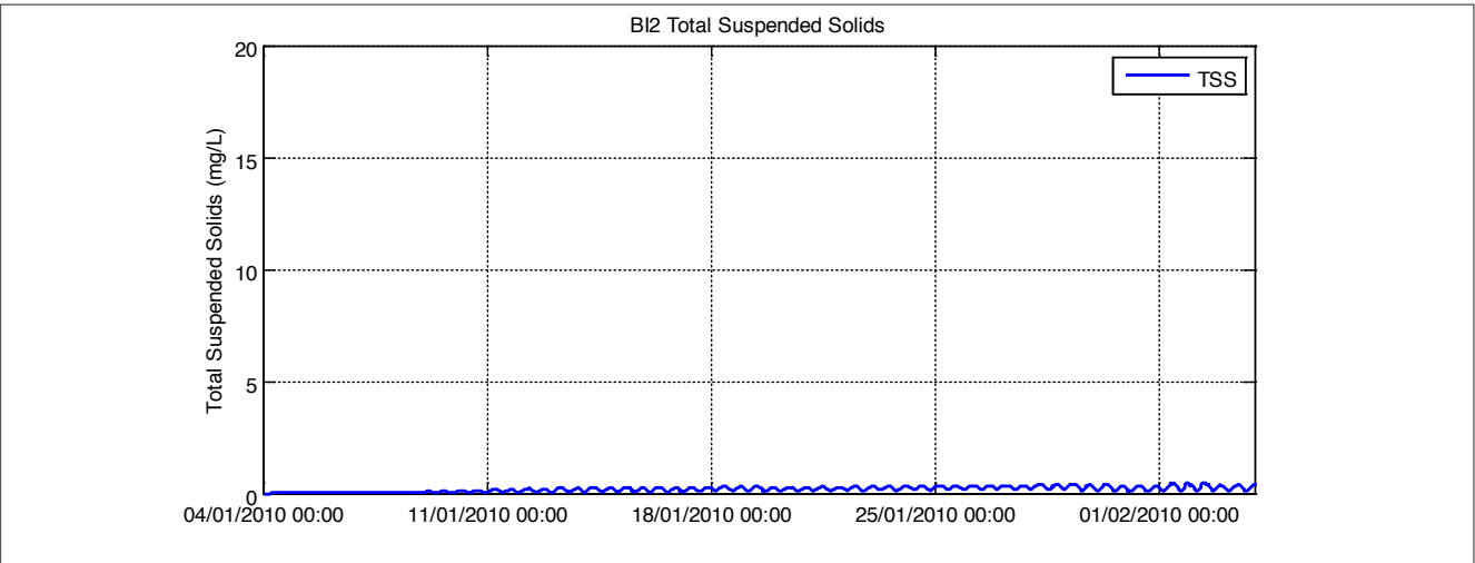
Figure C3: Summer period increase to total suspended solids – location BI2
