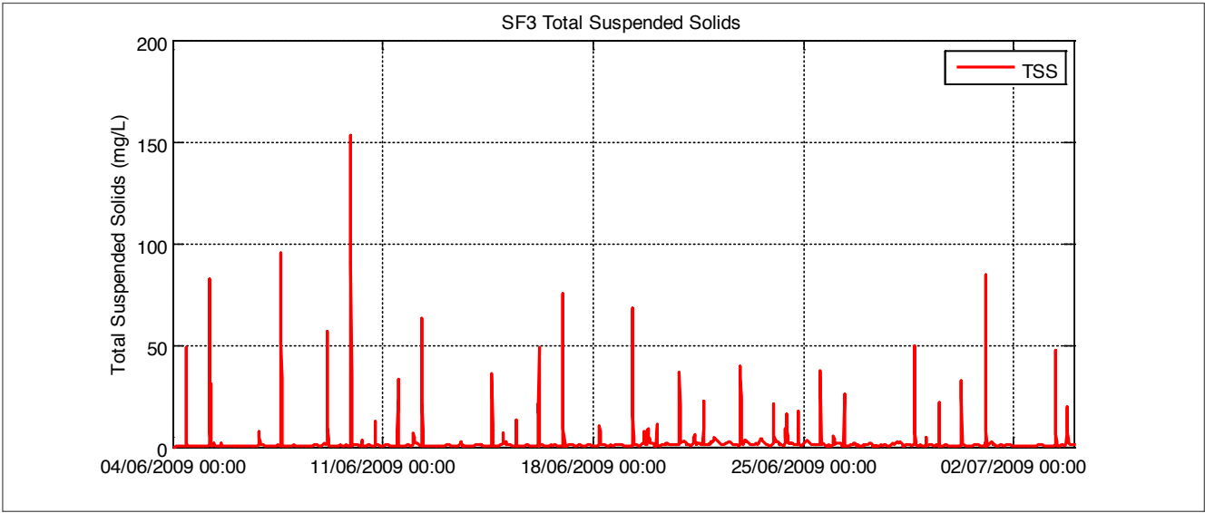
Figure C28: Winter period increase to total suspended solids – location SF3
