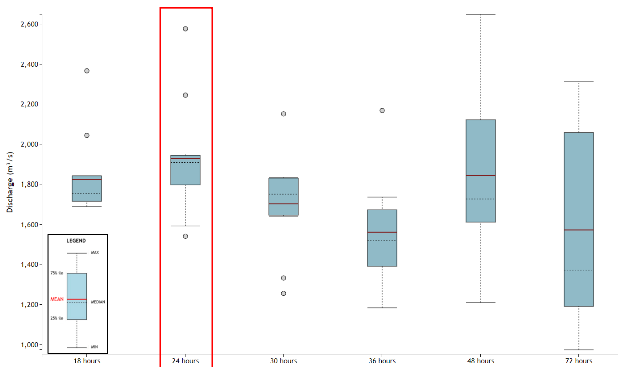
Figure E.4 - Box plots of 10% AEP design discharges at Deverill, Isaac River XP Rafts model
