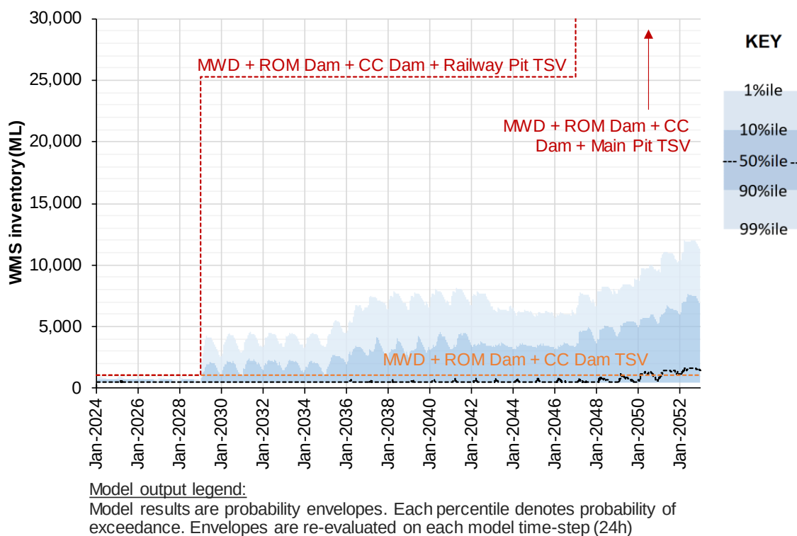
Figure 7.1 - Forecast water management system inventory
