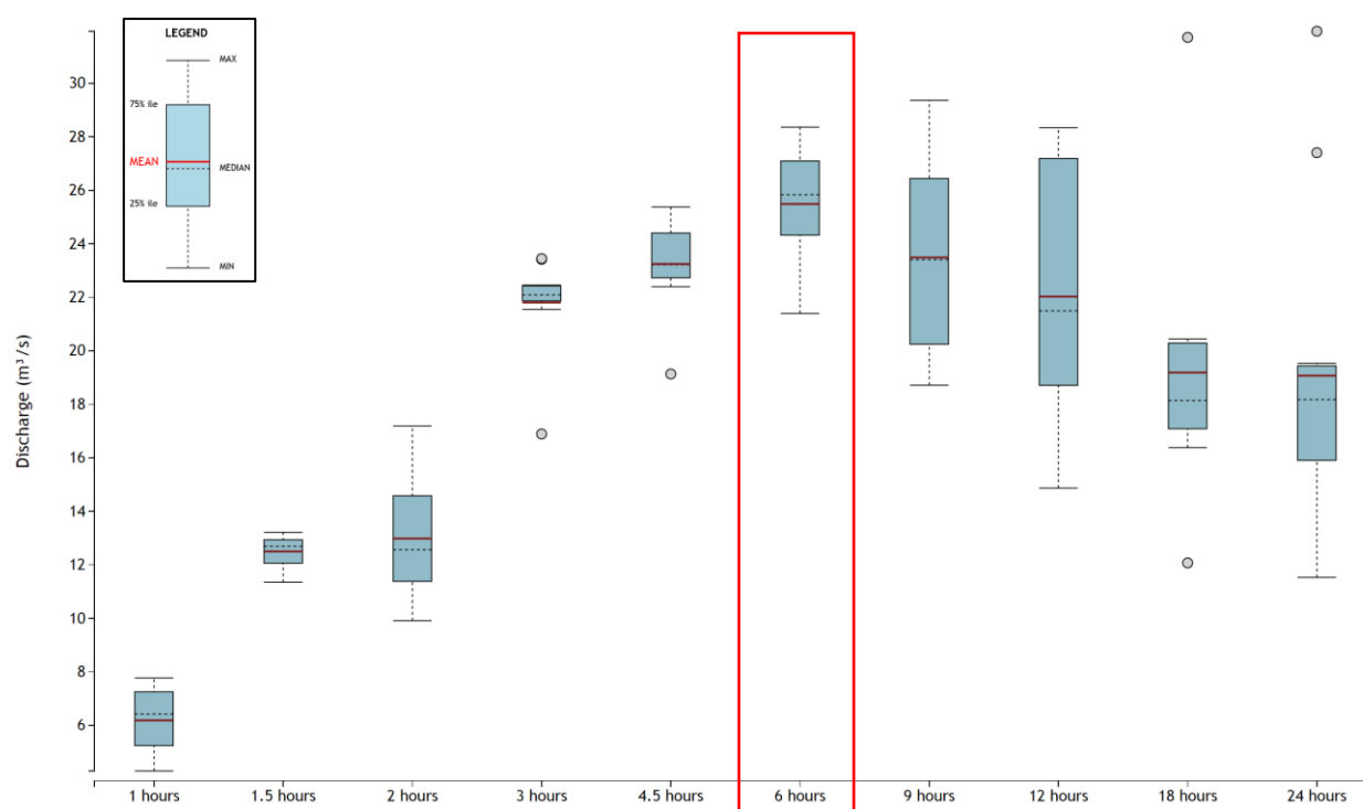
Figure E.1 - Box plots of 10% AEP design discharges at catchment 3, local drainage XPRafts model
