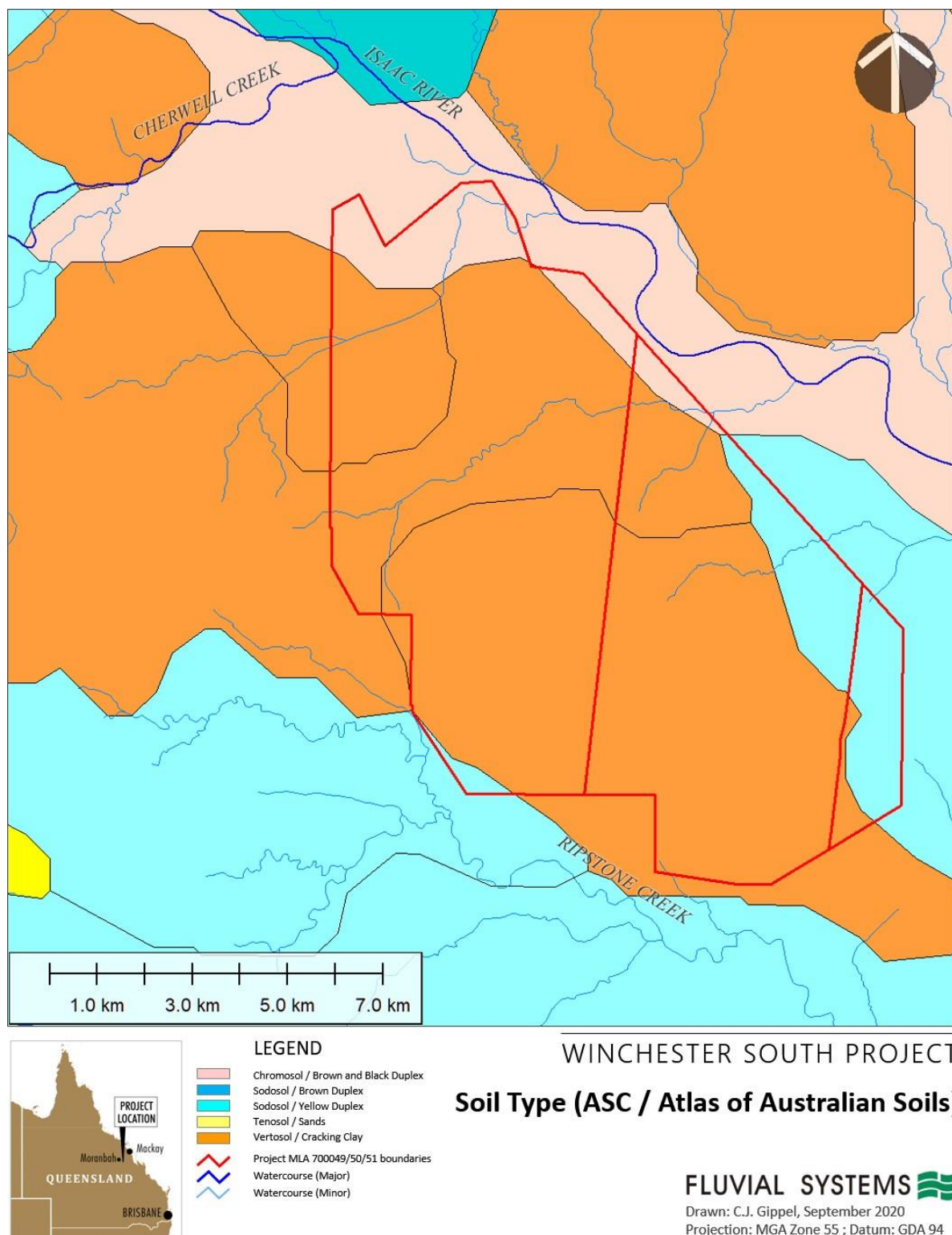
Figure 12. Soil Types in the Study Area.
