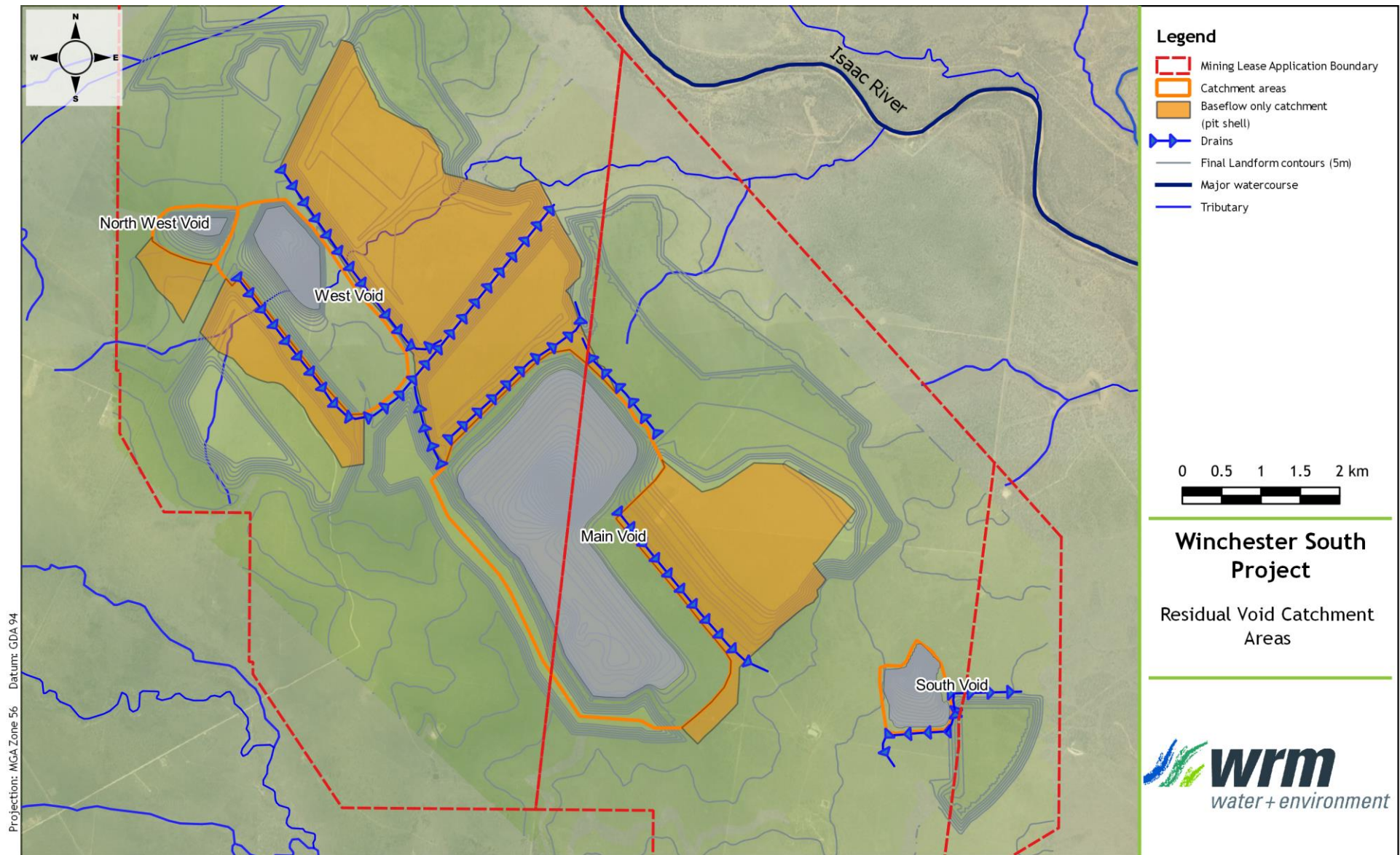
Figure 8.1 - Residual void catchment plan
