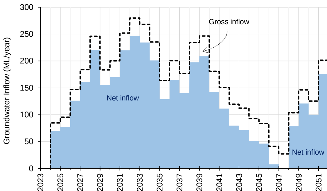
Figure 6.4 - Estimated annual groundwater inflows (data source: SLR, 2022)
