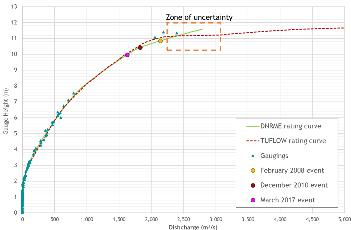
Figure C.2 - Comparison of DoR and modelled rating curves, Isaac River at Deverill
